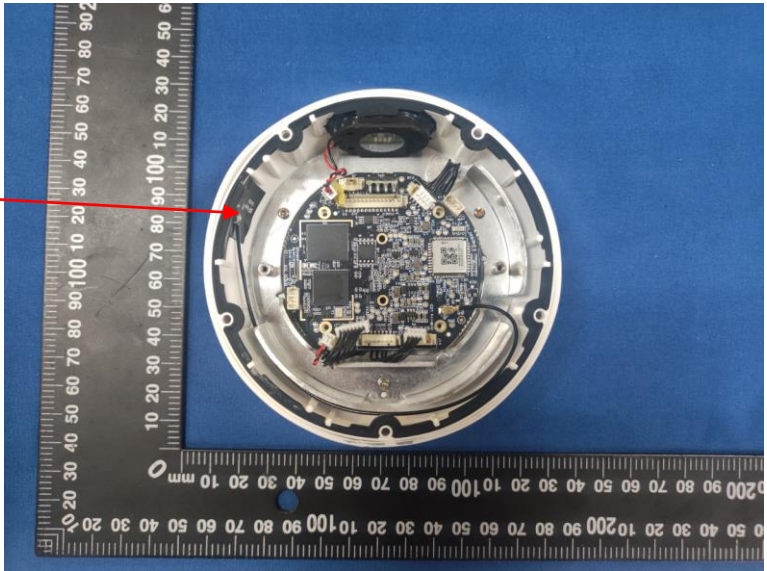
WIFI Antenna
