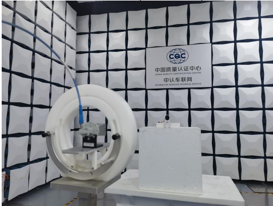
Radiated Emission (Above 42 GHz)
