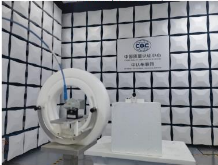
Radiated Emission (Above 42 GHz)
