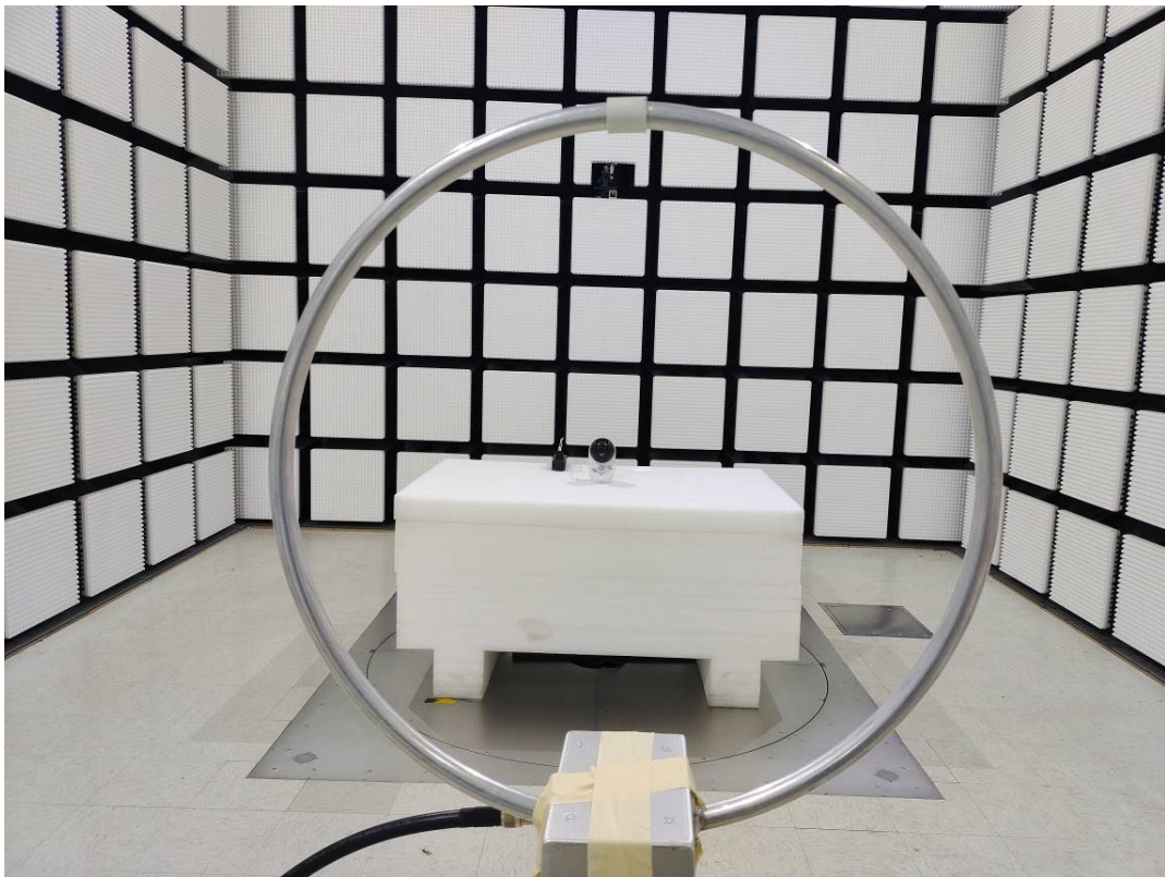
Radiated Emission 9k-30MHz Parallel View -P210
