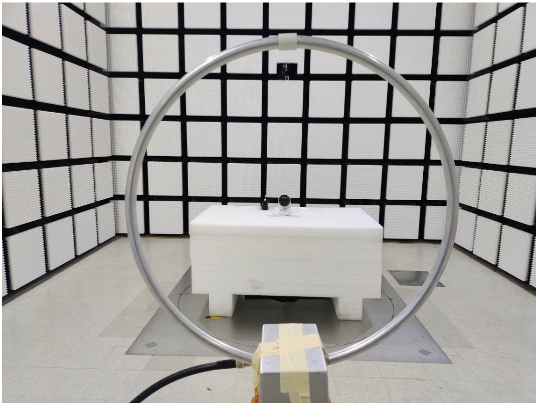
Radiated Emission 9K-30MHz Parallel View - P220
