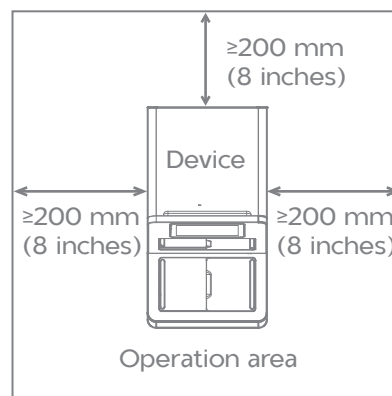
Figure 8 Space requirements
