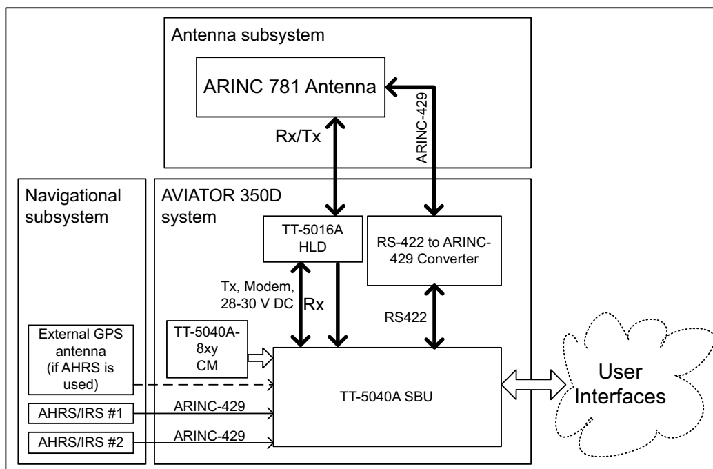
Figure 2-7: System configuration ARINC 429 antennas
