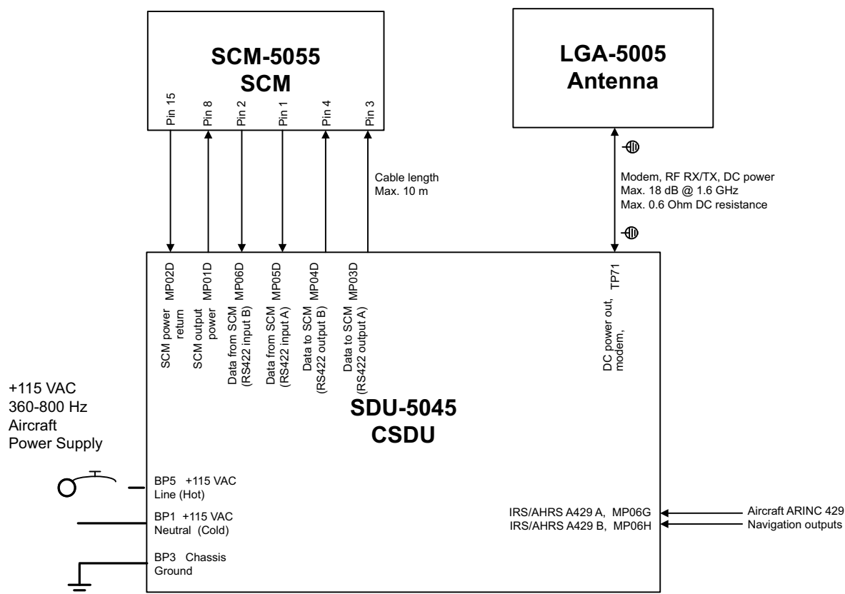
Figure 4-1: AVIATOR 200S system (minimum, AC powered)
