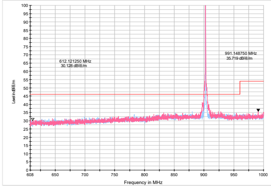
US915, 915MHz, 608 MHz to 1000MHz
