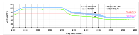
802.11n HT20 -Channel 11 Peak+ Average
