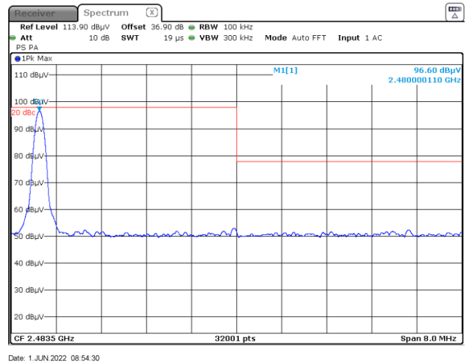
Figure 7.7-18: Non-restricted band edge at 2483.5 MHz, high channel
