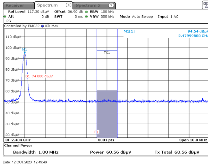
Figure 7.7-10: Band edge spurious emissions at 2483.5 MHz Peak – Hopping OFF
