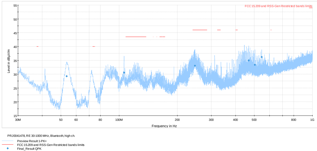
Figure 7.7-3: Radiated spurious emissions 30-1000 MHz high channel
