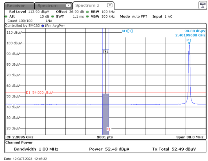
Figure 7.7-9: Band edge spurious emissions at 2390 MHz Average – Hopping OFF
