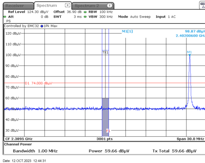
Figure 7.7-8: Band edge spurious emissions at 2390 MHz Peak – Hopping OFF
