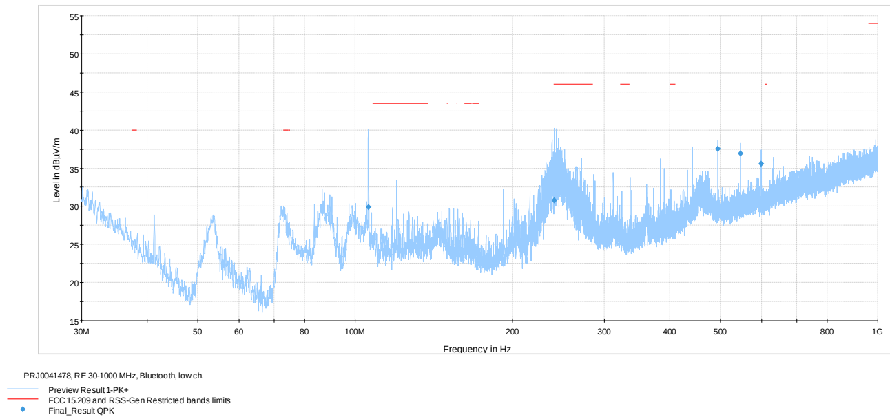
Figure 7.7-1: Radiated spurious emissions 30-1000 MHz low channel
