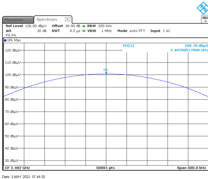
Figure 7.6-1: Output power on low channel
