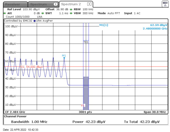
Figure 7.7-15: Band edge spurious emissions at 2483.5 MHz Average – Hopping ON
