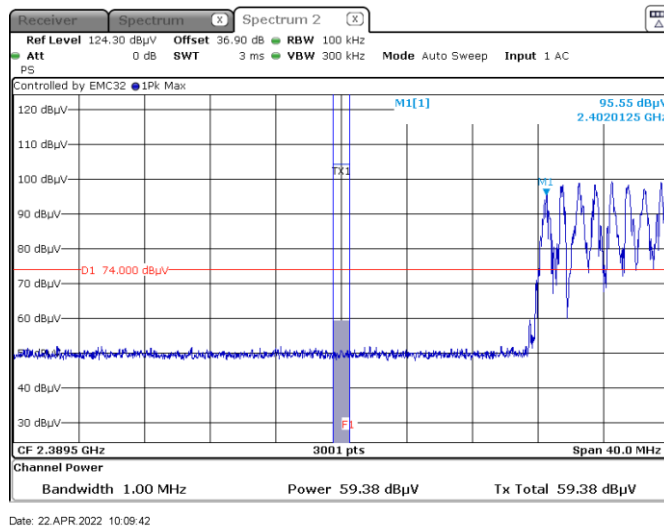
Figure 7.7-12: Band edge spurious emissions at 2390 MHz Peak – Hopping ON
