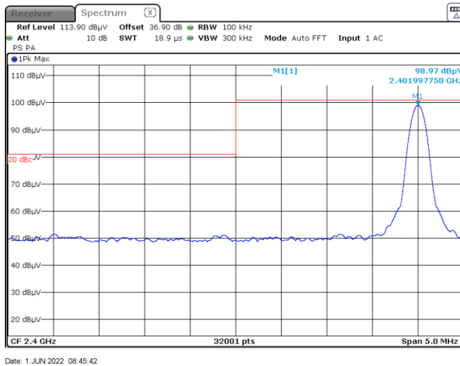
Figure 7.7-16: Non-restricted band edge at 2400 MHz, low channel
