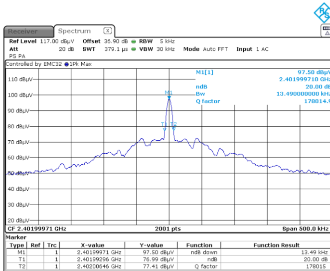
Figure 7.5-1: 20 dB bandwidth on low channel
