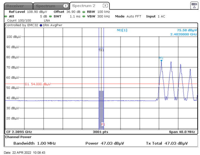
Figure 7.7-13: Band edge spurious emissions at 2390 MHz Average – Hopping ON
