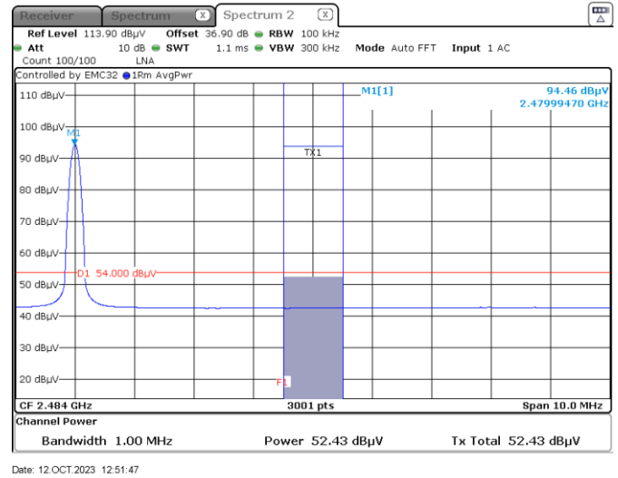
Figure 7.7-11: Band edge spurious emissions at 2483.5 MHz Average – Hopping OFF
