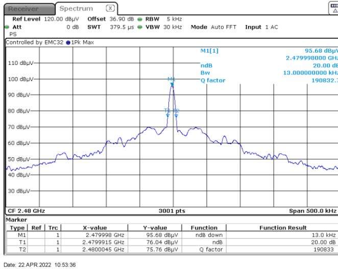
Figure 7.5-3: 20 dB bandwidth on high channel
