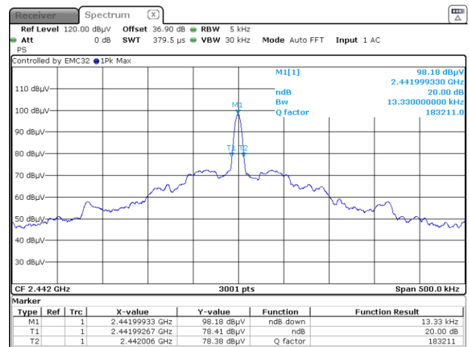
Figure 7.5-2: 20 dB bandwidth on mid channel
