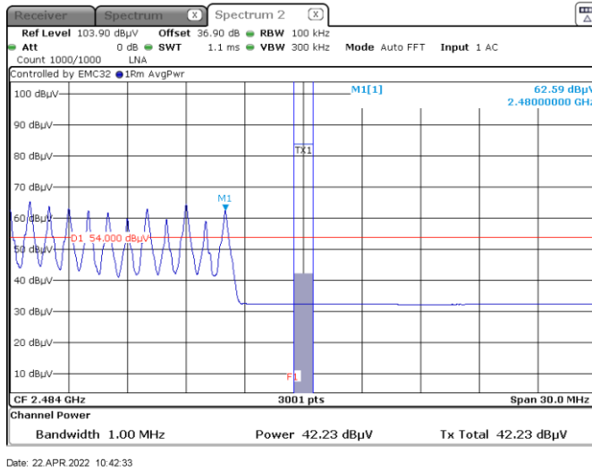
Figure 7.7-14: Band edge spurious emissions at 2483.5 MHz Peak – Hopping ON
