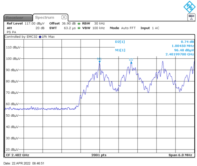
Figure 7.5-4: Carrier frequency separation
