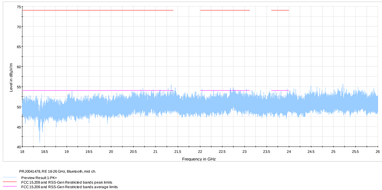
Figure 7.7-7: Sample plot, Radiated spurious emissions 18-26 GHz mid channel
