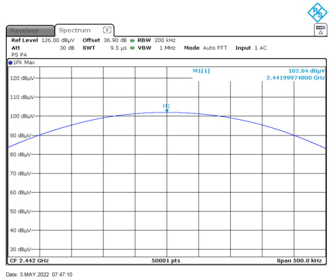
Figure 7.6-2: Output power on mid channel
