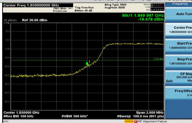
Band2-5MHz-16QAM-18625-25RB#0
