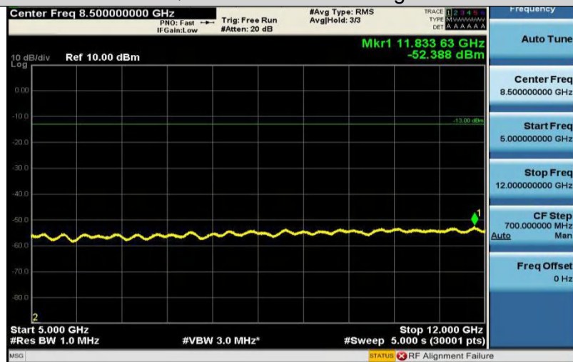
Band2-20MHz-16QAM-18900-1RB#0-Range3:5000~12000MHz
