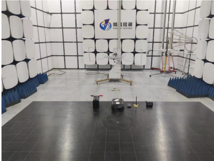
Radiated emission
