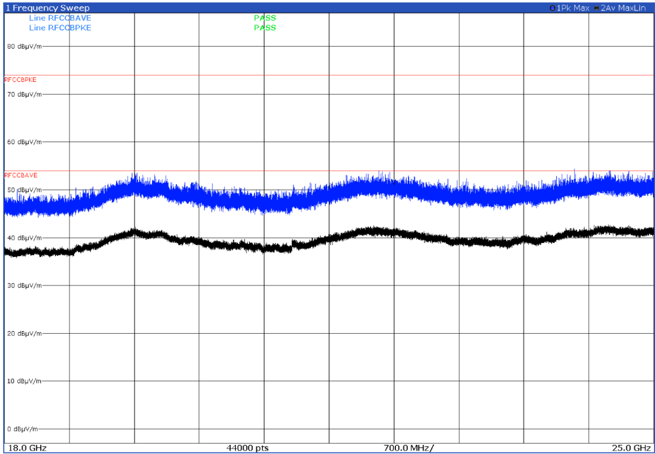
Figure 8.1-24: Radiated spurious emissions with LTE B12 at mid channel and WIFI at mid channel – antenna in horizontal polarization
