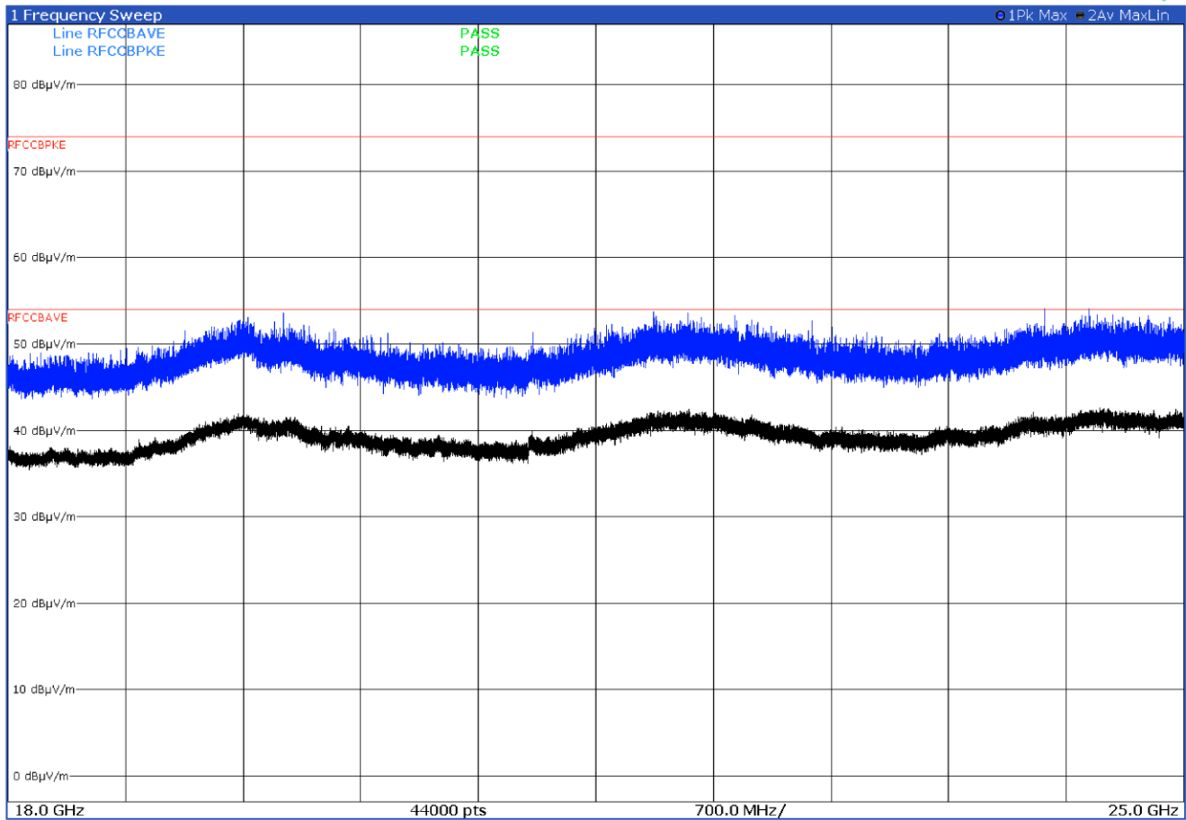
Figure 8.1-7: Radiated spurious emissions with LTE B2 at mid channel and BLE at mid channel – antenna in horizontal polarization
