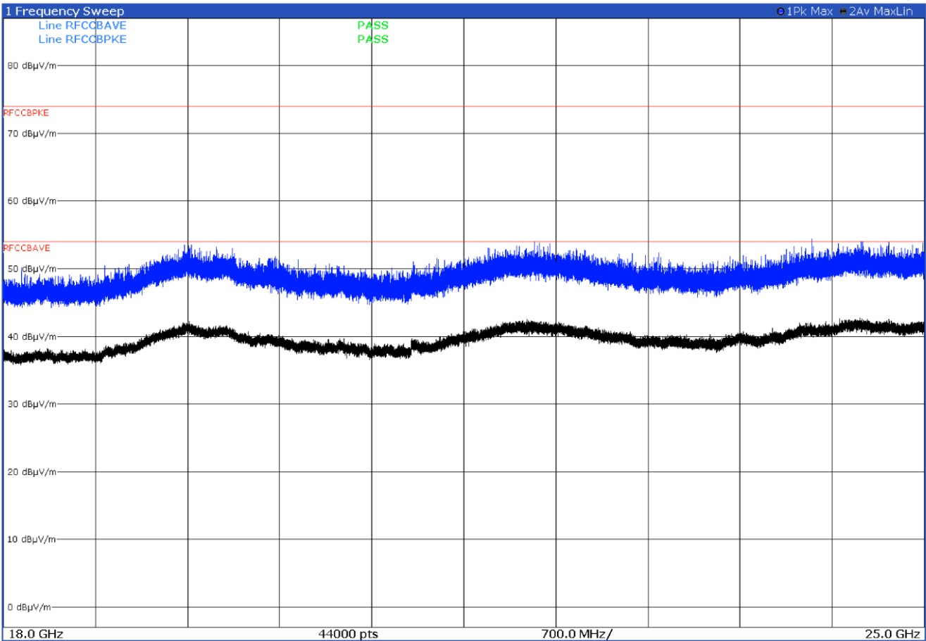
Figure 8.1-15: Radiated spurious emissions with LTE B4 at mid channel and WIFI at mid channel – antenna in horizontal polarization
