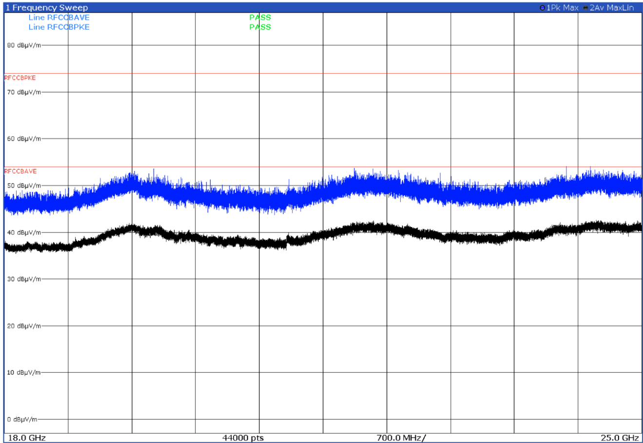
Figure 8.1-16: Radiated spurious emissions with LTE B4 at mid channel and WIFI at mid channel – antenna in vertical polarization
