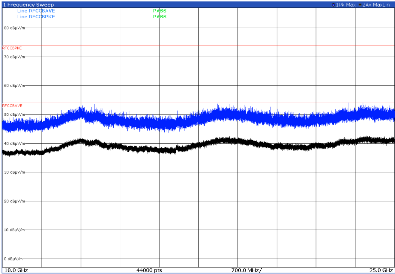
Figure 8.1-46: Radiated spurious emissions with WCDMA B5 at mid channel and WIFI at mid channel – antenna in vertical polarization
