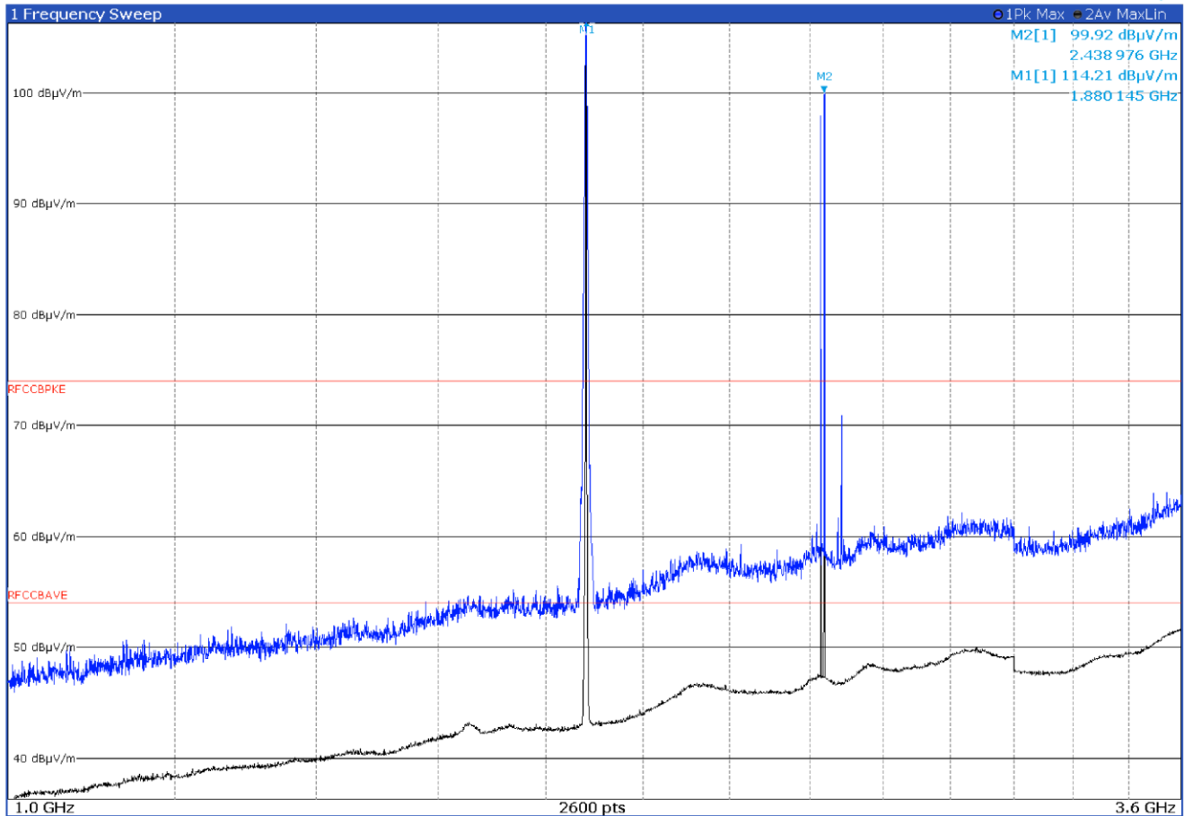
Figure 8.1-4: Radiated spurious emissions with LTE B2 at mid channel and WIFI at mid channel – antenna in vertical polarization
