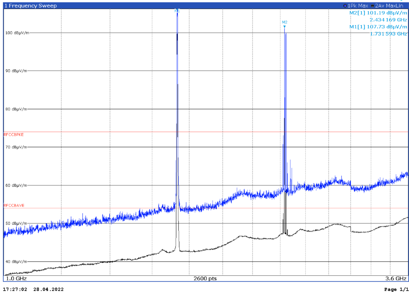
Figure 8.1-35: Radiated spurious emissions with WCDMA B4 at mid channel and WIFI at mid channel – antenna in vertical polarization
