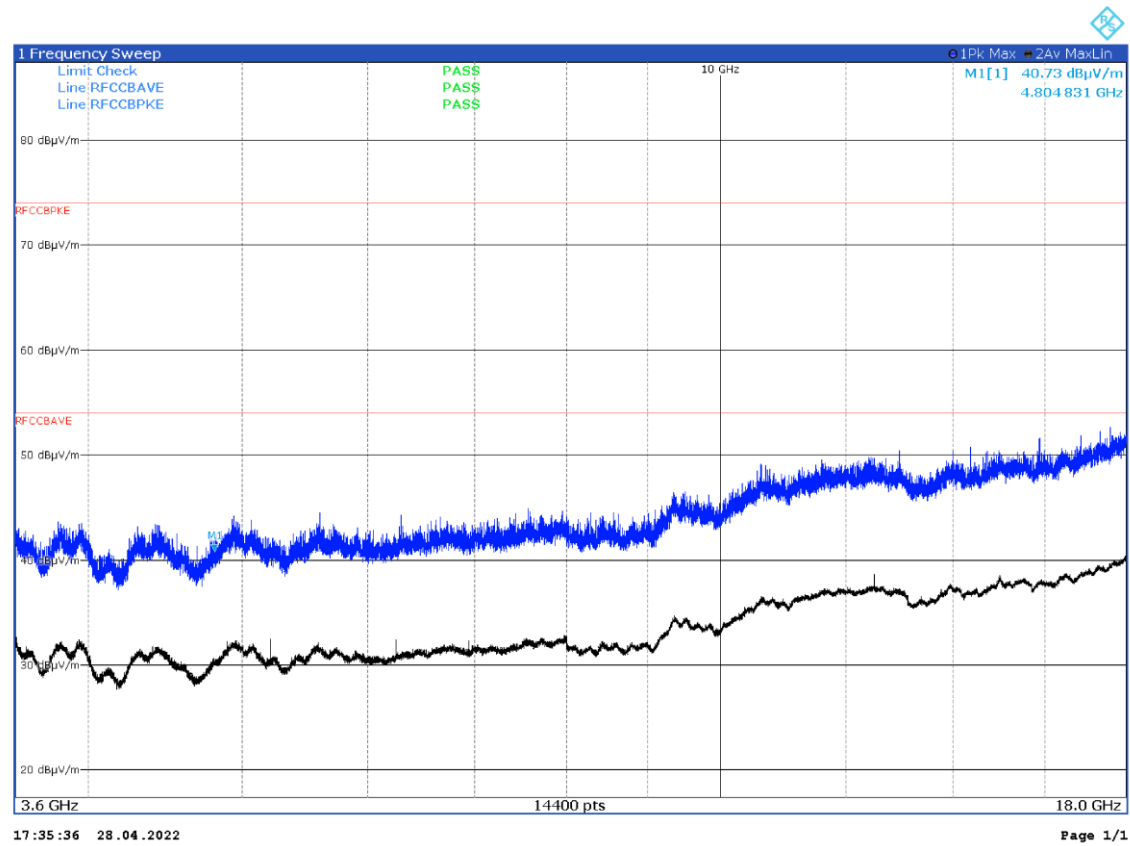
Figure 8.1-44: Radiated spurious emissions with WCDMA B5 at mid channel and WIFI at mid channel – antenna in vertical polarization
