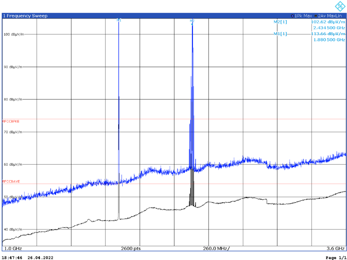
Figure 8.1-28: Radiated spurious emissions with WCDMA B2 at mid channel and WIFI at mid channel – antenna in horizontal polarization
