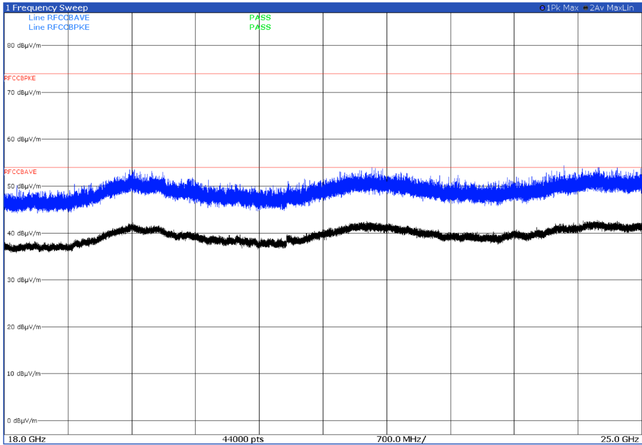
Figure 8.1-8: Radiated spurious emissions with LTE B2 at mid channel and BLE at mid channel – antenna in vertical polarization
