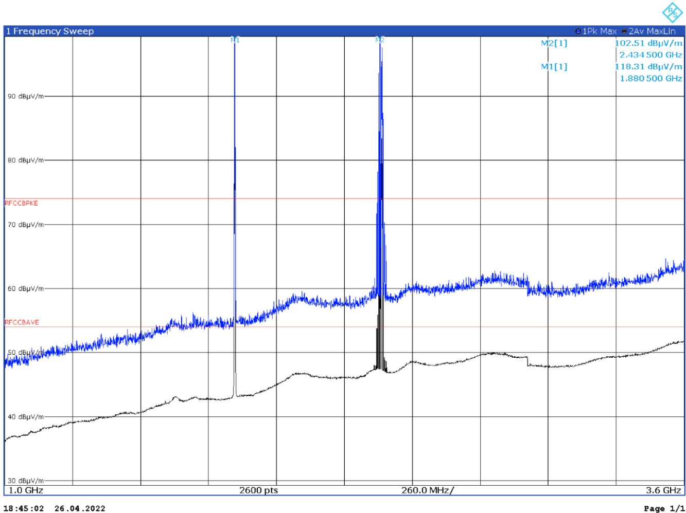
Figure 8.1-27: Radiated spurious emissions with WCDMA B2 at mid channel and WIFI at mid channel – antenna in vertical polarization
