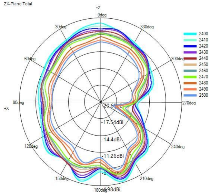
(1) X-Z Plane(unit:dBi):
