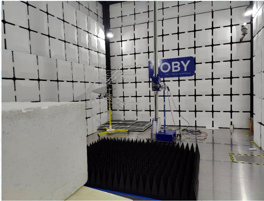
Photo of Setup for Radiated Emission (Above 1 GHz)
