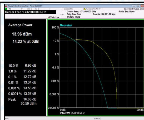
Band4-3MHz-16QAM-20175-6-0-Low-12.72-<=13-PASS
