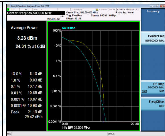
Band5-3MHz-16QAM-20525-6-0-Low-10.17-<=13-PASS
