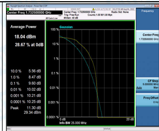
Band4-10MHz-16QAM-20175-6-0-Low-9.60-<=13-PASS
