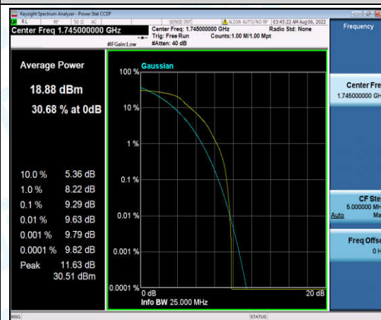
Band4-20MHz-QPSK-20300-6-0-High-9.29-<=13-PASS
