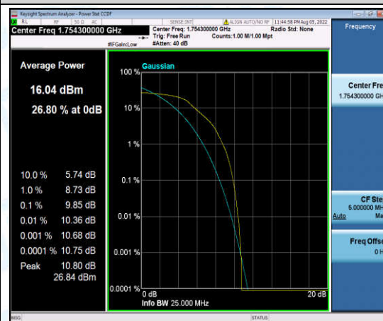
Band4-1.4MHz-QPSK-20393-6-0-High-9.85-<=13-PASS
