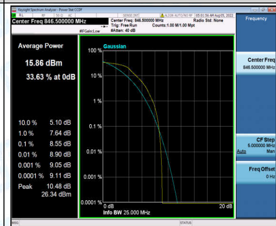
Band5-5MHz-QPSK-20625-6-0-High-8.55-<=13-PASS
