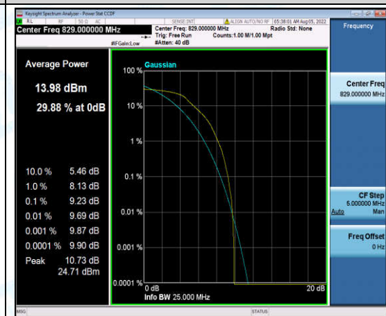
Band5-10MHz-QPSK-20450-6-0-Low-9.23-<=13-PASS
