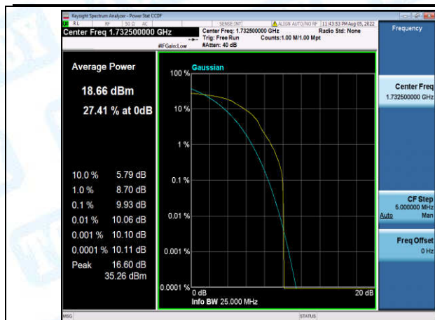
Band4-1.4MHz-16QAM-20175-1-0-Low-9.93-<=13-PASS
