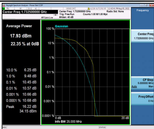
Band4-1.4MHz-QPSK-20175-1-0-Low-10.45-<=13-PASS
