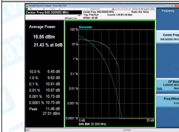
Band5-5MHz-16QAM-20625-1-0-High-10.61-<=13-PASS
