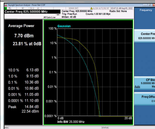
Band5-3MHz-16QAM-20415-6-0-Low-10.36-<=13-PASS
