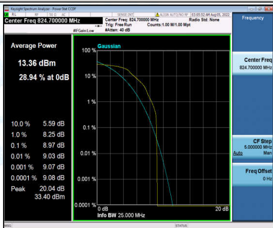
Band5-1.4MHz-QPSK-20407-1-0-Low-8.97-<=13-PASS
