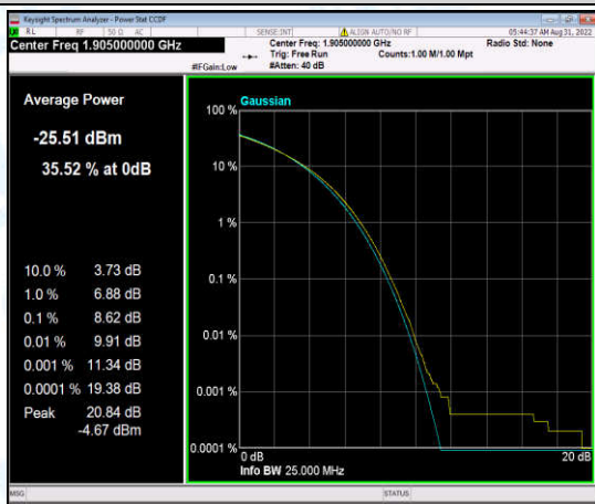
Band2-15MHz-16QAM-19150-1-0-High-8.62-<=13-PASS
