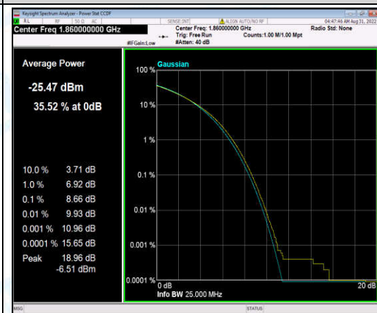
Band2-20MHz-16QAM-18700-6-0-Low-8.66-<=13-PASS
