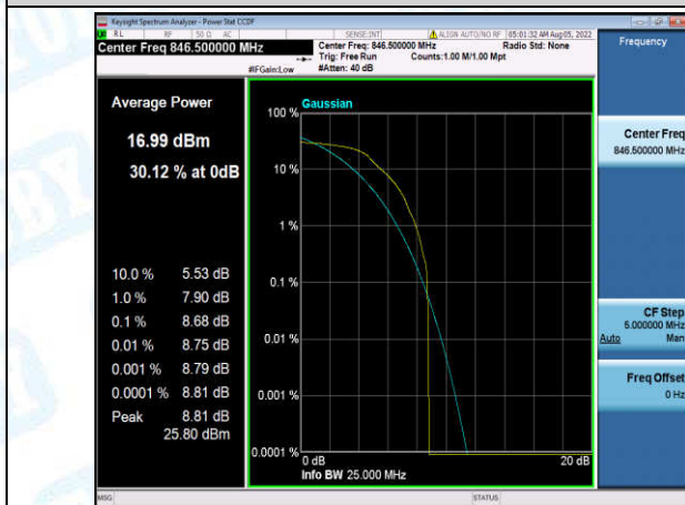
Band5-5MHz-QPSK-20625-1-0-High-8.68-<=13-PASS
