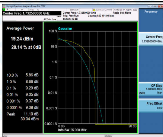
Band4-15MHz-16QAM-20175-1-0-Low-9.29-<=13-PASS
