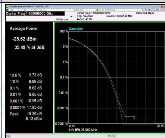
Band2-20MHz-QPSK-19100-6-0-High-8.62-<=13-PASS
