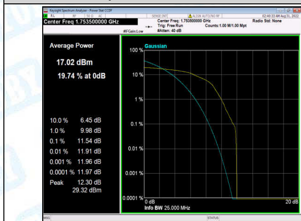
Band4-3MHz-16QAM-20385-1-0-High-11.54-<=13-PASS
