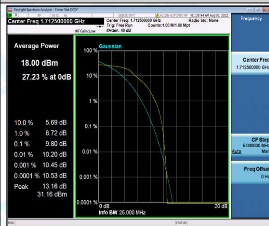
Band4-5MHz-16QAM-19975-6-0-Low-9.80-<=13-PASS
