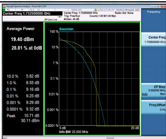
Band4-20MHz-16QAM-20175-1-0-Low-9.16-<=13-PASS
