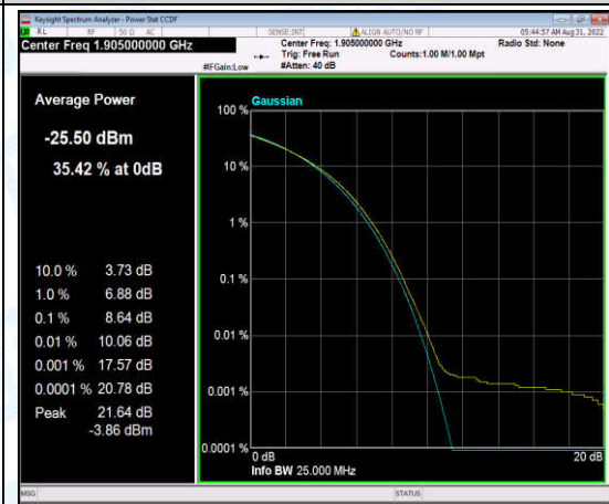
Band2-15MHz-16QAM-19150-6-0-High-8.64-<=13-PASS
