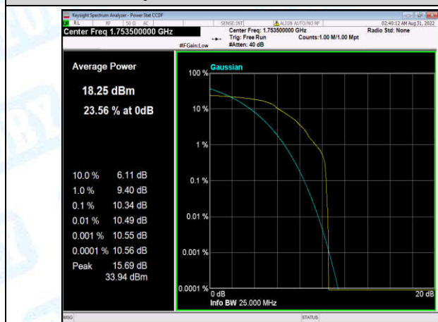
Band4-3MHz-QPSK-20385-1-0-High-10.34-<=13-PASS
