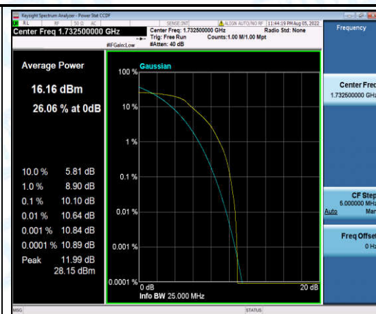
Band4-1.4MHz-16QAM-20175-6-0-Low-10.10-<=13-PASS
