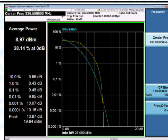
Band5-3MHz-QPSK-20525-6-0-Low-9.45-<=13-PASS
