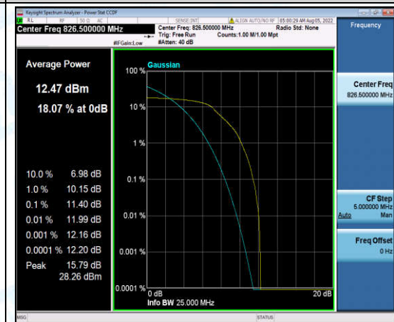
Band5-5MHz-16QAM-20425-6-0-Low-11.40-<=13-PASS
