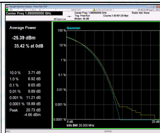
Band2-20MHz-QPSK-18900-6-0-Low-8.65-<=13-PASS
