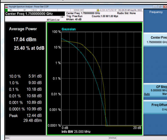
Band4-10MHz-QPSK-20350-6-0-High-10.18-<=13-PASS
