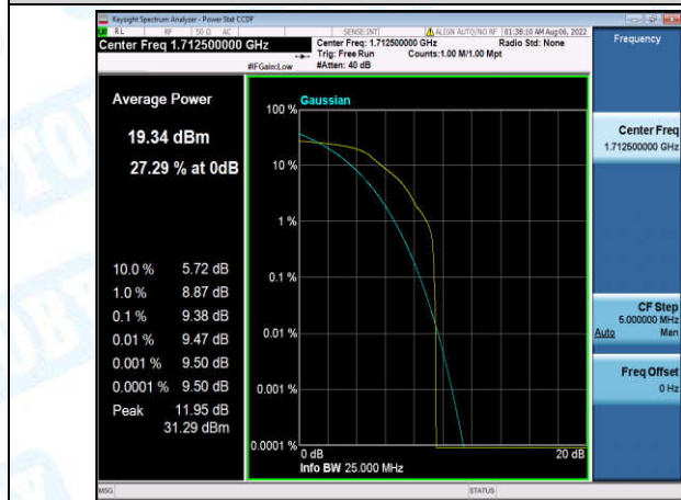
Band4-5MHz-QPSK-19975-1-0-Low-9.38-<=13-PASS
