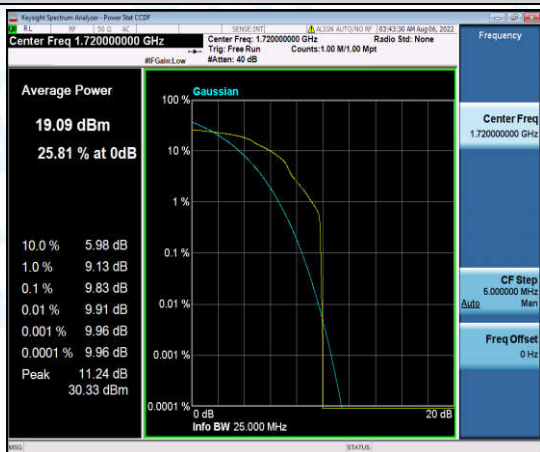
Band4-20MHz-16QAM-20050-1-0-Low-9.83-<=13-PASS
