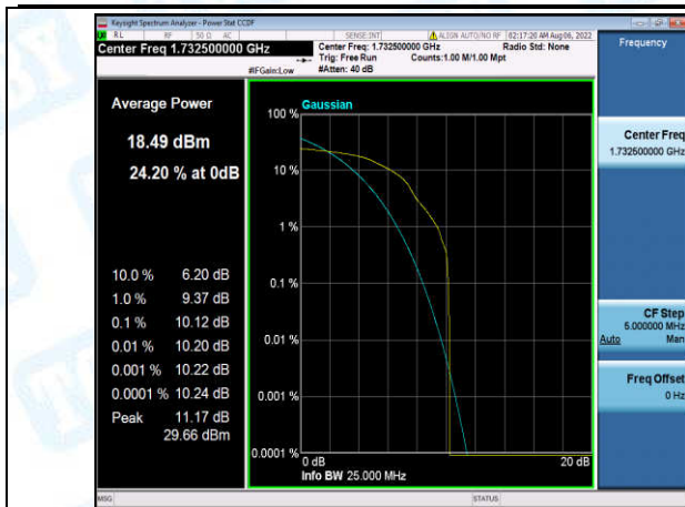
Band4-10MHz-16QAM-20175-1-0-Low-10.12-<=13-PASS
