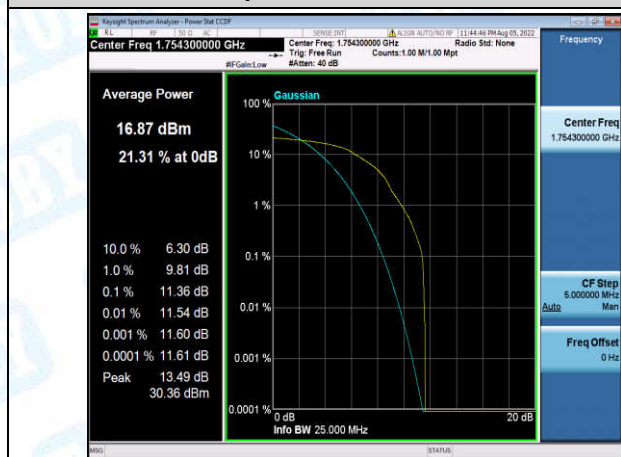
Band4-1.4MHz-16QAM-20393-1-0-High-11.36-<=13-PASS
