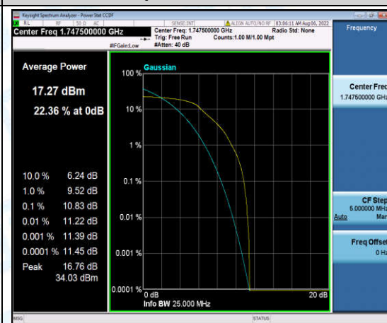
Band4-15MHz-QPSK-20325-6-0-High-10.83-<=13-PASS
