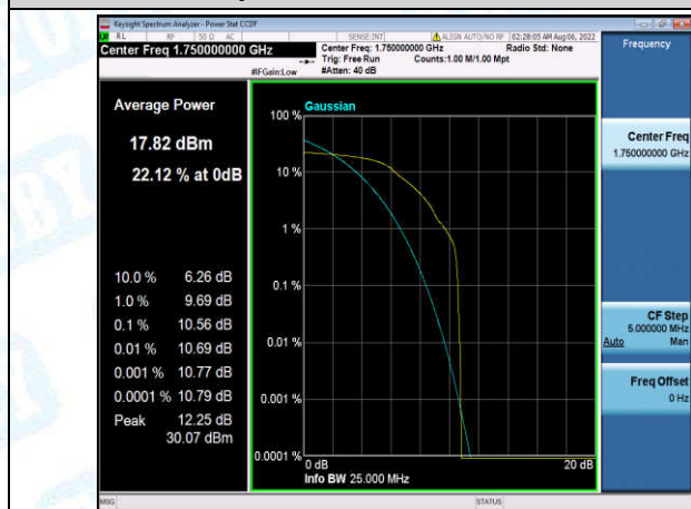
Band4-10MHz-QPSK-20350-1-0-High-10.56-<=13-PASS
