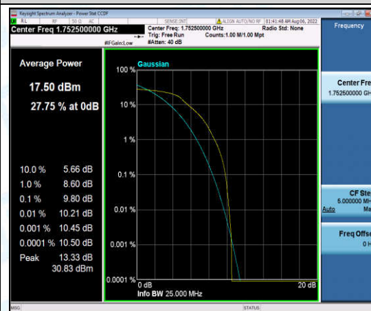
Band4-5MHz-16QAM-20375-6-0-High-9.80-<=13-PASS
