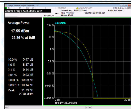
Band4-3MHz-QPSK-20175-6-0-Low-9.44-<=13-PASS
