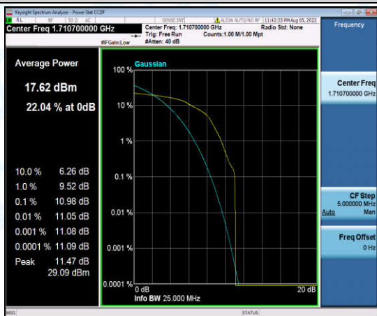
Band4-1.4MHz-16QAM-19957-1-0-Low-10.98-<=13-PASS
