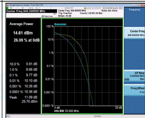
Band5-5MHz-16QAM-20625-6-0-High-9.77-<=13-PASS
