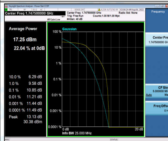
Band4-15MHz-16QAM-20325-6-0-High-10.85-<=13-PASS
