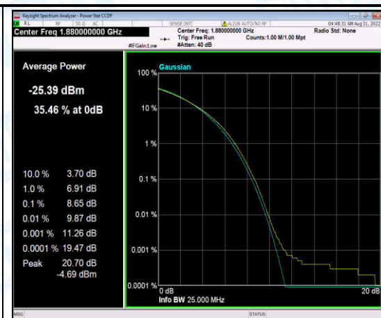
Band2-20MHz-16QAM-18900-6-0-Low-8.65-8.65-PASS
