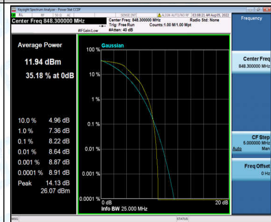
Band5-1.4MHz-16QAM-20643-6-0-High-8.22-<=13-PASS
