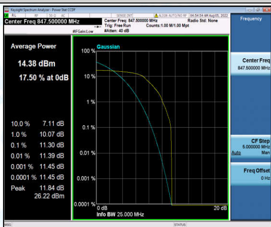
Band5-3MHz-QPSK-20635-1-0-High-11.30-<=13-PASS
