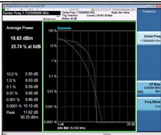
Band4-20MHz-QPSK-20175-1-0-Low-9.59-<=13-PASS
