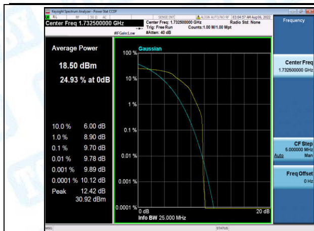
Band4-15MHz-QPSK-20175-1-0-Low-9.70-<=13-PASS
