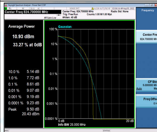
Band5-1.4MHz-QPSK-20407-6-0-Low-8.61-<=13-PASS
