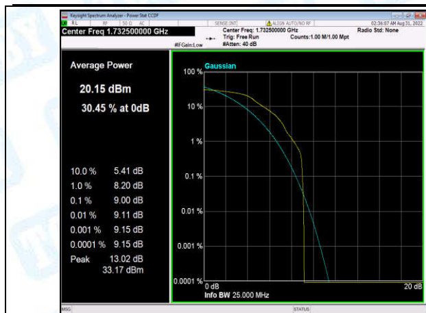
Band4-3MHz-QPSK-20175-1-0-Low-9.00-<=13-PASS
