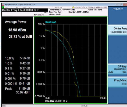
Band4-20MHz-QPSK-20300-1-0-High-9.27-<=13-PASS
