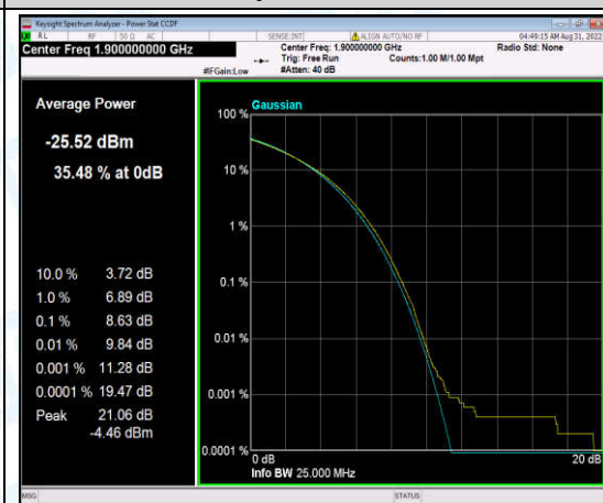
Band2-20MHz-16QAM-19100-6-0-High-8.63-8.63-PASS
