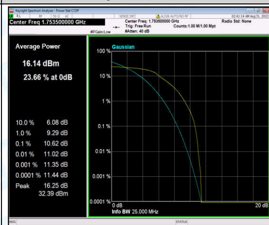
Band4-3MHz-16QAM-20385-6-0-High-10.62-<=13-PASS
