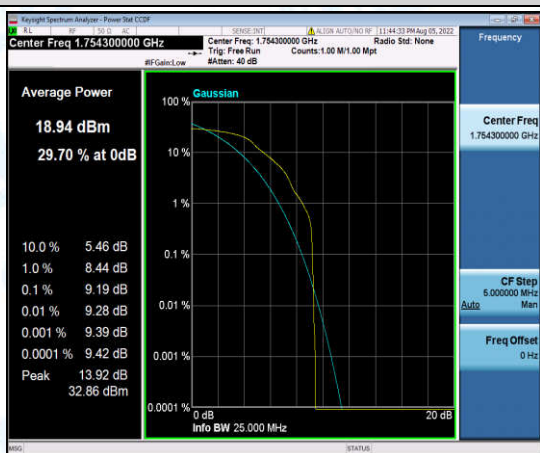
Band4-1.4MHz-QPSK-20393-1-0-High-9.19-<=13-PASS
