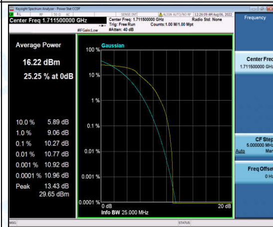
Band4-3MHz-QPSK-19965-6-0-Low-10.27-<=13-PASS
