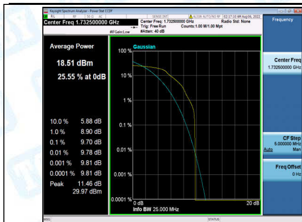
Band4-10MHz-QPSK-20175-1-0-Low-9.70-<=13-PASS
