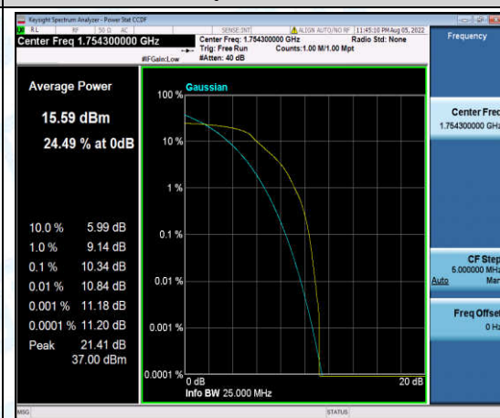
Band4-1.4MHz-16QAM-20393-6-0-High-10.34-<=13-PASS
