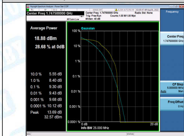
Band4-15MHz-QPSK-20325-1-0-High-9.30-<=13-PASS
