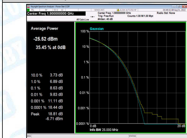
Band2-20MHz-QPSK-19100-1-0-High-8.63-<=13-PASS
