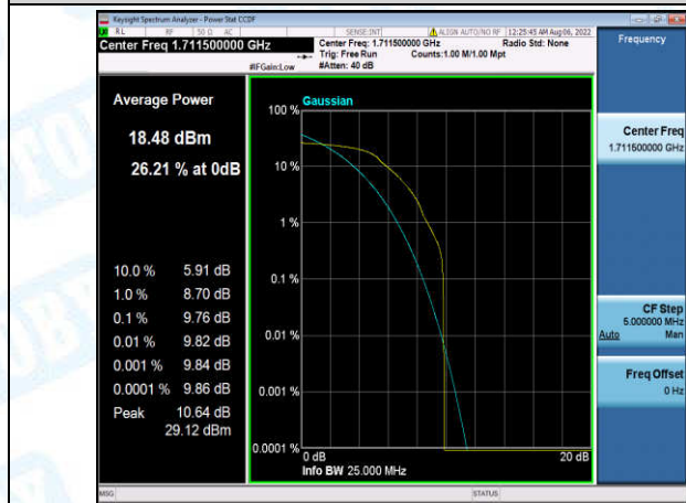
Band4-3MHz-QPSK-19965-1-0-Low-9.76-<=13-PASS
