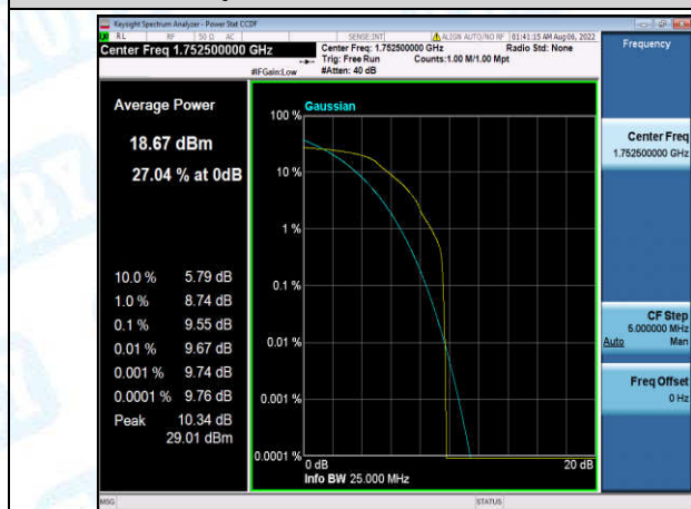
Band4-5MHz-QPSK-20375-1-0-High-9.55-<=13-PASS
