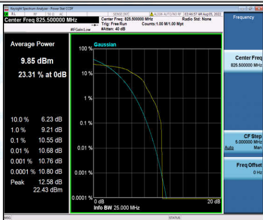
Band5-3MHz-16QAM-20415-1-0-Low-10.55-<=13-PASS
