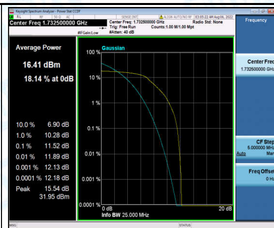
Band4-15MHz-QPSK-20175-6-0-Low-11.52-<=13-PASS
