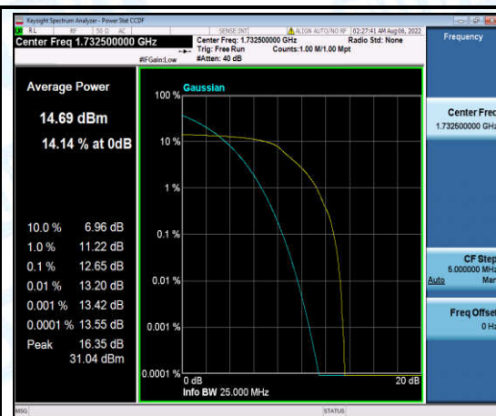
Band4-10MHz-QPSK-20175-6-0-Low-12.65-<=13-PASS
