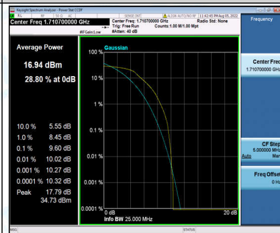
Band4-1.4MHz-QPSK-19957-6-0-Low-9.60-9.60-PASS
