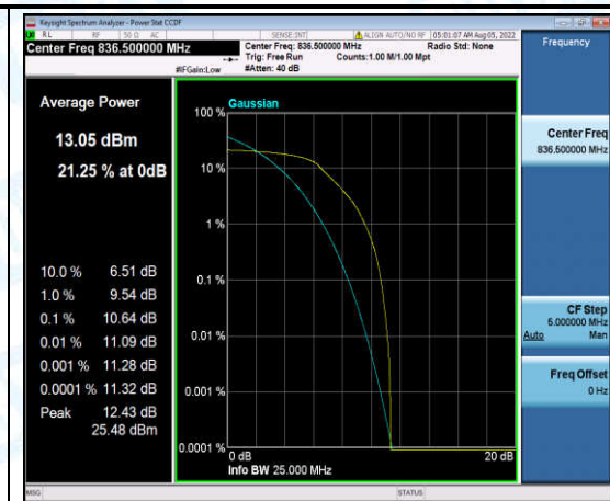
Band5-5MHz-QPSK-20525-6-0-Low-10.64-<=13-PASS
