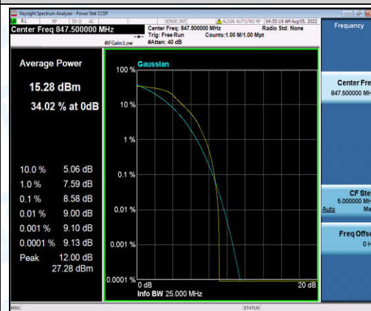
Band5-3MHz-QPSK-20635-6-0-High-8.58-<=13-PASS
