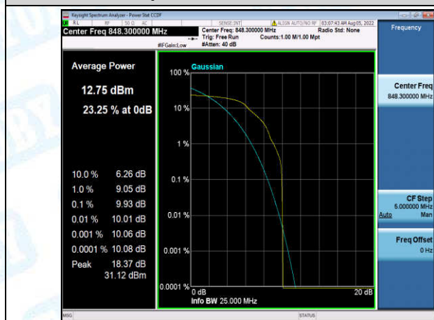
Band5-1.4MHz-QPSK-20643-1-0-High-9.93-<=13-PASS
