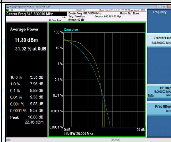
Band5-1.4MHz-QPSK-20643-6-0-High-8.89-<=13-PASS
