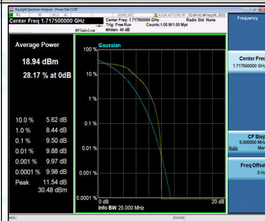
Band4-15MHz-16QAM-20025-6-0-Low-9.50-<=13-PASS
