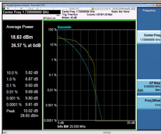
Band4-20MHz-QPSK-20050-1-0-Low-9.60-<=13-PASS
