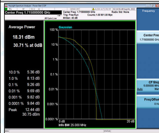
Band4-10MHz-16QAM-20000-6-0-Low-9.26-<=13-PASS
