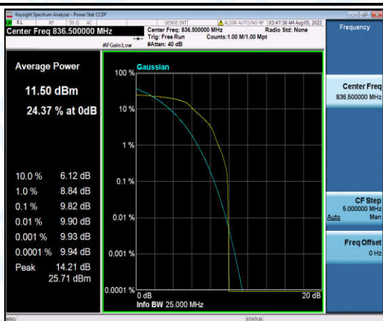
Band5-3MHz-QPSK-20525-1-0-Low-9.82-<=13-PASS
