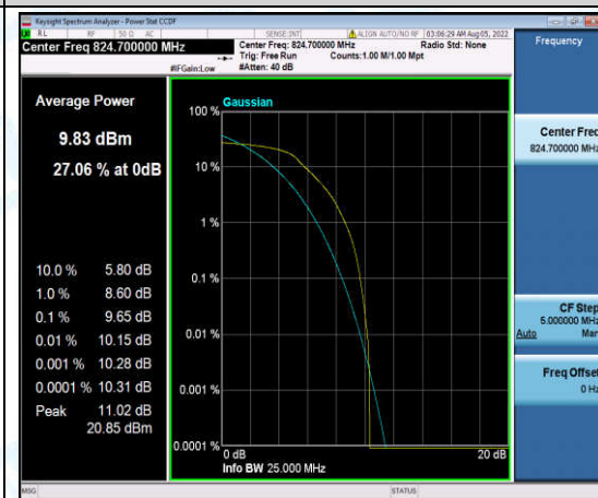
Band5-1.4MHz-16QAM-20407-6-0-Low-9.65-<=13-PASS
