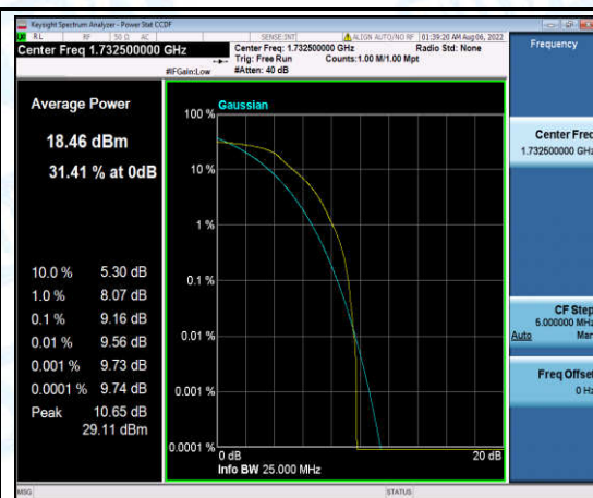
Band4-5MHz-QPSK-20175-6-0-Low-9.16-<=13-PASS
