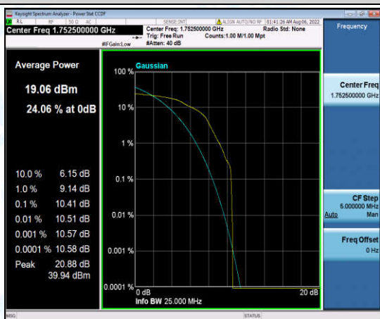
Band4-5MHz-16QAM-20375-1-0-High-10.41-<=13-PASS
