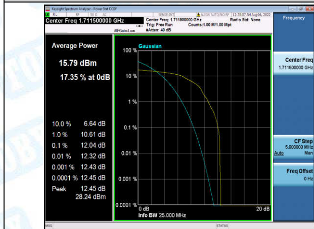
Band4-3MHz-16QAM-19965-1-0-Low-12.04-<=13-PASS
