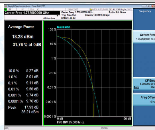
Band4-5MHz-QPSK-20375-6-0-High-9.11-<=13-PASS
