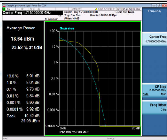
Band4-10MHz-QPSK-20000-1-0-Low-9.73-<=13-PASS
