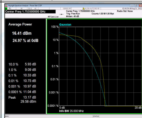
Band4-3MHz-QPSK-20385-6-0-High-10.33-<=13-PASS
