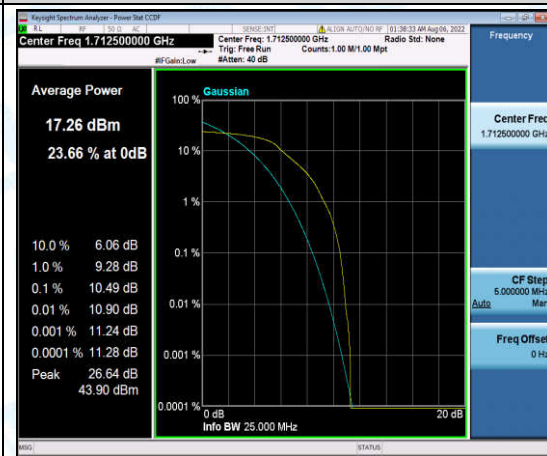
Band4-5MHz-QPSK-19975-6-0-Low-10.49-<=13-PASS
