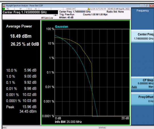
Band4-20MHz-16QAM-20300-1-0-High-9.92-<=13-PASS
