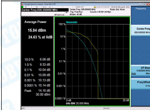
Band5-5MHz-16QAM-20425-1-0-Low-10.04-<=13-PASS
