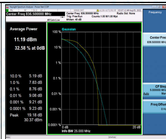
Band5-1.4MHz-QPSK-20525-6-0-Low-8.76-<=13-PASS
