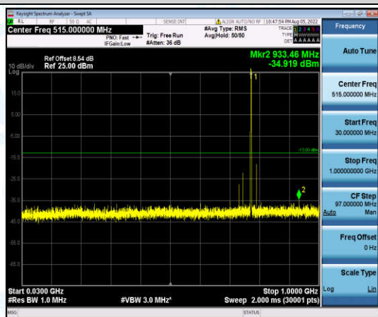
Band13-5MHz-16QAM-23205-1-0-Low-30-1000--34.92-PASS
