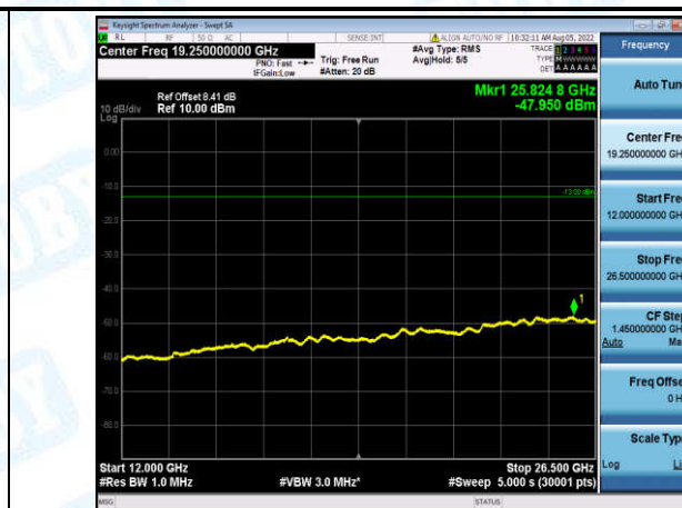
Band12-10MHz-16QAM-23130-1-0-High-12000-26500--47.95-PASS
