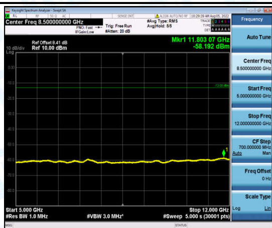
Band12-10MHz-QPSK-23130-1-0-High-5000-12000--58.19-PASS
