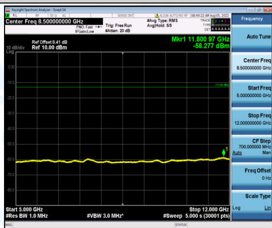
Band12-5MHz-QPSK-23095-1-0-Low-5000-12000--58.28-PASS
