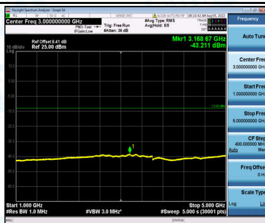
Band12-3MHz-16QAM-23095-1-0-Low-1000-5000--43.21-PASS
