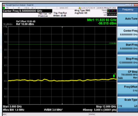
Band2-1.4MHz-16QAM-18900-1-0-Low-5000-12000--56.02-PASS
