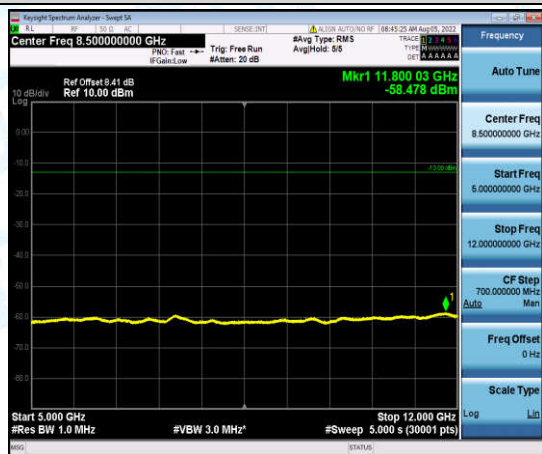
Band12-5MHz-QPSK-23035-1-0-Low-5000-12000--58.48-PASS
