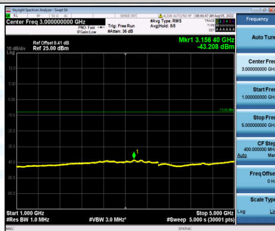
Band12-5MHz-16QAM-23035-1-0-Low-1000-5000--43.21-PASS
