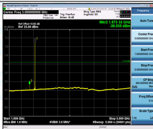
Band2-3MHz-16QAM-18615-1-0-Low-1000-5000--39.04-PASS
