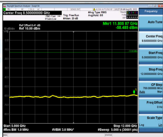
Band12-10MHz-16QAM-23095-1-0-Low-5000-12000--58.49-PASS
