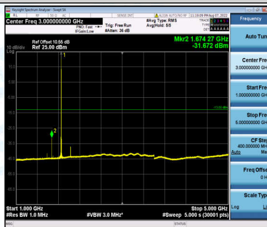
Band2-3MHz-QPSK-18615-1-0-Low-1000-5000--31.67-PASS
