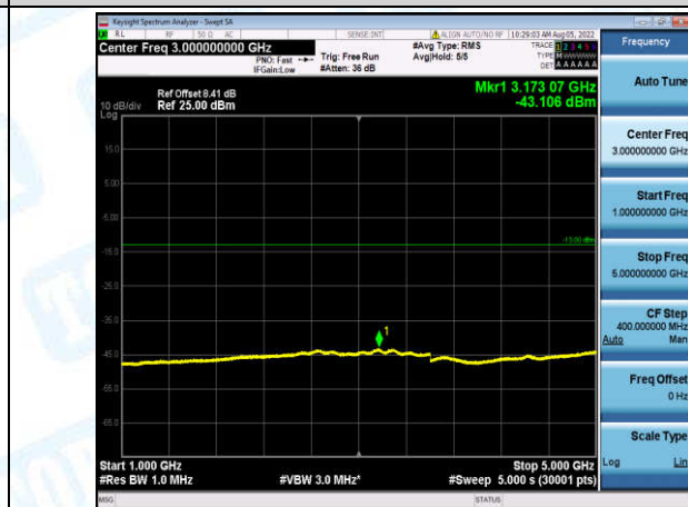
Band12-10MHz-QPSK-23130-1-0-High-1000-5000--43.11-PASS
