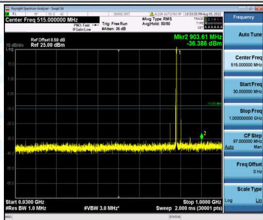
Band13-5MHz-QPSK-23255-1-0-High-30-1000--36.39-PASS
