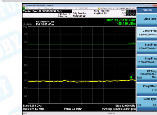
Band12-10MHz-QPSK-23095-1-0-Low-5000-12000--58.42-PASS
