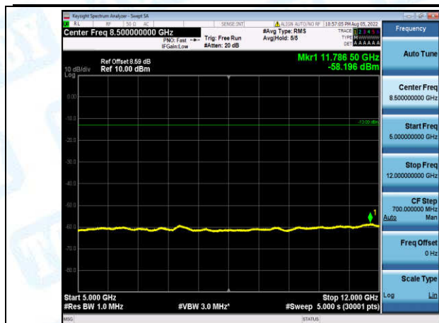
Band13-5MHz-16QAM-23255-1-0-High-5000-12000--58.2-PASS
