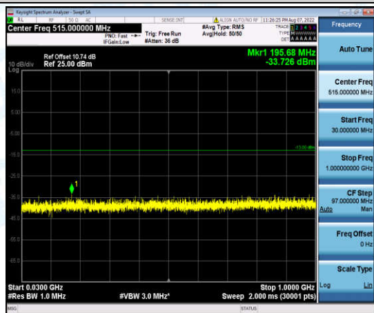
Band2-3MHz-QPSK-19185-1-0-High-30-1000--33.73-PASS
