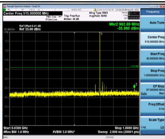
Band12-10MHz-16QAM-23095-1-0-Low-30-1000--35.86-PASS
