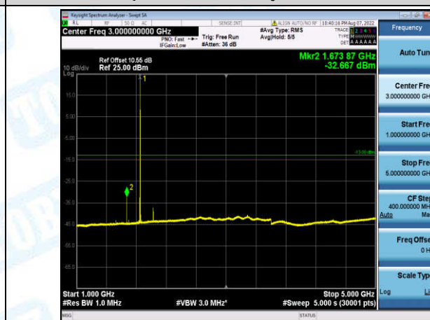
Band2-1.4MHz-16QAM-18607-1-0-Low-1000-5000--32.67-PASS
