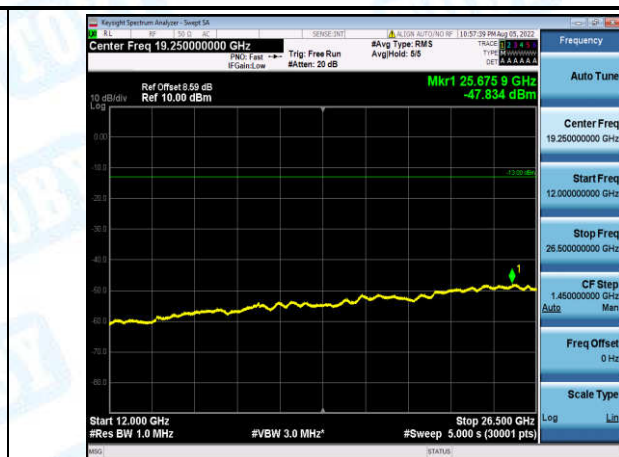
Band13-5MHz-16QAM-23255-1-0-High-12000-26500--47.83-PASS
