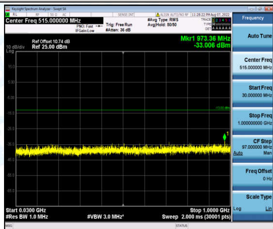
Band2-3MHz-16QAM-19185-1-0-High-30-1000--33.01-PASS
