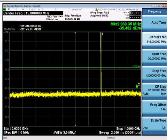
Band12-10MHz-16QAM-23060-1-0-Low-30-1000--35.48-PASS
