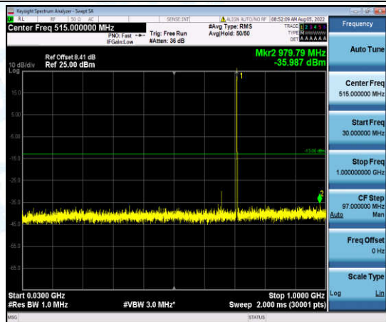
Band12-5MHz-QPSK-23155-1-0-High-30-1000--35.99-PASS
