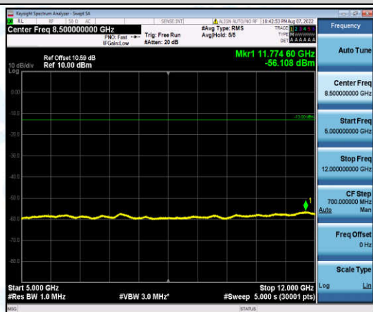
Band2-1.4MHz-QPSK-18900-1-0-Low-5000-12000--56.11-PASS
