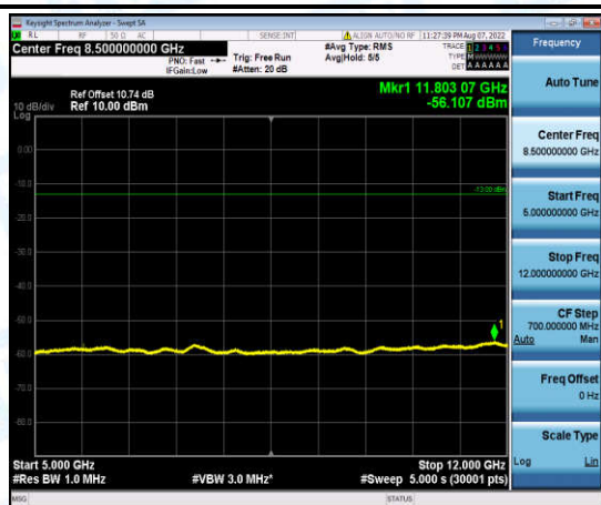
Band2-3MHz-QPSK-19185-1-0-High-5000-12000--56.11-PASS
