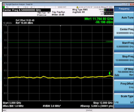
Band2-3MHz-16QAM-18615-1-0-Low-5000-12000--56.2-PASS
