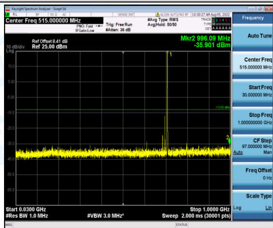
Band12-10MHz-16QAM-23130-1-0-High-30-1000--35.9-PASS
