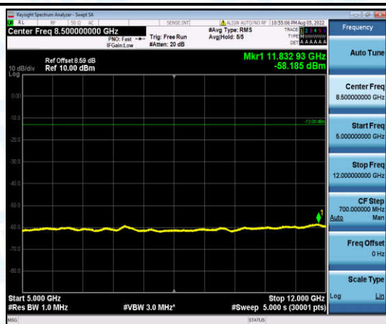
Band13-5MHz-QPSK-23255-1-0-High-5000-12000--58.19-PASS
