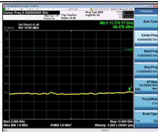
Band12-5MHz-16QAM-23155-1-0-High-5000-12000--58.48-PASS
