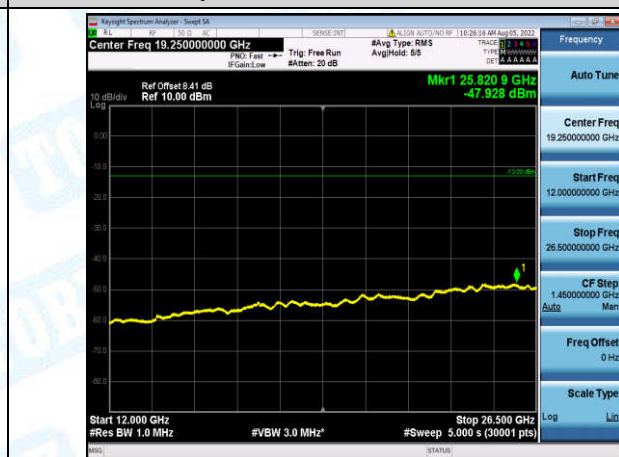
Band12-10MHz-QPSK-23095-1-0-Low-12000-26500--47.93-PASS
