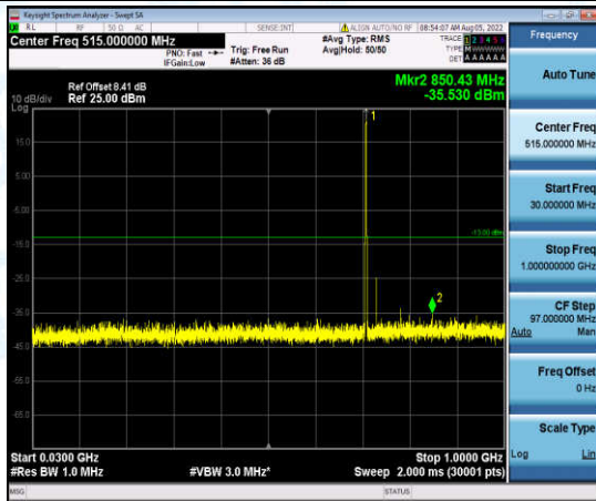
Band12-5MHz-16QAM-23155-1-0-High-30-1000--35.53-PASS
