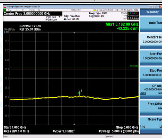
Band12-5MHz-QPSK-23035-1-0-Low-1000-5000--43.23-PASS
