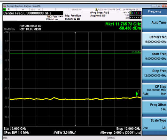
Band12-3MHz-16QAM-23095-1-0-Low-5000-12000--58.44-PASS
