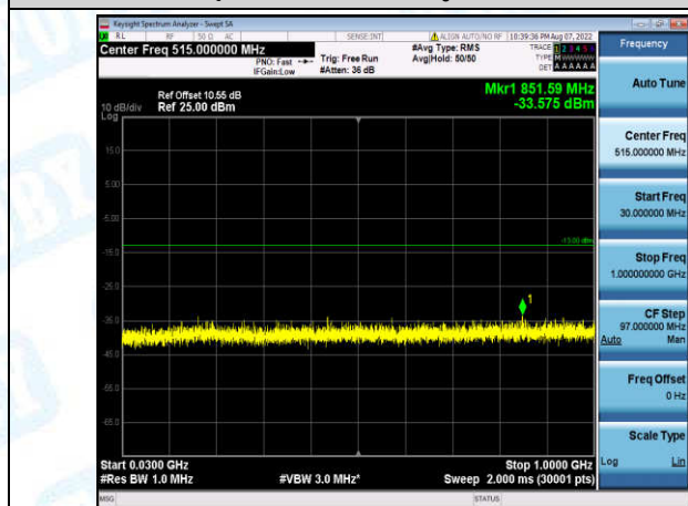
Band2-1.4MHz-16QAM-18607-1-0-Low-30-1000--33.58-PASS
