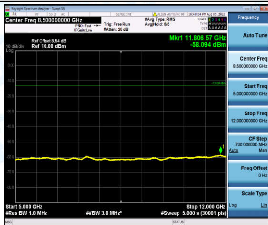
Band13-5MHz-16QAM-23205-1-0-Low-5000-12000--58.09-PASS
