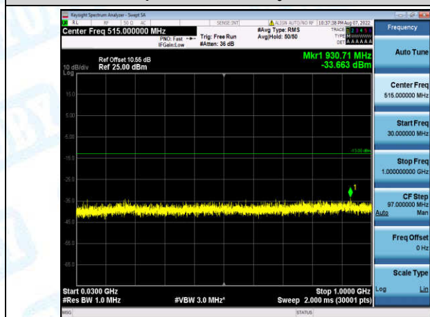
Band2-1.4MHz-QPSK-18607-1-0-Low-30-1000--33.66-PASS
