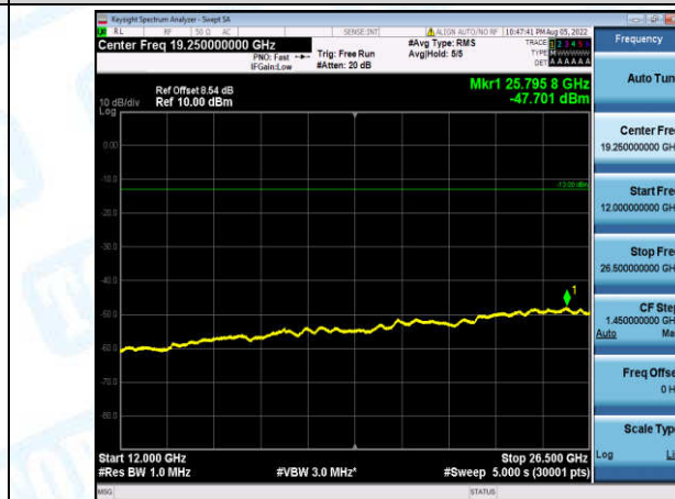
Band13-5MHz-QPSK-23205-1-0-Low-12000-26500--47.7-PASS
