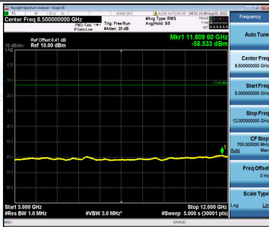
Band12-5MHz-16QAM-23095-1-0-Low-5000-12000--58.53-PASS
