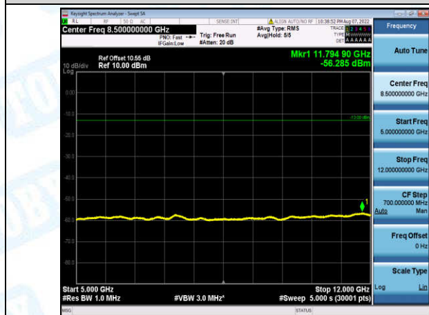
Band2-1.4MHz-QPSK-18607-1-0-Low-5000-12000--56.29-PASS
