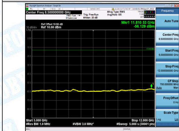
Band2-1.4MHz-16QAM-18607-1-0-Low-5000-12000--56.13-PASS
