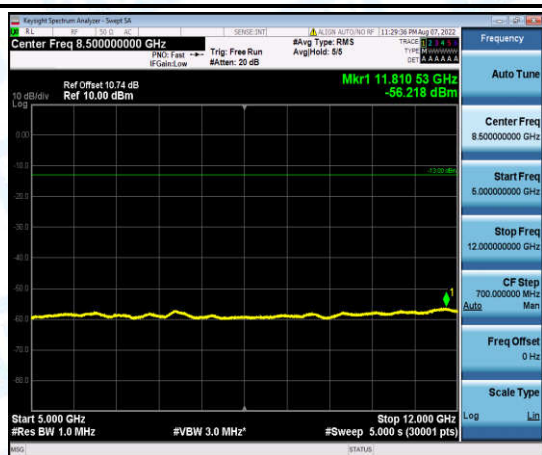
Band2-3MHz-16QAM-19185-1-0-High-5000-12000--56.22-PASS
