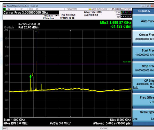
Band2-3MHz-QPSK-18900-1-0-Low-1000-5000--31.13-PASS
