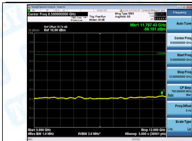
Band2-1.4MHz-QPSK-19193-1-0-High-5000-12000--56.1-PASS
