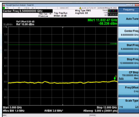
Band13-5MHz-16QAM-23230-1-0-Low-5000-12000--58.24-PASS
