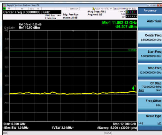
Band2-3MHz-QPSK-18615-1-0-Low-5000-12000--56.21-PASS
