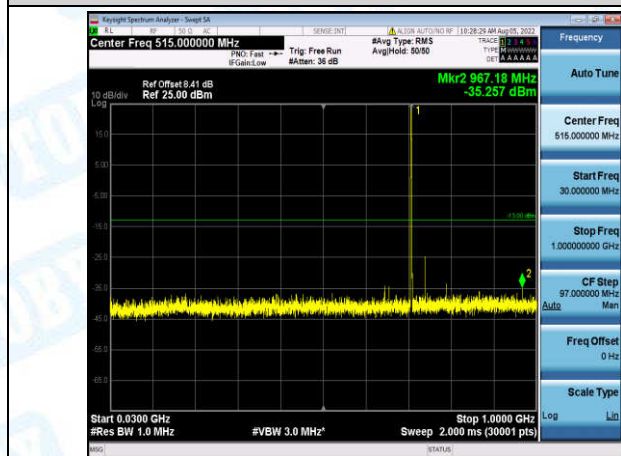
Band12-10MHz-QPSK-23130-1-0-High-30-1000--35.26-PASS
