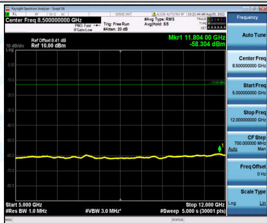
Band12-10MHz-QPSK-23060-1-0-Low-5000-12000--58.3-PASS
