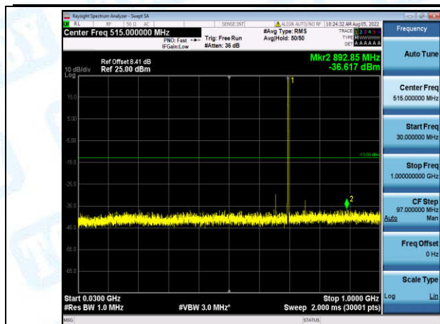
Band12-10MHz-QPSK-23095-1-0-Low-30-1000--36.62-PASS
