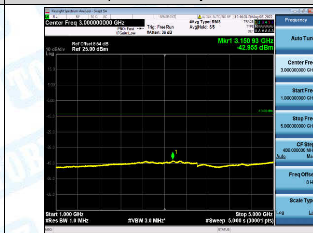
Band13-5MHz-QPSK-23205-1-0-Low-1000-5000--42.96-PASS
