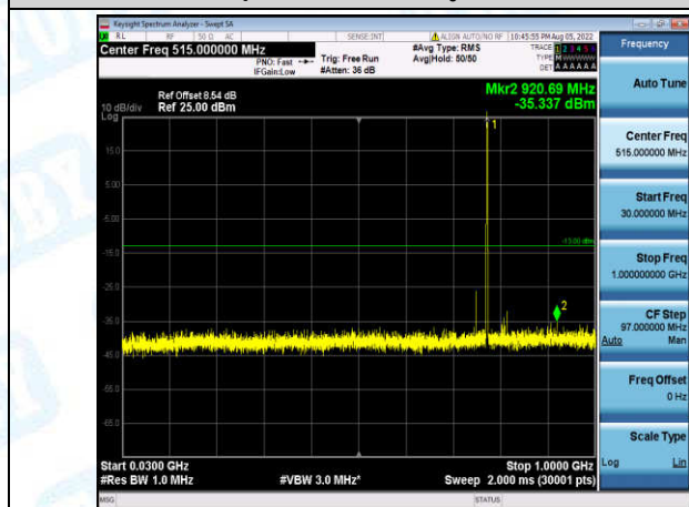
Band13-5MHz-QPSK-23205-1-0-Low-30-1000--35.34-PASS
