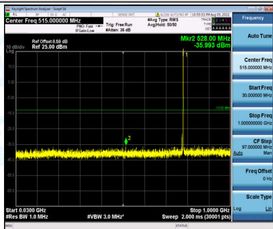
Band13-5MHz-16QAM-23255-1-0-High-30-1000--35.99-PASS
