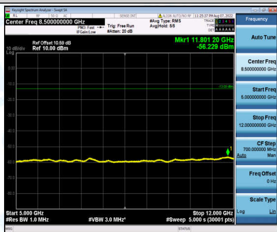
Band2-3MHz-16QAM-18900-1-0-Low-5000-12000--56.23-PASS
