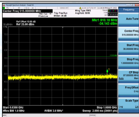
Band2-3MHz-QPSK-18615-1-0-Low-30-1000--34.14-PASS
