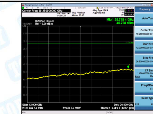
Band2-1.4MHz-16QAM-18607-1-0-Low-12000-26500--45.8-PASS
