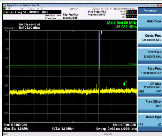
Band12-3MHz-16QAM-23165-1-0-High-30-1000--35.98-PASS
