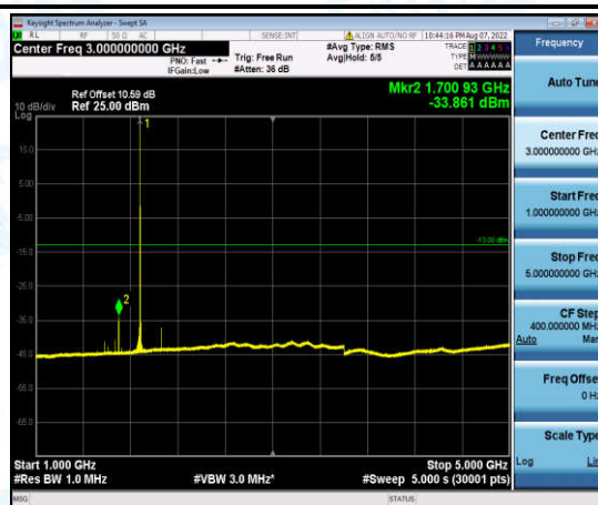
Band2-1.4MHz-16QAM-18900-1-0-Low-1000-5000--33.86-PASS
