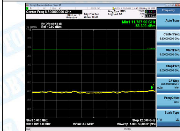
Band13-5MHz-QPSK-23205-1-0-Low-5000-12000--58.31-PASS
