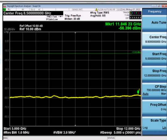
Band2-3MHz-QPSK-18900-1-0-Low-5000-12000--56.4-PASS
