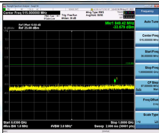
Band2-1.4MHz-16QAM-18900-1-0-Low-30-1000--33.68-PASS
