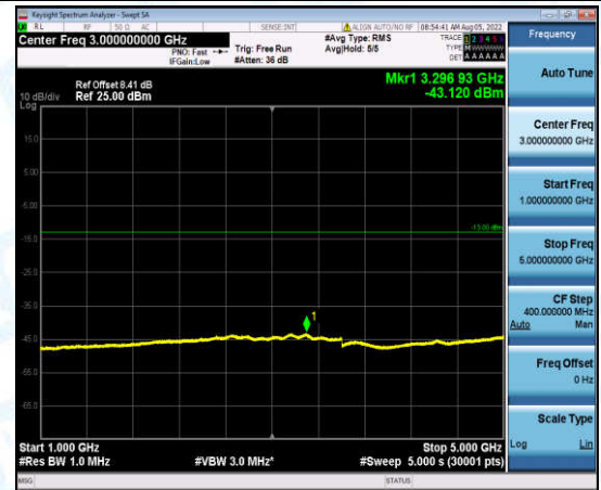
Band12-5MHz-16QAM-23155-1-0-High-1000-5000--43.12-PASS
