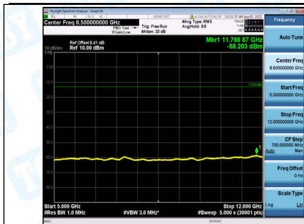
Band12-10MHz-16QAM-23130-1-0-High-5000-12000--58.2-PASS
