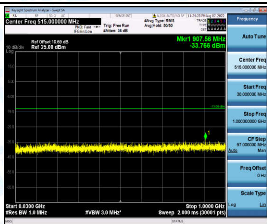
Band2-3MHz-16QAM-18900-1-0-Low-30-1000--33.77-PASS
