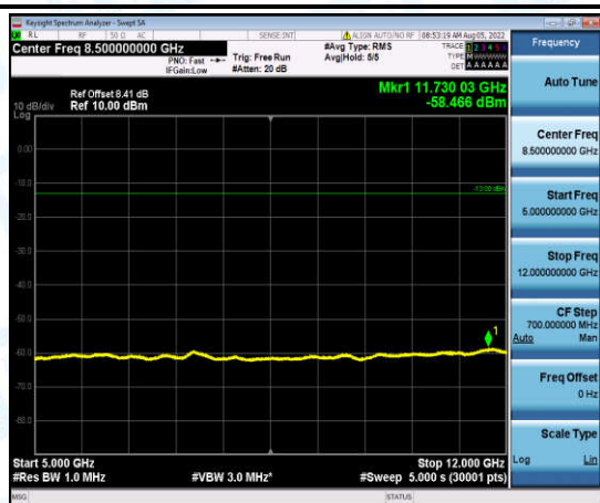
Band12-5MHz-QPSK-23155-1-0-High-5000-12000--58.47-PASS
