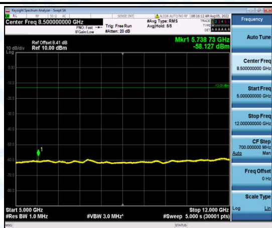
Band12-3MHz-16QAM-23165-1-0-High-5000-12000--58.13-PASS
