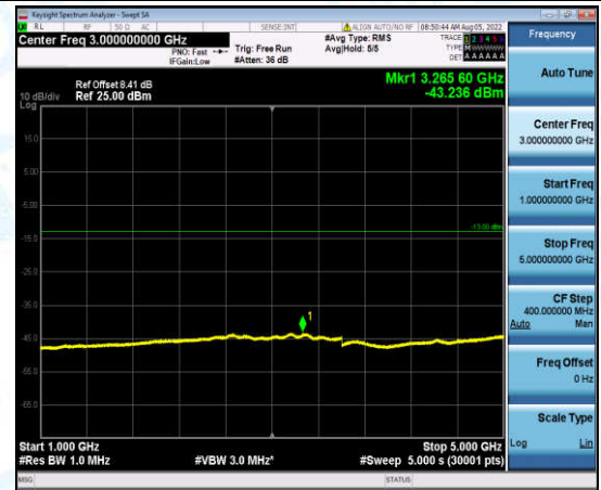
Band12-5MHz-16QAM-23095-1-0-Low-1000-5000--43.24-PASS
