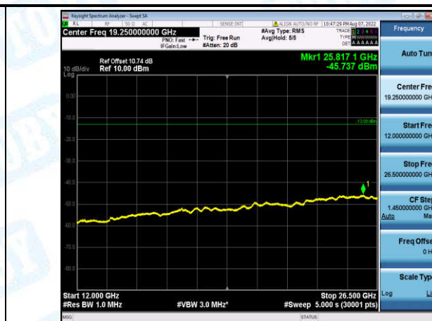
Band2-1.4MHz-QPSK-19193-1-0-High-12000-26500--45.74-PASS
