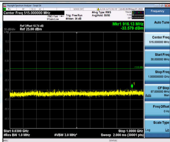
Band2-1.4MHz-QPSK-19193-1-0-High-30-1000--33.58-PASS
