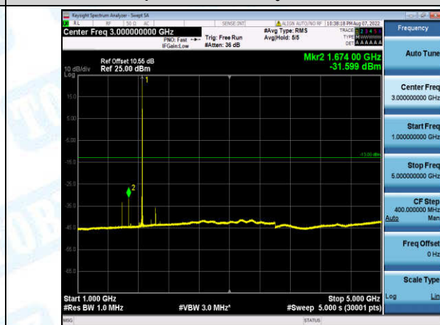
Band2-1.4MHz-QPSK-18607-1-0-Low-1000-5000--31.6-PASS
