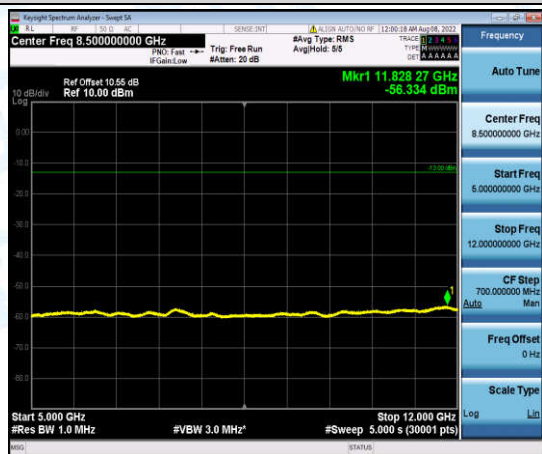
Band2-5MHz-QPSK-18625-1-0-Low-5000-12000--56.33-PASS
