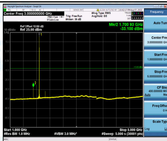
Band2-1.4MHz-QPSK-18900-1-0-Low-1000-5000--33.1-PASS
