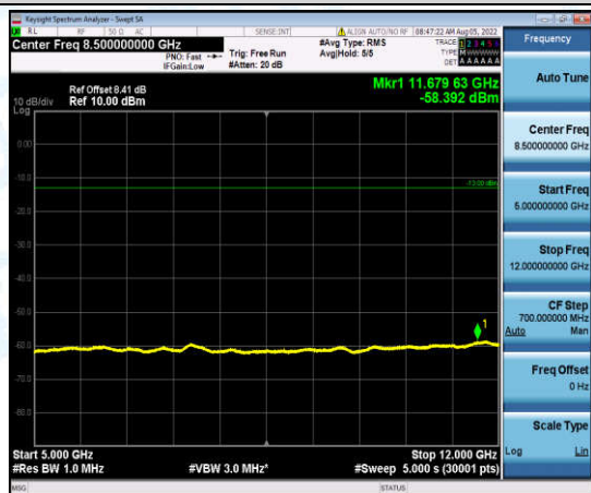
Band12-5MHz-16QAM-23035-1-0-Low-5000-12000--58.39-PASS
