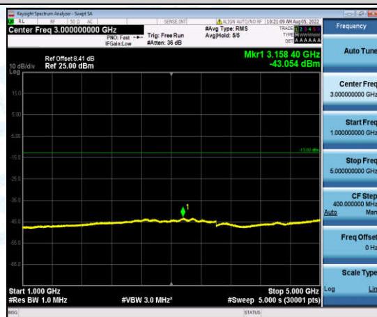
Band12-10MHz-QPSK-23060-1-0-Low-1000-5000--43.05-PASS
