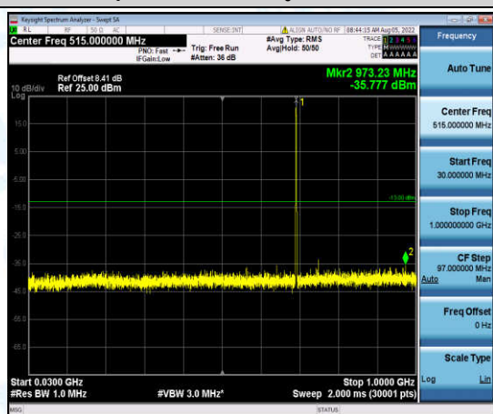
Band12-5MHz-QPSK-23035-1-0-Low-30-1000--35.78-PASS
