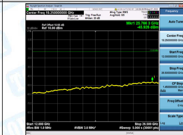
Band2-1.4MHz-QPSK-18607-1-0-Low-12000-26500--45.93-PASS
