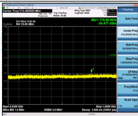
Band2-5MHz-QPSK-18625-1-0-Low-30-1000--34.48-PASS
