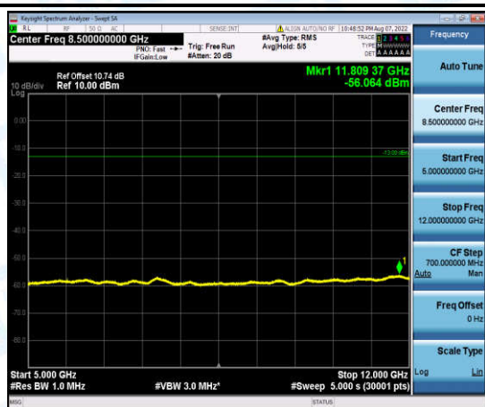
Band2-1.4MHz-16QAM-19193-1-0-High-5000-12000--56.06-PASS
