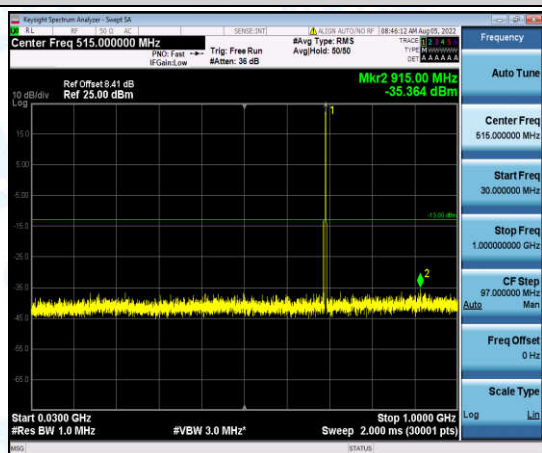
Band12-5MHz-16QAM-23035-1-0-Low-30-1000--35.36-PASS
