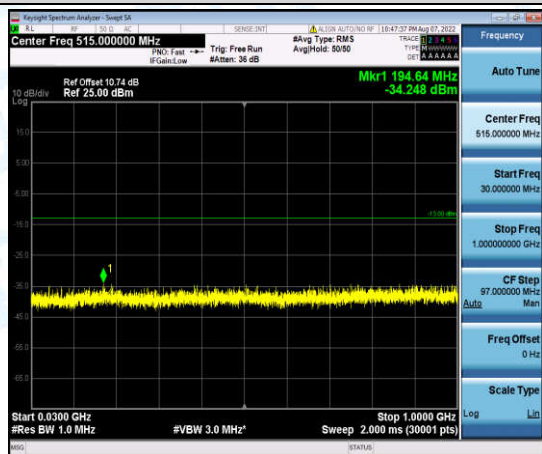
Band2-1.4MHz-16QAM-19193-1-0-High-30-1000--34.25-PASS
