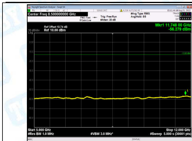
Band2-20MHz-QPSK-19100-1-0-High-5000-12000--56.28-PASS
