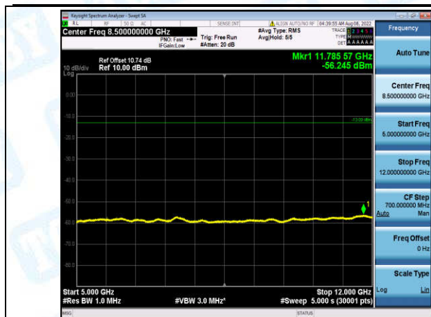
Band2-10MHz-16QAM-19150-1-0-High-5000-12000--56.25-PASS
