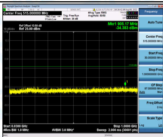
Band2-10MHz-16QAM-18900-1-0-Low-30-1000--34.38-PASS
