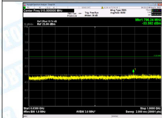
Band2-15MHz-16QAM-19150-1-0-High-30-1000--33.59-PASS
