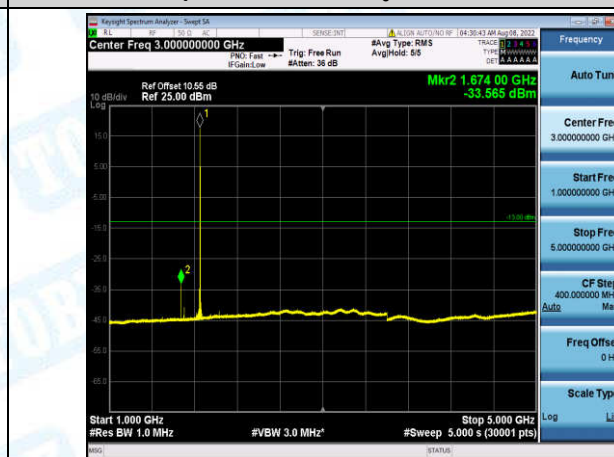
Band2-10MHz-16QAM-18650-1-0-Low-1000-5000--33.57-PASS
