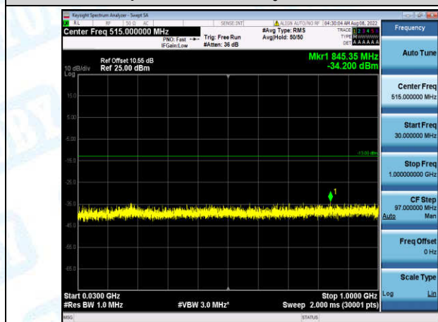
Band2-10MHz-16QAM-18650-1-0-Low-30-1000--34.2-PASS
