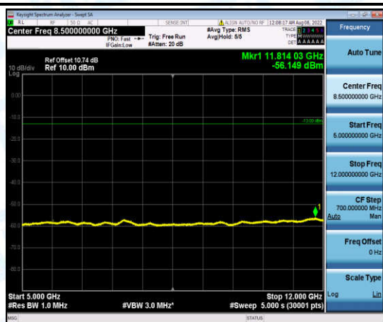
Band2-5MHz-QPSK-19175-1-0-High-5000-12000--56.15-PASS
