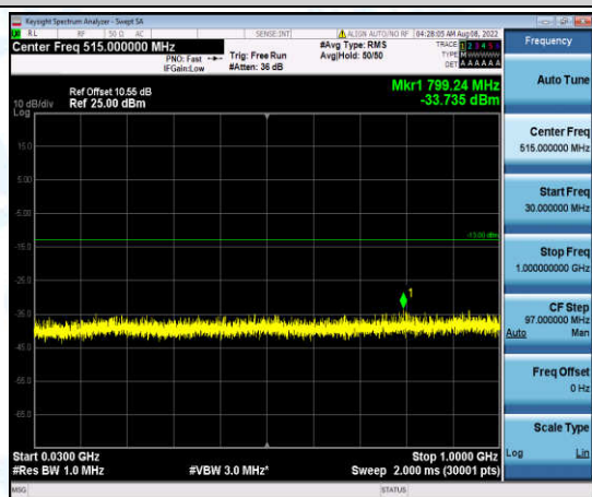
Band2-10MHz-QPSK-18650-1-0-Low-30-1000--33.74-PASS
