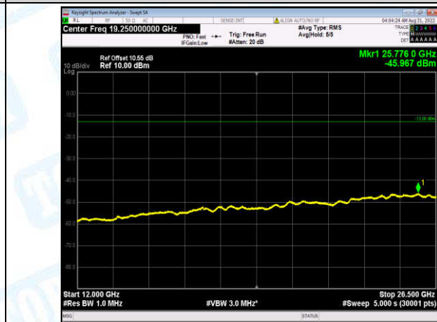
Band2-15MHz-16QAM-18675-1-0-Low-12000-26500--45.97-PASS
