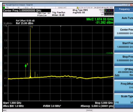
Band2-10MHz-QPSK-18650-1-0-Low-1000-5000--31.28-PASS
