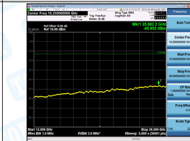
Band2-10MHz-16QAM-18650-1-0-Low-12000-26500--45.95-PASS
