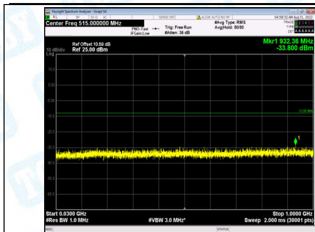
Band2-20MHz-16QAM-18900-1-0-Low-30-1000--33.8-PASS
