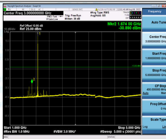
Band2-5MHz-16QAM-18625-1-0-Low-1000-5000--30.89-PASS
