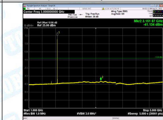
Band2-15MHz-16QAM-18675-1-0-Low-1000-5000--41.13-PASS
