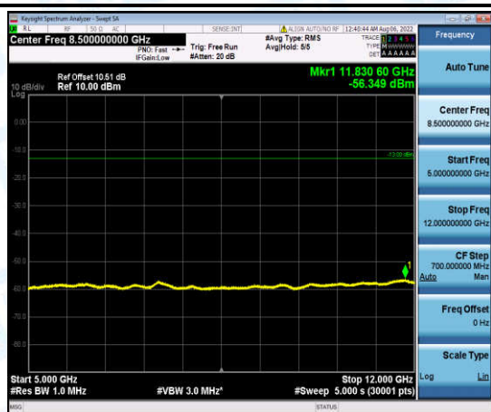
Band4-3MHz-QPSK-20385-1-0-High-5000-12000--56.35-PASS
