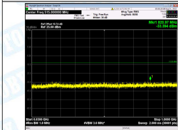
Band2-20MHz-QPSK-19100-1-0-High-30-1000--33.39-PASS
