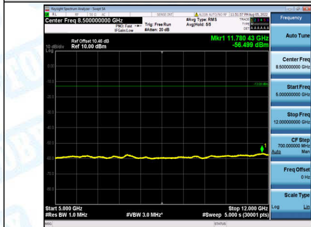
Band4-1.4MHz-QPSK-19957-1-0-Low-5000-12000--56.5-PASS
