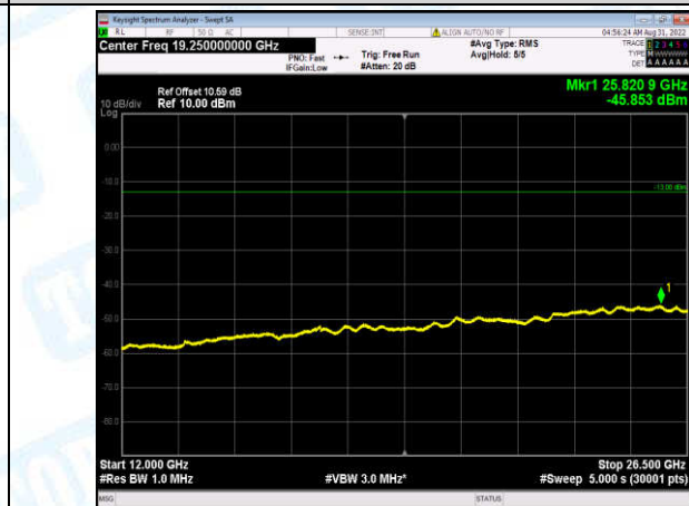
Band2-20MHz-16QAM-18700-1-0-Low-12000-26500--45.85-PASS
