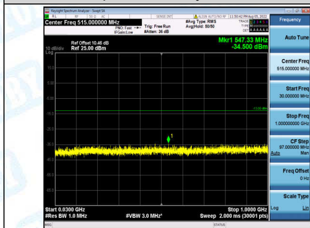
Band4-1.4MHz-QPSK-19957-1-0-Low-30-1000--34.5-PASS
