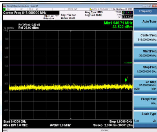
Band2-5MHz-16QAM-18900-1-0-Low-30-1000--33.52-PASS
