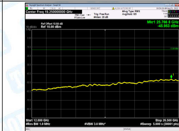
Band2-20MHz-QPSK-18700-1-0-Low-12000-26500--45.95-PASS
