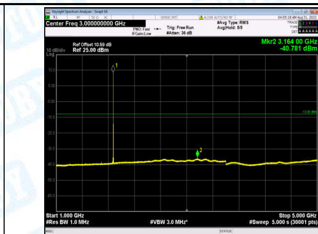
Band2-15MHz-QPSK-18900-1-0-Low-1000-5000--40.78-PASS
