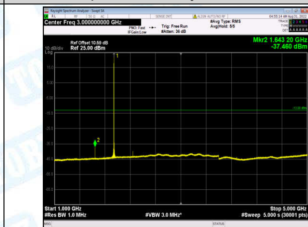
Band2-20MHz-16QAM-18700-1-0-Low-1000-5000--37.46-PASS
