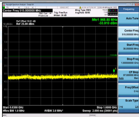
Band4-1.4MHz-16QAM-20393-1-0-High-30-1000--33.91-PASS
