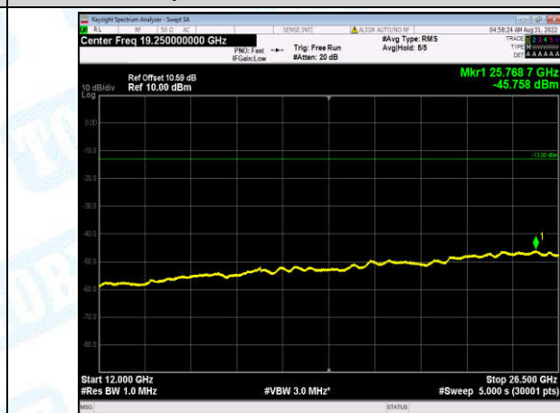
Band2-20MHz-QPSK-18900-1-0-Low-12000-26500--45.76-PASS
