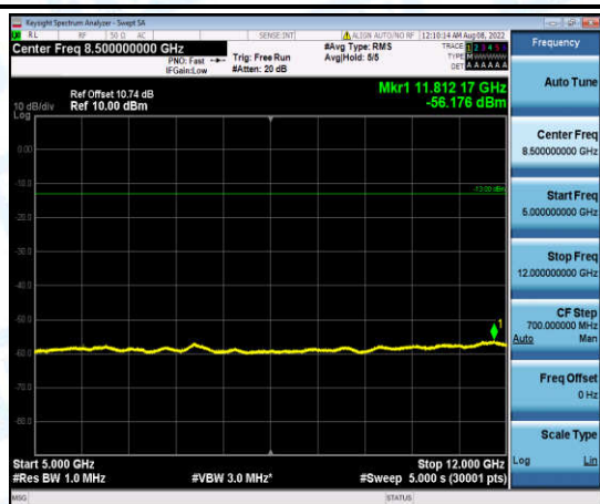
Band2-5MHz-16QAM-19175-1-0-High-5000-12000--56.18-PASS
