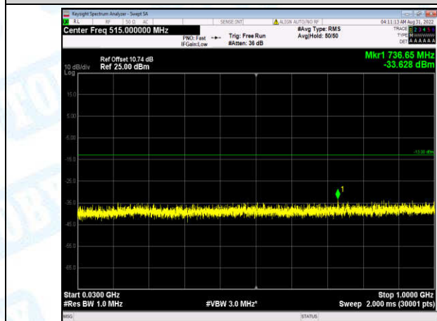
Band2-15MHz-QPSK-19150-1-0-High-30-1000--33.63-PASS
