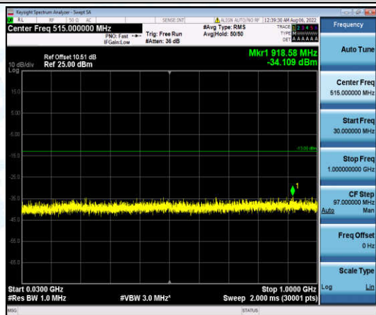
Band4-3MHz-QPSK-20385-1-0-High-30-1000--34.11-PASS
