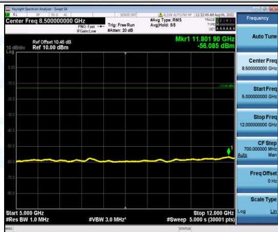
Band4-3MHz-QPSK-19965-1-0-Low-5000-12000--56.09-PASS
