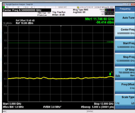
Band4-3MHz-16QAM-19965-1-0-Low-5000-12000--56.41-PASS
