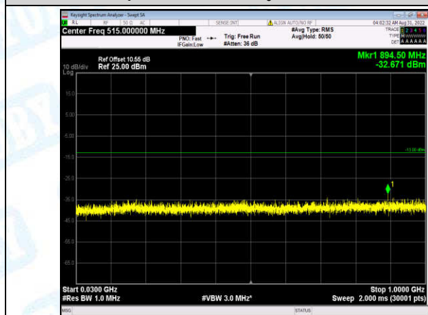
Band2-15MHz-16QAM-18675-1-0-Low-30-1000--32.67-PASS
