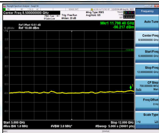
Band4-1.4MHz-16QAM-20393-1-0-High-5000-12000--56.22-PASS
