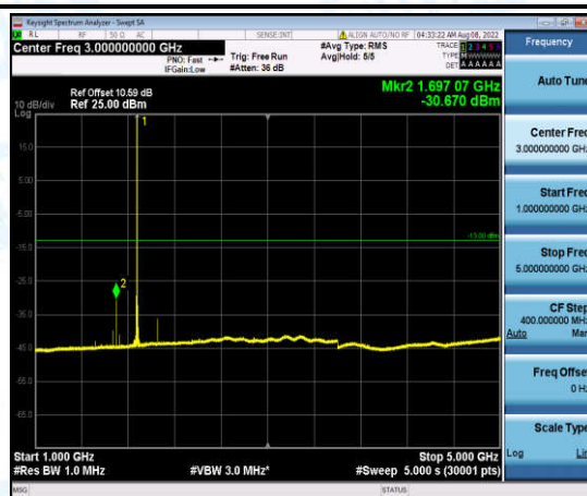
Band2-10MHz-QPSK-18900-1-0-Low-1000-5000--30.67-PASS
