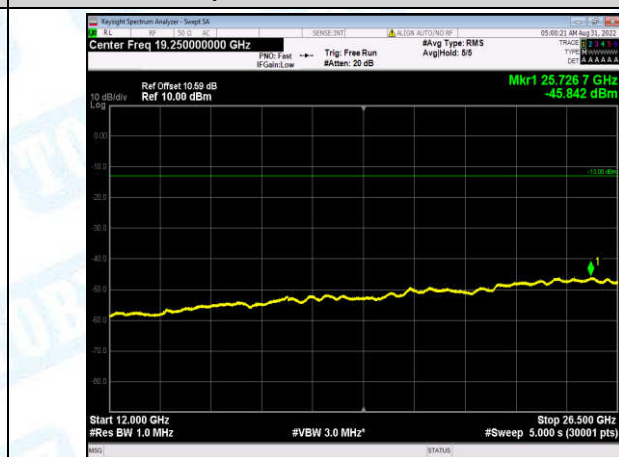
Band2-20MHz-16QAM-18900-1-0-Low-12000-26500--45.84-PASS
