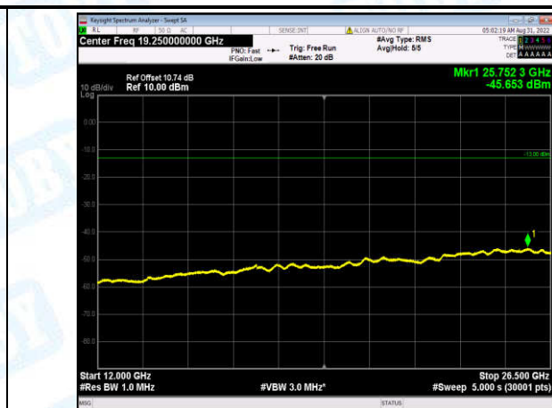
Band2-20MHz-QPSK-19100-1-0-High-12000-26500--45.65-PASS
