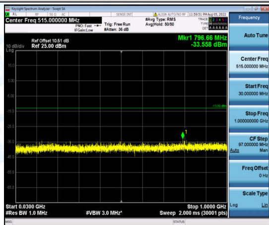
Band4-1.4MHz-QPSK-20393-1-0-High-30-1000--33.56-PASS
