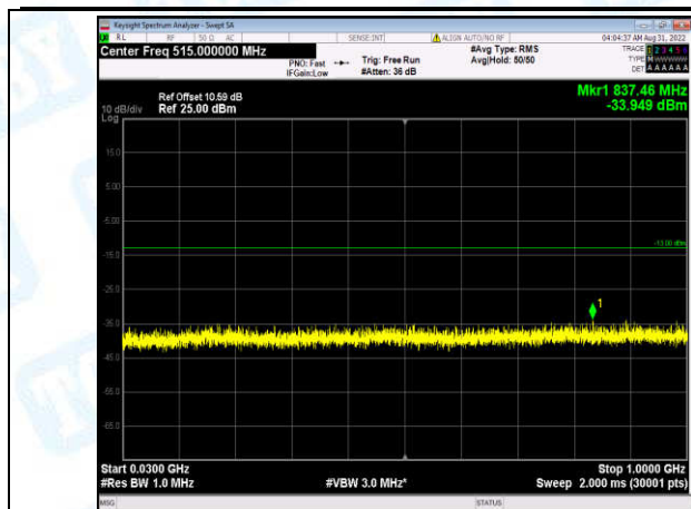
Band2-15MHz-QPSK-18900-1-0-Low-30-1000--33.95-PASS
