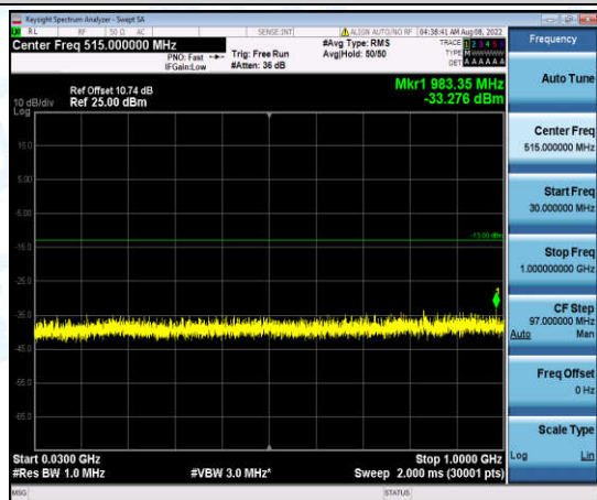
Band2-10MHz-16QAM-19150-1-0-High-30-1000--33.28-PASS
