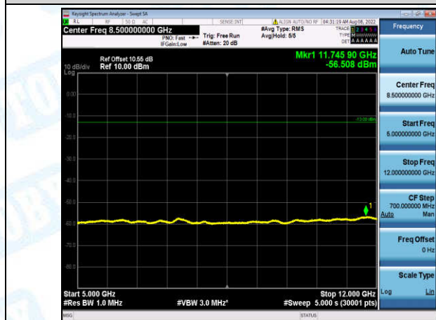
Band2-10MHz-16QAM-18650-1-0-Low-5000-12000--56.51-PASS
