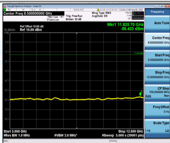
Band2-5MHz-16QAM-18900-1-0-Low-5000-12000--56.42-PASS
