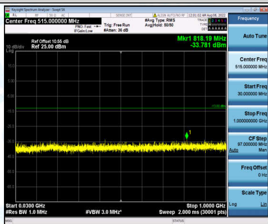
Band2-5MHz-16QAM-18625-1-0-Low-30-1000--33.78-PASS
