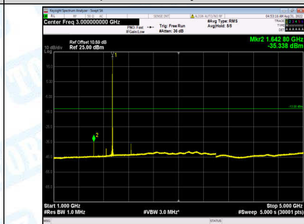
Band2-20MHz-QPSK-18700-1-0-Low-1000-5000--35.34-PASS
