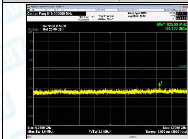
Band2-15MHz-QPSK-18675-1-0-Low-30-1000--34.1-PASS
