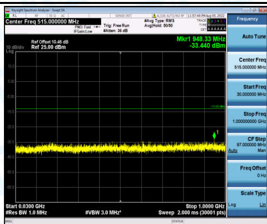
Band4-1.4MHz-16QAM-20175-1-0-Low-30-1000--33.44-PASS
