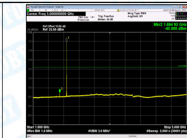
Band2-15MHz-16QAM-18900-1-0-Low-1000-5000--40.99-PASS
