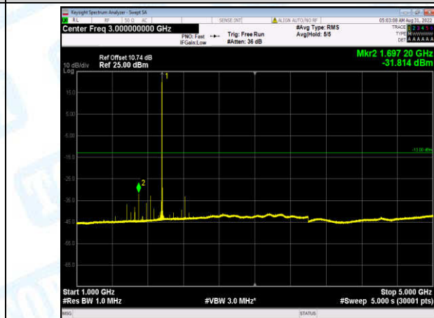
Band2-20MHz-16QAM-19100-1-0-High-1000-5000--31.81-PASS
