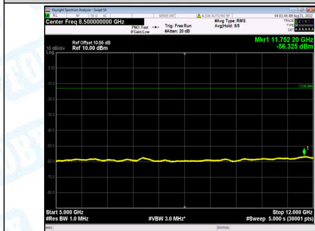
Band2-15MHz-QPSK-18675-1-0-Low-5000-12000--56.33-PASS
