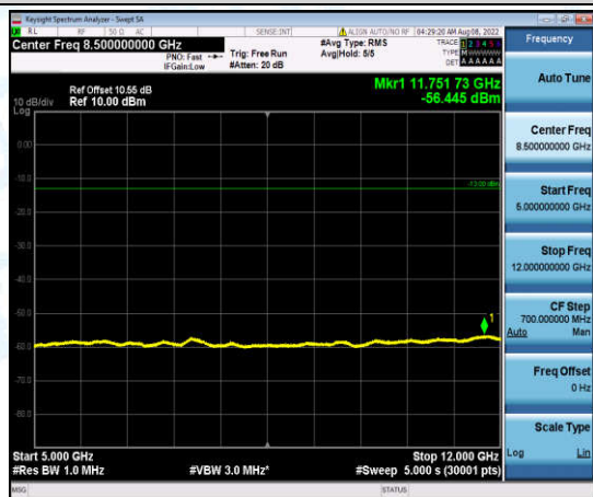
Band2-10MHz-QPSK-18650-1-0-Low-5000-12000--56.45-PASS
