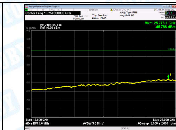
Band2-15MHz-QPSK-19150-1-0-High-12000-26500--45.79-PASS
