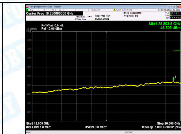
Band2-15MHz-16QAM-19150-1-0-High-12000-26500--45.81-PASS
