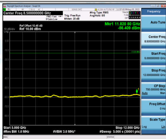
Band4-1.4MHz-QPSK-20175-1-0-Low-5000-12000--56.41-PASS
