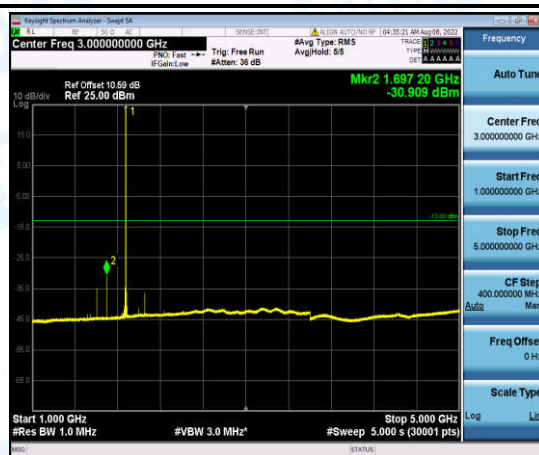
Band2-10MHz-16QAM-18900-1-0-Low-1000-5000--30.91-PASS
