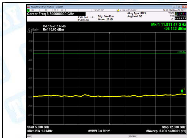
Band2-15MHz-16QAM-19150-1-0-High-5000-12000--56.14-PASS
