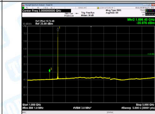
Band2-20MHz-QPSK-19100-1-0-High-1000-5000--35.98-PASS
