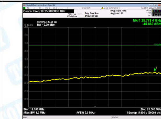
Band2-15MHz-QPSK-18675-1-0-Low-12000-26500--45.86-PASS
