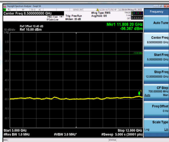
Band4-1.4MHz-16QAM-20175-1-0-Low-5000-12000--56.37-PASS
