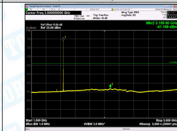
Band2-15MHz-QPSK-18675-1-0-Low-1000-5000--41.17-PASS
