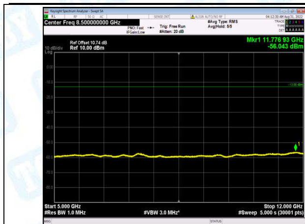
Band2-15MHz-QPSK-19150-1-0-High-5000-12000--56.04-PASS
