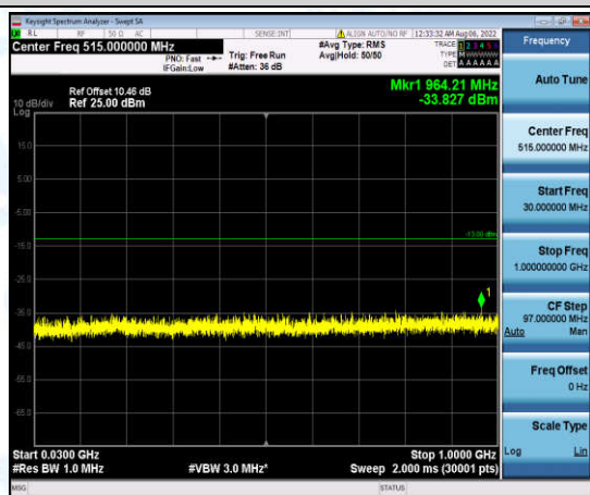
Band4-3MHz-16QAM-19965-1-0-Low-30-1000--33.83-PASS
