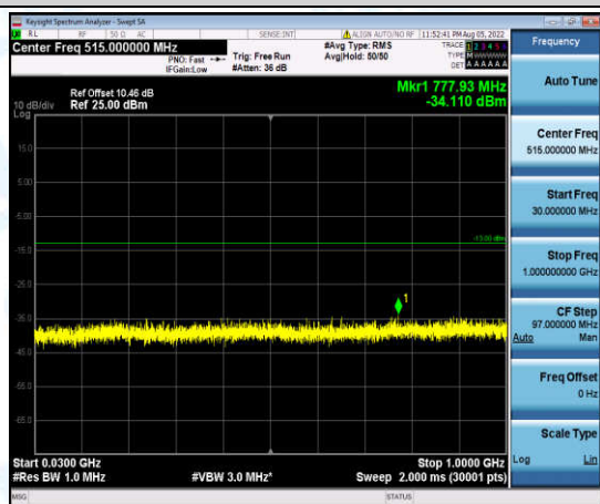
Band4-1.4MHz-16QAM-19957-1-0-Low-30-1000--34.11-PASS
