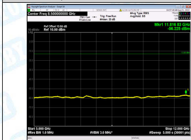
Band2-20MHz-QPSK-18900-1-0-Low-5000-12000--56.23-PASS
