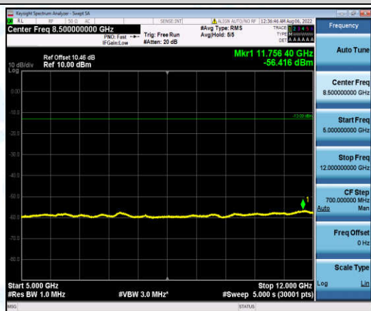
Band4-3MHz-QPSK-20175-1-0-Low-5000-12000--56.42-PASS
