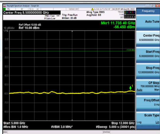
Band2-10MHz-16QAM-18900-1-0-Low-5000-12000--56.45-PASS
