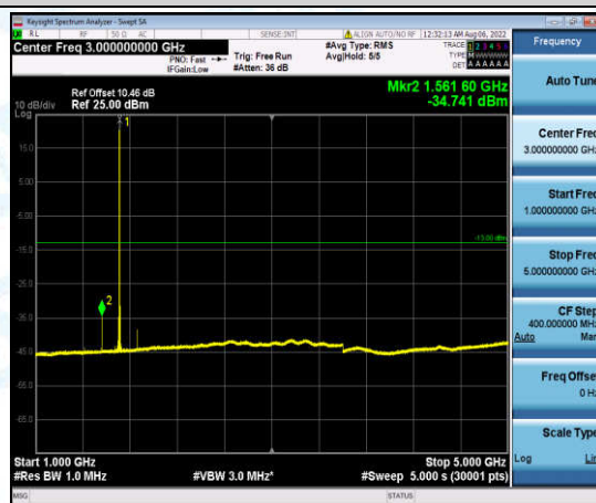
Band4-3MHz-QPSK-19965-1-0-Low-1000-5000--34.74-PASS
