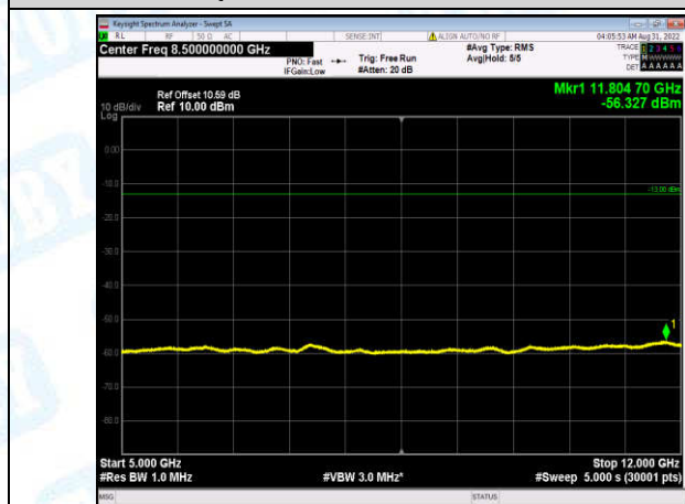
Band2-15MHz-QPSK-18900-1-0-Low-5000-12000--56.33-PASS
