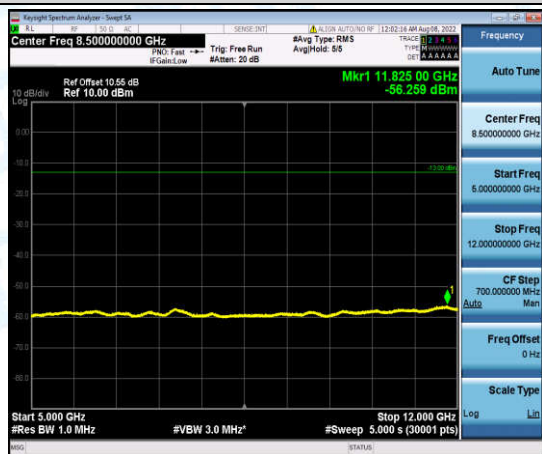
Band2-5MHz-16QAM-18625-1-0-Low-5000-12000--56.26-PASS
