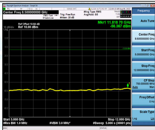
Band2-5MHz-QPSK-18900-1-0-Low-5000-12000--56.37-PASS
