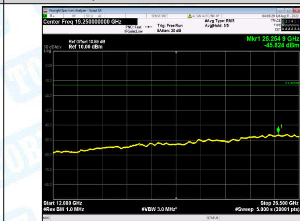
Band2-15MHz-QPSK-18900-1-0-Low-12000-26500--45.82-PASS
