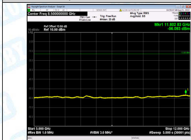
Band2-20MHz-16QAM-18900-1-0-Low-5000-12000--56.09-PASS
