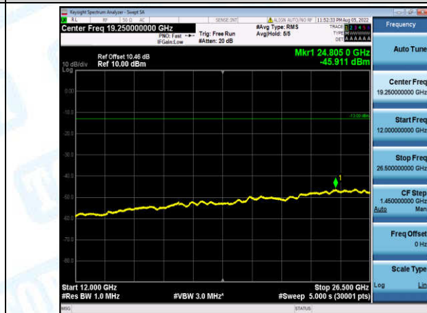
Band4-1.4MHz-QPSK-19957-1-0-Low-12000-26500--45.91-PASS
