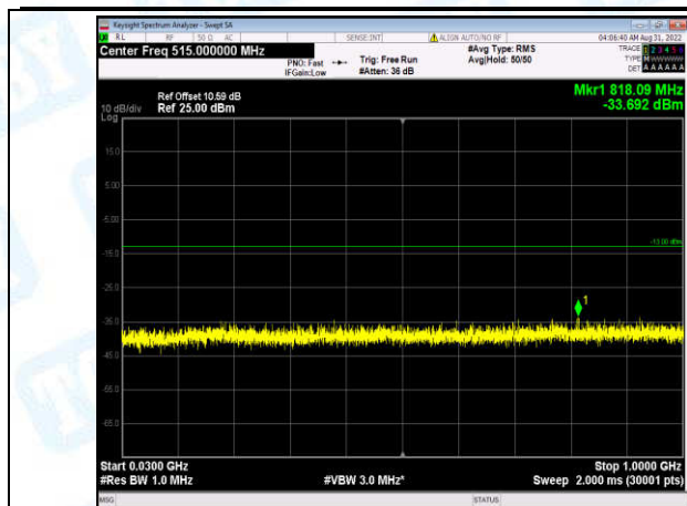
Band2-15MHz-16QAM-18900-1-0-Low-30-1000--33.69-PASS
