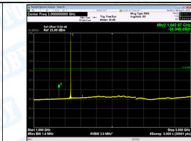
Band2-20MHz-16QAM-18900-1-0-Low-1000-5000--34.05-PASS
