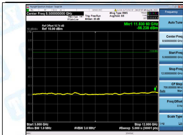
Band2-10MHz-QPSK-19150-1-0-High-5000-12000--56.24-PASS
