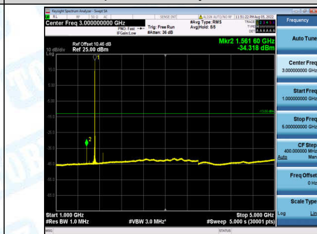
Band4-1.4MHz-QPSK-19957-1-0-Low-1000-5000--34.32-PASS
