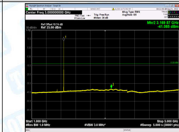
Band2-15MHz-QPSK-19150-1-0-High-1000-5000--41.09-PASS
