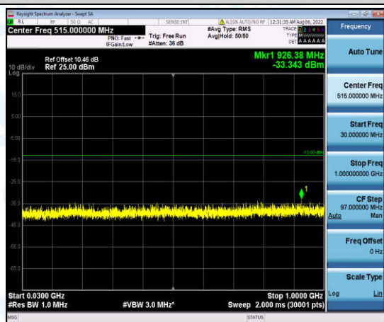
Band4-3MHz-QPSK-19965-1-0-Low-30-1000--33.34-PASS
