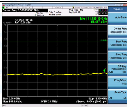
Band4-1.4MHz-QPSK-20393-1-0-High-5000-12000--56.46-PASS
