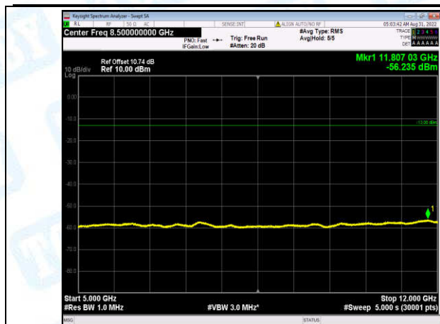
Band2-20MHz-16QAM-19100-1-0-High-5000-12000--56.24-PASS
