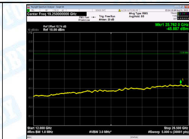
Band2-20MHz-16QAM-19100-1-0-High-12000-26500--45.89-PASS
