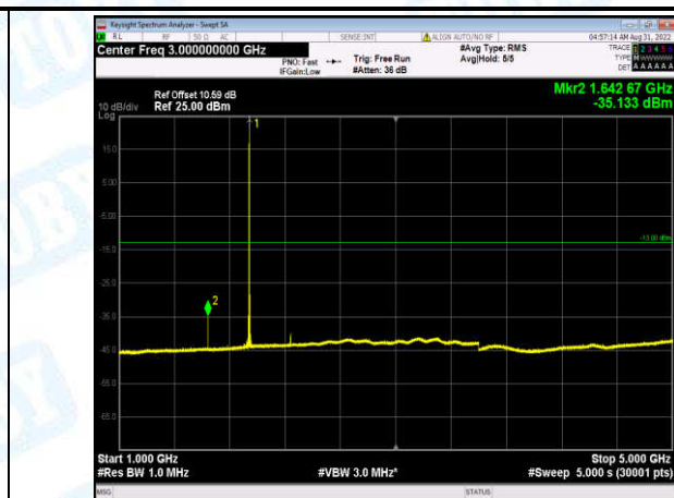
Band2-20MHz-QPSK-18900-1-0-Low-1000-5000--35.13-PASS
