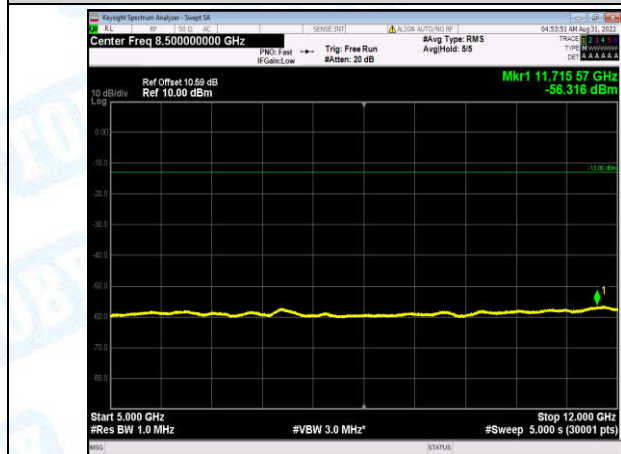
Band2-20MHz-QPSK-18700-1-0-Low-5000-12000--56.32-PASS
