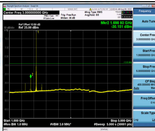
Band2-5MHz-QPSK-18900-1-0-Low-1000-5000--30.15-PASS
