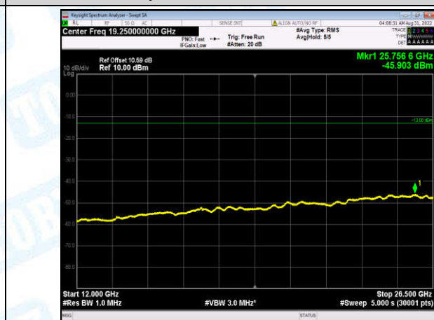
Band2-15MHz-16QAM-18900-1-0-Low-12000-26500--45.9-PASS
