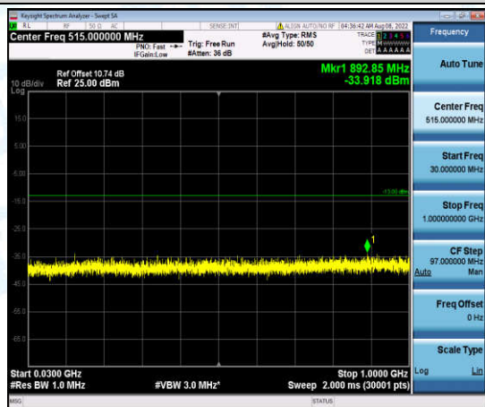
Band2-10MHz-QPSK-19150-1-0-High-30-1000--33.92-PASS
