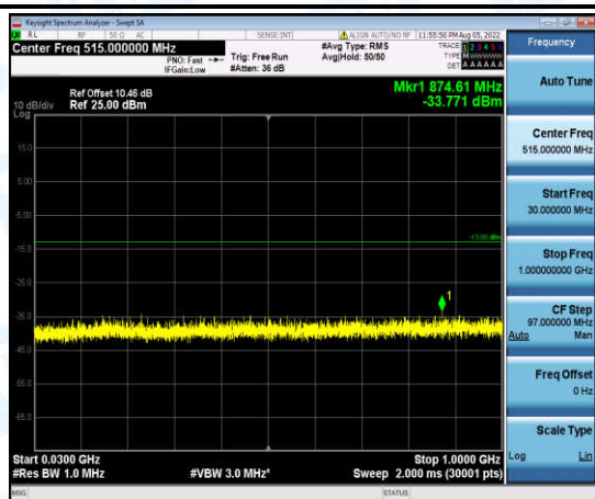
Band4-1.4MHz-QPSK-20175-1-0-Low-30-1000--33.77-PASS
