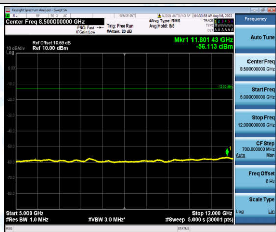
Band2-10MHz-QPSK-18900-1-0-Low-5000-12000--56.11-PASS
