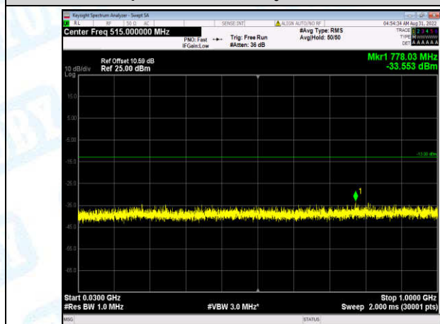
Band2-20MHz-16QAM-18700-1-0-Low-30-1000--33.55-PASS
