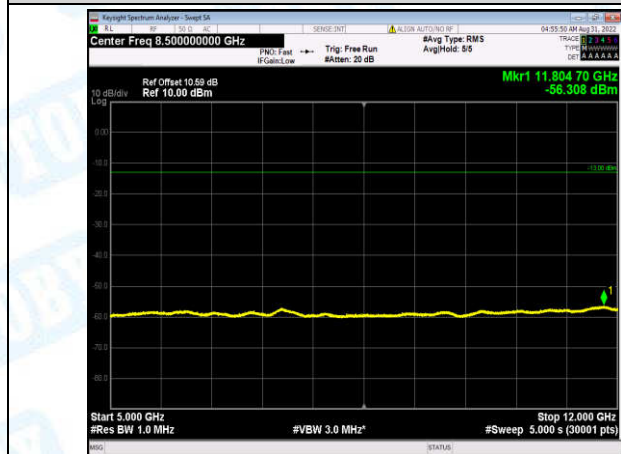
Band2-20MHz-16QAM-18700-1-0-Low-5000-12000--56.31-PASS
