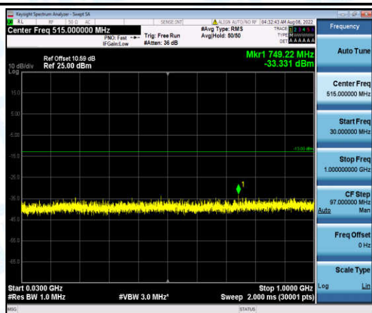
Band2-10MHz-QPSK-18900-1-0-Low-30-1000--33.33-PASS
