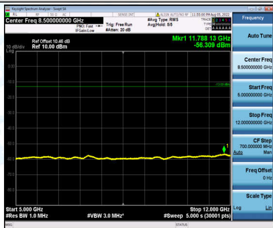
Band4-1.4MHz-16QAM-19957-1-0-Low-5000-12000--56.31-PASS
