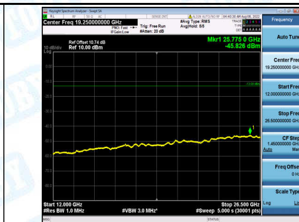
Band2-10MHz-16QAM-19150-1-0-High-12000-26500--45.83-PASS
