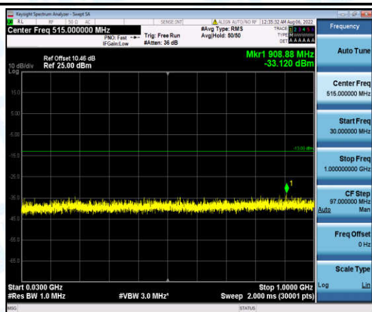
Band4-3MHz-QPSK-20175-1-0-Low-30-1000--33.12-PASS
