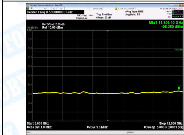
Band2-15MHz-16QAM-18675-1-0-Low-5000-12000--56.39-PASS
