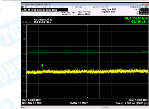
Band2-20MHz-16QAM-19100-1-0-High-30-1000--33.12-PASS
