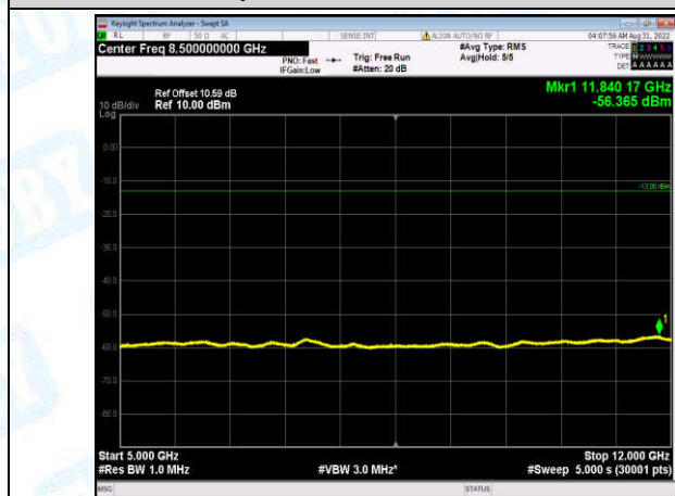
Band2-15MHz-16QAM-18900-1-0-Low-5000-12000--56.37-PASS
