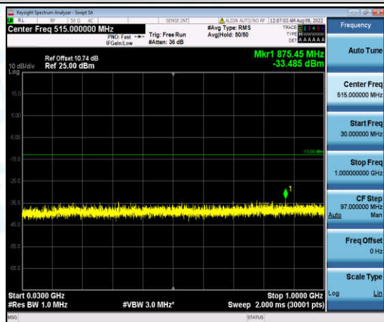
Band2-5MHz-QPSK-19175-1-0-High-30-1000--33.49-PASS
