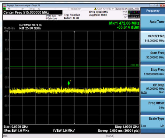
Band2-5MHz-16QAM-19175-1-0-High-30-1000--33.61-PASS
