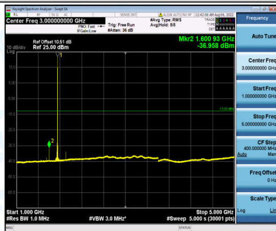
Band4-3MHz-16QAM-20385-1-0-High-1000-5000--36.96-PASS
