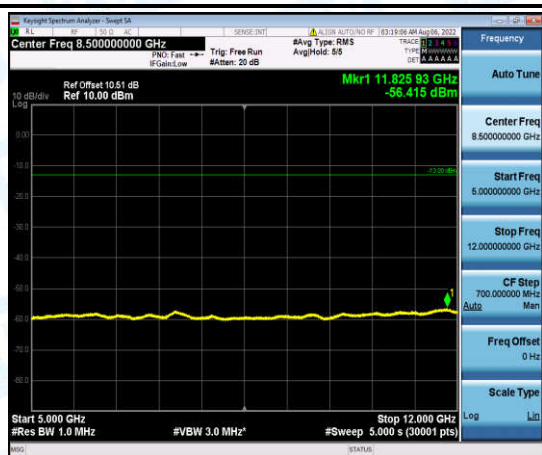
Band4-15MHz-QPSK-20325-1-0-High-5000-12000--56.42-PASS
