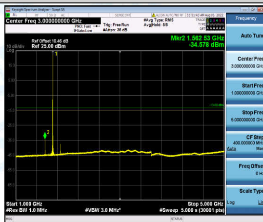
Band4-20MHz-16QAM-20050-1-0-Low-1000-5000--34.58-PASS
