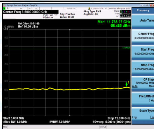
Band4-20MHz-16QAM-20300-1-0-High-5000-12000--56.47-PASS
