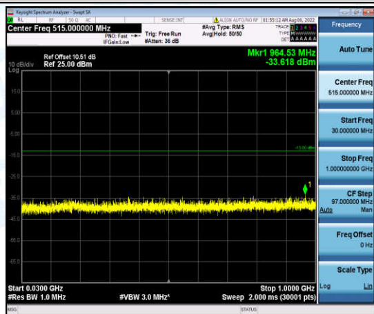
Band4-5MHz-16QAM-20375-1-0-High-30-1000--33.62-PASS
