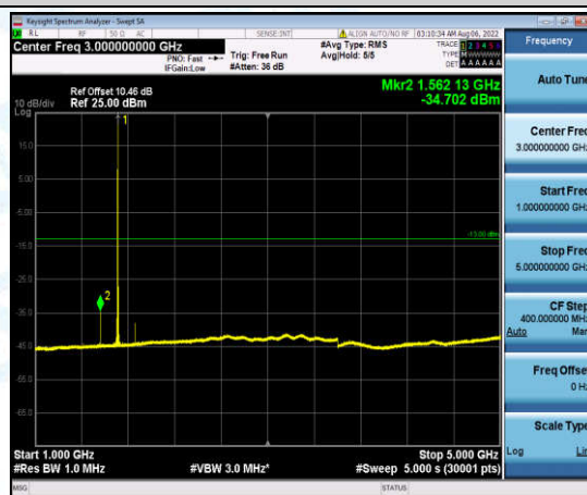
Band4-15MHz-QPSK-20025-1-0-Low-1000-5000--34.7-PASS
