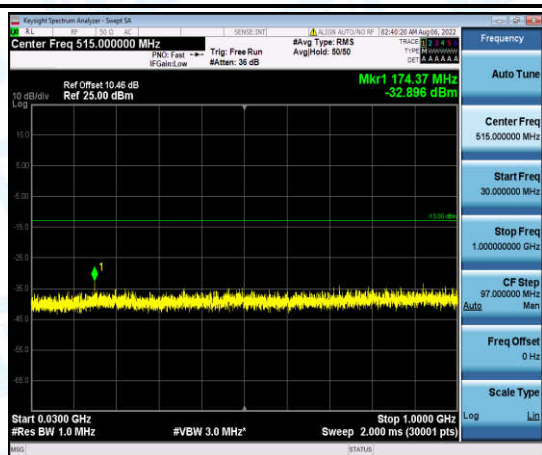
Band4-10MHz-16QAM-20175-1-0-Low-30-1000--32.9-PASS
