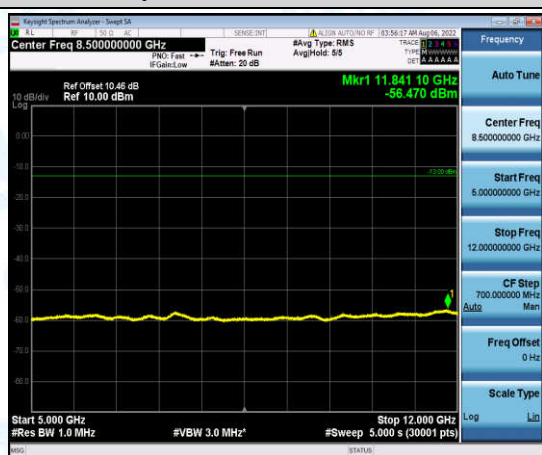
Band4-20MHz-16QAM-20175-1-0-Low-5000-12000--56.47-PASS
