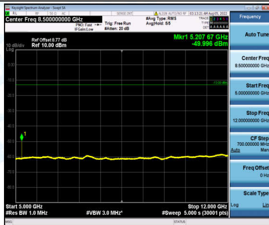
Band5-1.4MHz-QPSK-20407-1-0-Low-5000-12000--50-PASS
