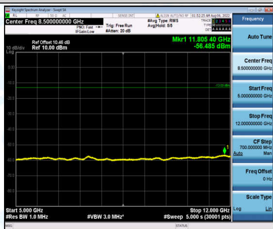
Band4-5MHz-16QAM-20175-1-0-Low-5000-12000--56.49-PASS
