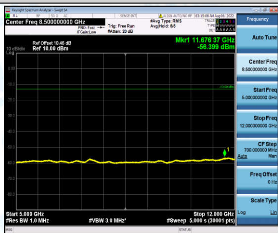
Band4-15MHz-QPSK-20175-1-0-Low-5000-12000--56.4-PASS
