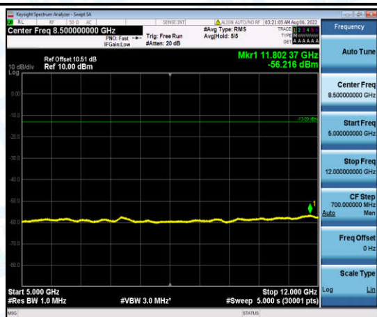
Band4-15MHz-16QAM-20325-1-0-High-5000-12000--56.22-PASS
