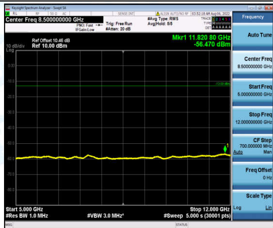
Band4-20MHz-16QAM-20050-1-0-Low-5000-12000--56.47-PASS
