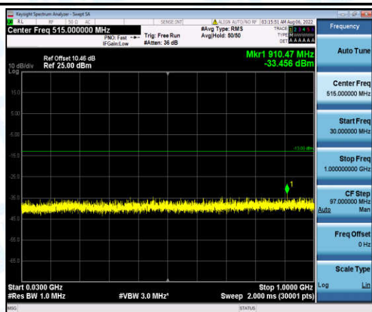
Band4-15MHz-16QAM-20175-1-0-Low-30-1000--33.46-PASS
