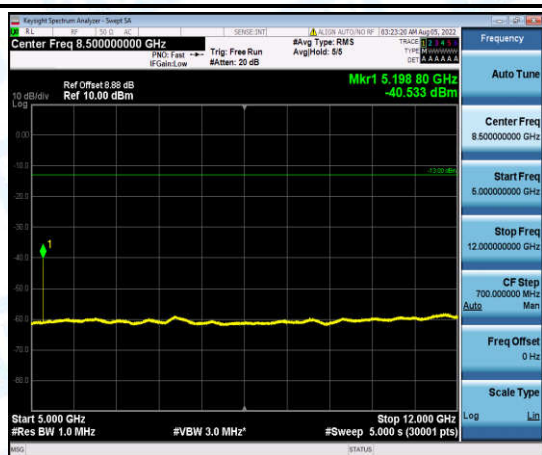
Band5-1.4MHz-16QAM-20643-1-0-High-5000-12000--40.53-PASS
