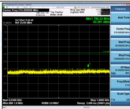
Band4-20MHz-QPSK-20050-1-0-Low-30-1000--33.29-PASS
