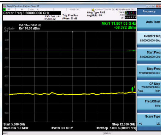
Band4-10MHz-16QAM-20350-1-0-High-5000-12000--56.37-PASS
