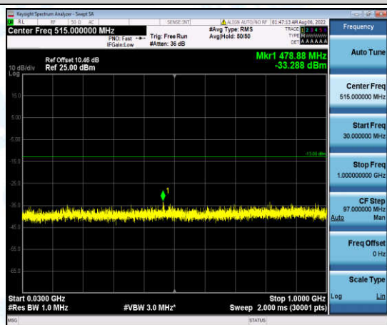
Band4-5MHz-16QAM-19975-1-0-Low-30-1000--33.29-PASS
