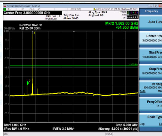
Band4-10MHz-QPSK-20000-1-0-Low-1000-5000--34.65-PASS
