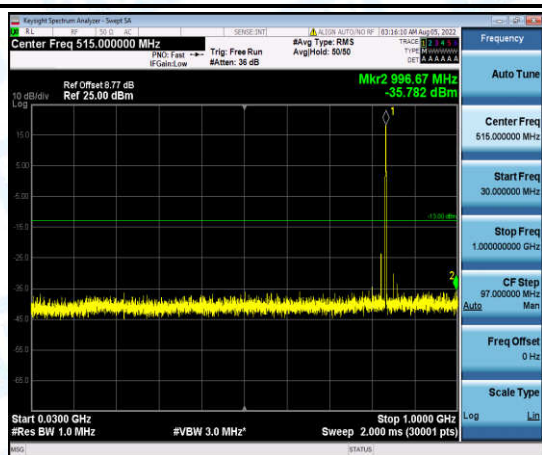
Band5-1.4MHz-QPSK-20525-1-0-Low-30-1000--35.78-PASS
