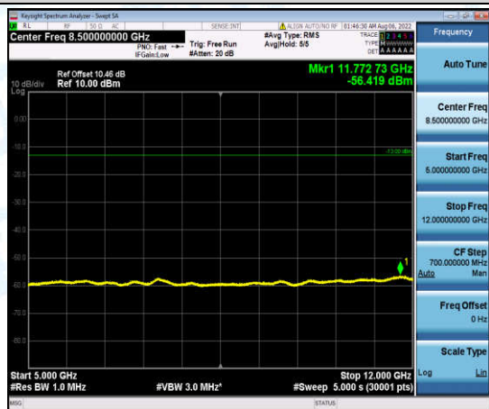
Band4-5MHz-QPSK-19975-1-0-Low-5000-12000--56.42-PASS
