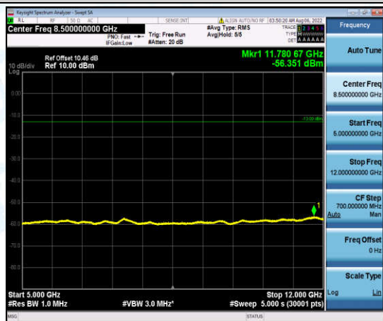
Band4-20MHz-QPSK-20050-1-0-Low-5000-12000--56.35-PASS
