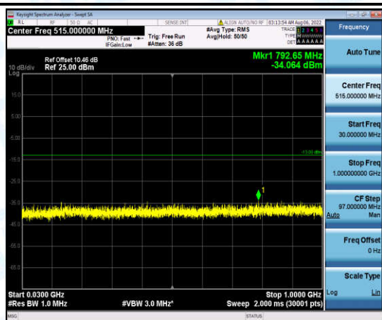
Band4-15MHz-QPSK-20175-1-0-Low-30-1000--34.06-PASS
