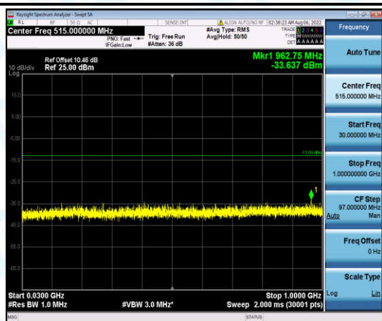
Band4-10MHz-QPSK-20175-1-0-Low-30-1000--33.64-PASS
