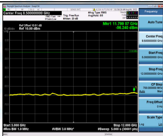
Band4-5MHz-16QAM-20375-1-0-High-5000-12000--56.24-PASS
