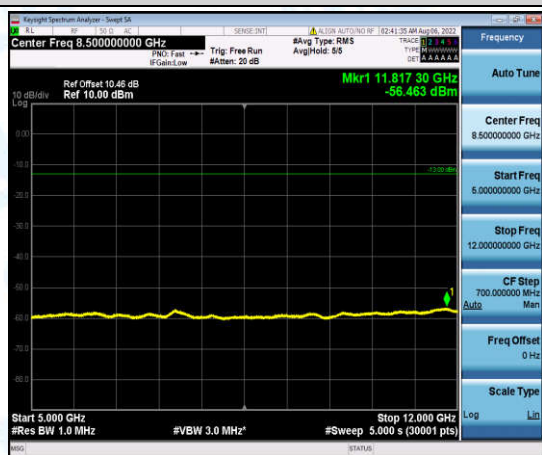
Band4-10MHz-16QAM-20175-1-0-Low-5000-12000--56.46-PASS
