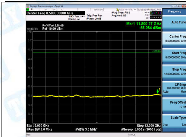
Band5-1.4MHz-QPSK-20643-1-0-High-5000-12000--58.08-PASS
