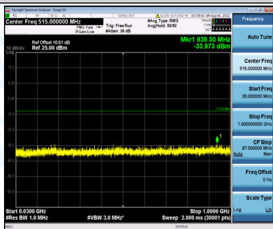
Band4-20MHz-16QAM-20300-1-0-High-30-1000--33.97-PASS
