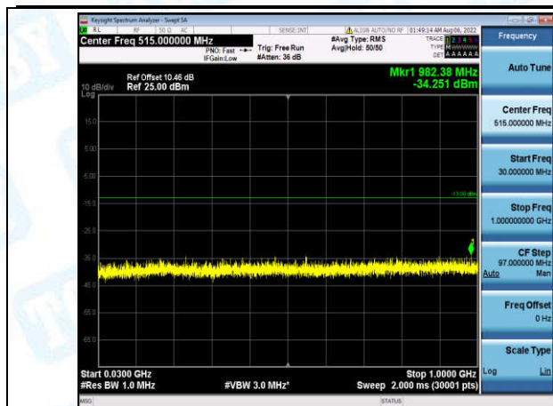
Band4-5MHz-QPSK-20175-1-0-Low-30-1000--34.25-PASS
