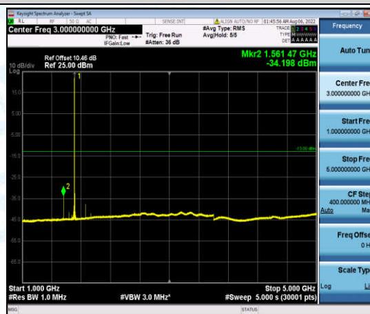
Band4-5MHz-QPSK-19975-1-0-Low-1000-5000--34.2-PASS
