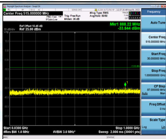
Band4-3MHz-16QAM-20175-1-0-Low-30-1000--33.84-PASS
