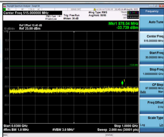
Band4-5MHz-QPSK-19975-1-0-Low-30-1000--33.74-PASS
