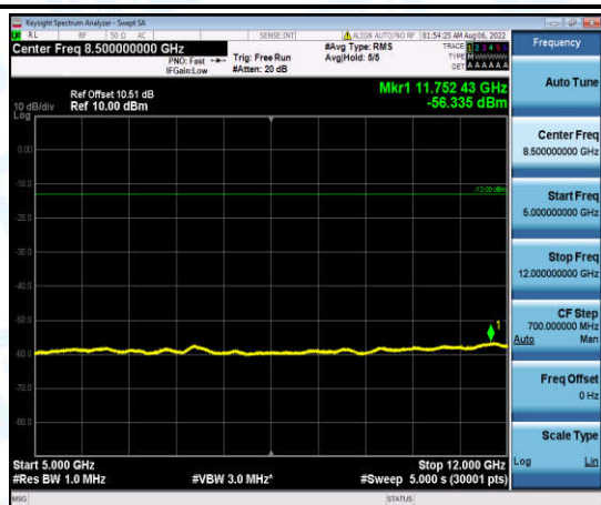
Band4-5MHz-QPSK-20375-1-0-High-5000-12000--56.34-PASS
