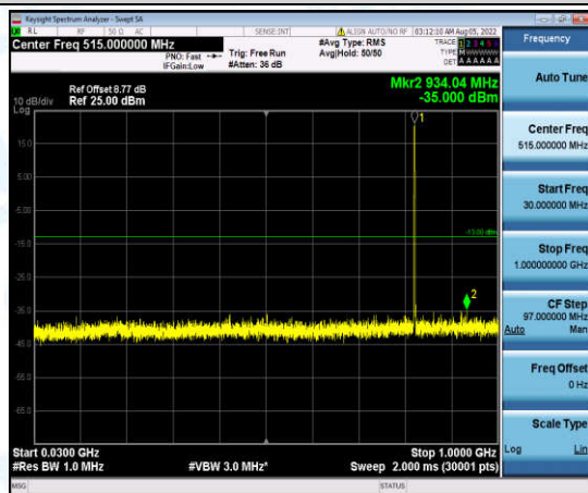
Band5-1.4MHz-QPSK-20407-1-0-Low-30-1000--35-PASS
