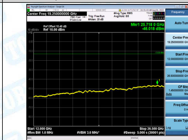
Band4-5MHz-QPSK-20175-1-0-Low-12000-26500--46.02-PASS
