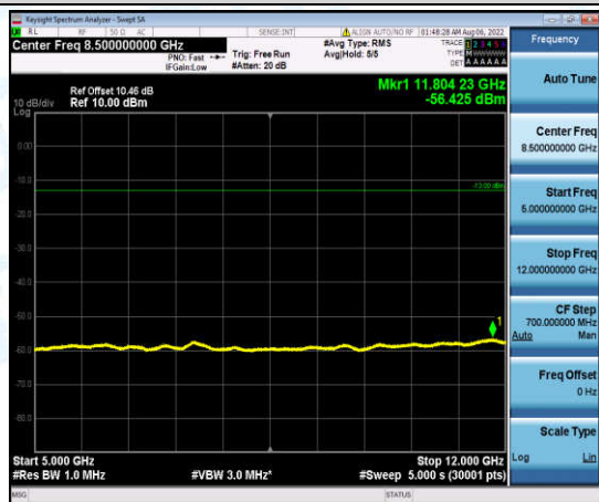
Band4-5MHz-16QAM-19975-1-0-Low-5000-12000--56.43-PASS
