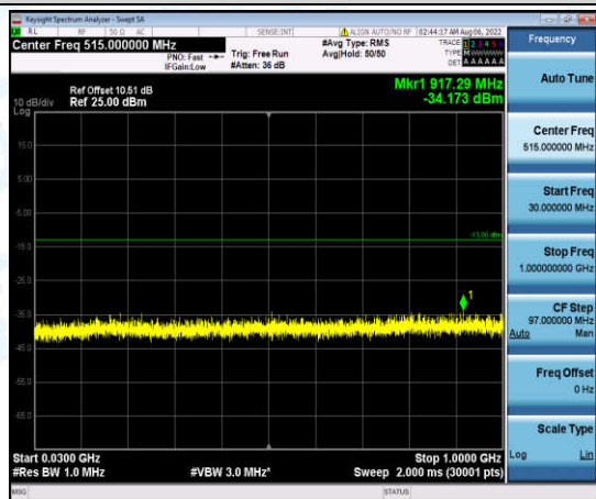
Band4-10MHz-16QAM-20350-1-0-High-30-1000--34.17-PASS
