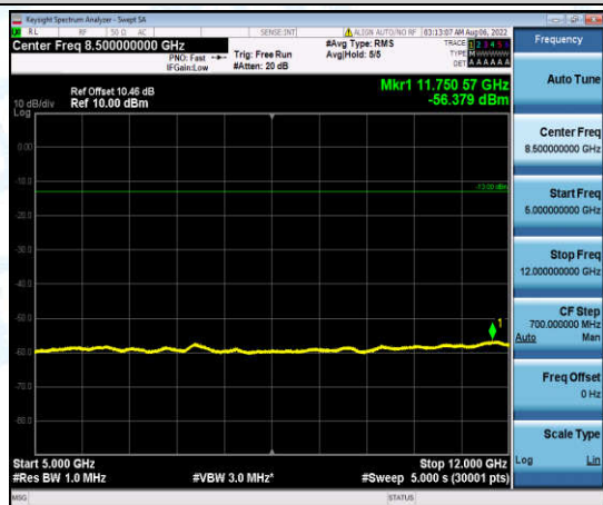
Band4-15MHz-16QAM-20025-1-0-Low-5000-12000--56.38-PASS
