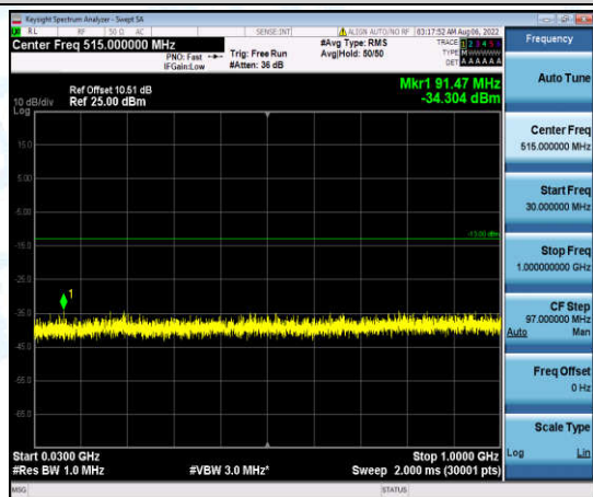
Band4-15MHz-QPSK-20325-1-0-High-30-1000--34.3-PASS
