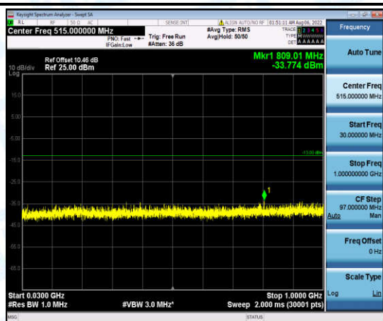
Band4-5MHz-16QAM-20175-1-0-Low-30-1000--33.77-PASS
