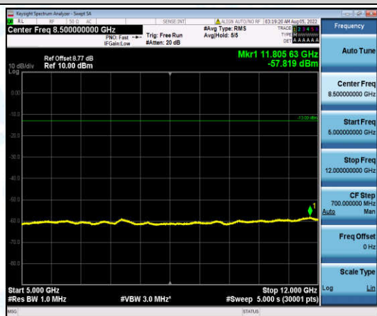
Band5-1.4MHz-16QAM-20525-1-0-Low-5000-12000--57.82-PASS
