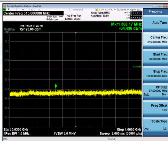
Band4-10MHz-QPSK-20000-1-0-Low-30-1000--34.44-PASS
