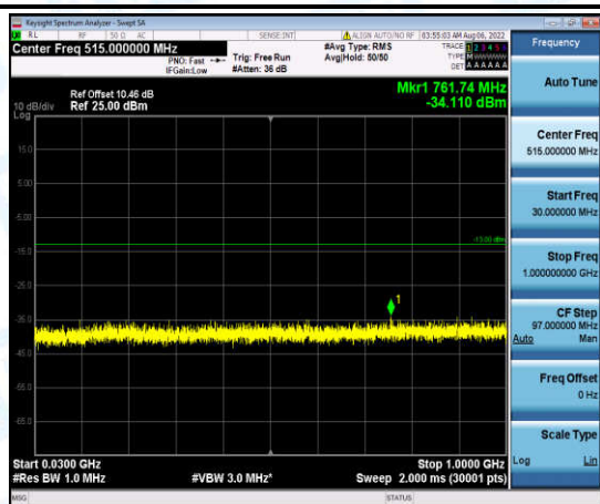
Band4-20MHz-16QAM-20175-1-0-Low-30-1000--34.11-PASS
