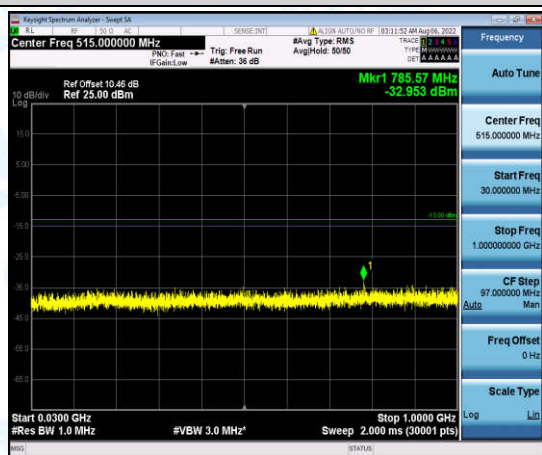
Band4-15MHz-16QAM-20025-1-0-Low-30-1000--32.95-PASS
