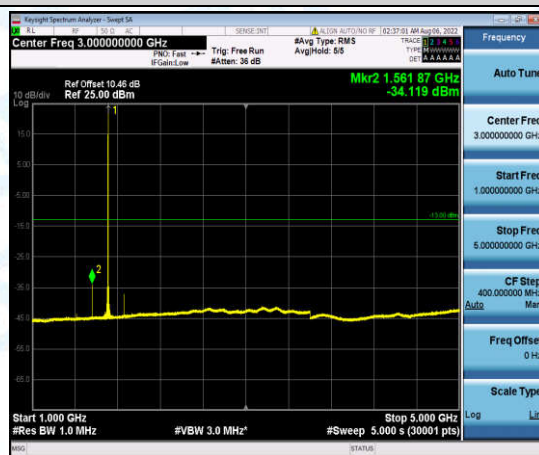
Band4-10MHz-16QAM-20000-1-0-Low-1000-5000--34.12-PASS
