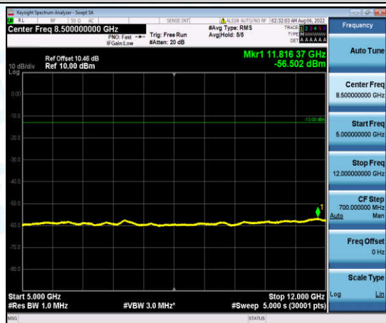
Band4-10MHz-QPSK-20000-1-0-Low-5000-12000--56.5-PASS
