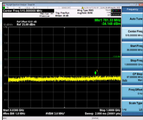
Band4-3MHz-16QAM-20385-1-0-High-30-1000--34.15-PASS
