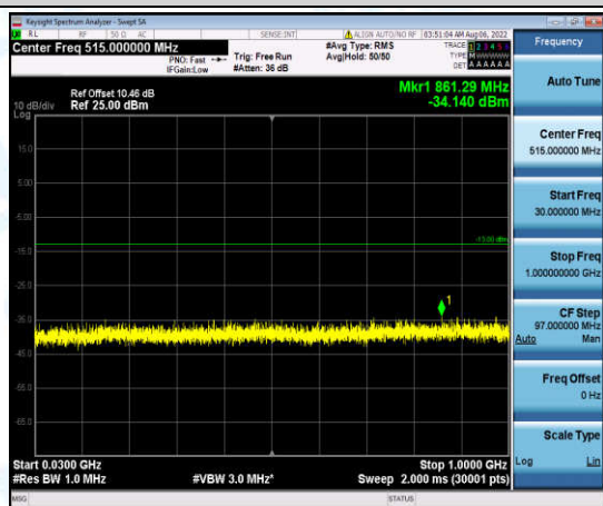
Band4-20MHz-16QAM-20050-1-0-Low-30-1000--34.14-PASS
