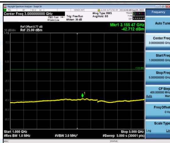
Band5-1.4MHz-QPSK-20525-1-0-Low-1000-5000--42.71-PASS
