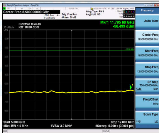
Band4-15MHz-QPSK-20025-1-0-Low-5000-12000--56.5-PASS
