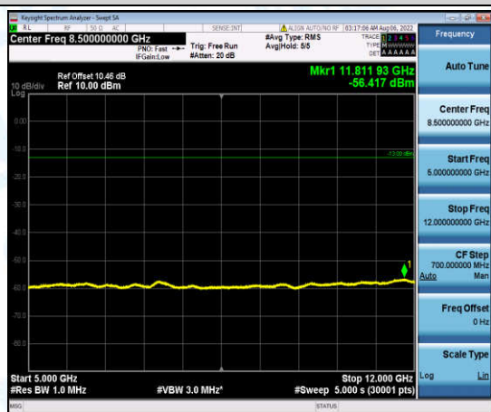
Band4-15MHz-16QAM-20175-1-0-Low-5000-12000--56.42-PASS
