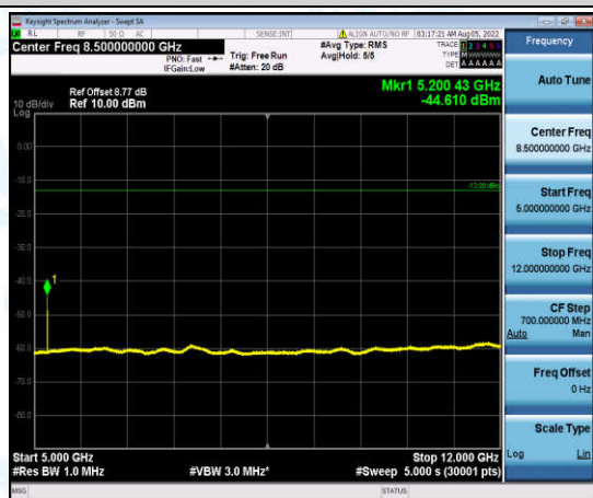
Band5-1.4MHz-QPSK-20525-1-0-Low-5000-12000--44.61-PASS
