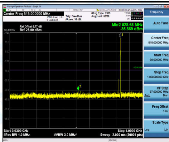
Band5-1.4MHz-16QAM-20525-1-0-Low-30-1000--35.87-PASS
