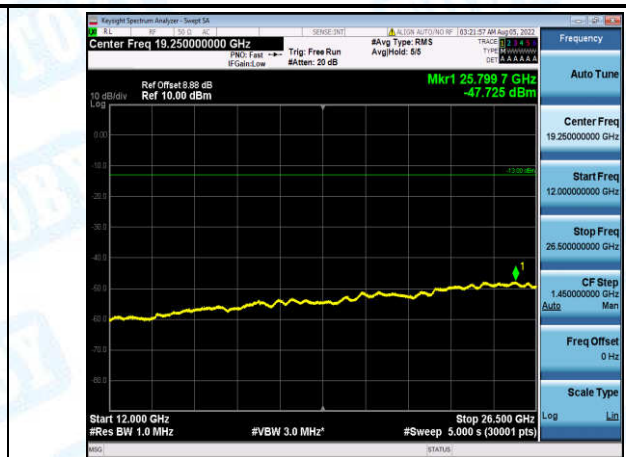
Band5-1.4MHz-QPSK-20643-1-0-High-12000-26500--47.73-PASS
