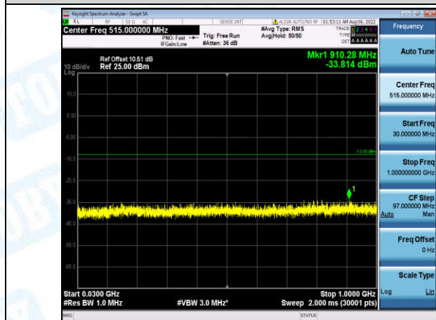
Band4-5MHz-QPSK-20375-1-0-High-30-1000--33.81-PASS
