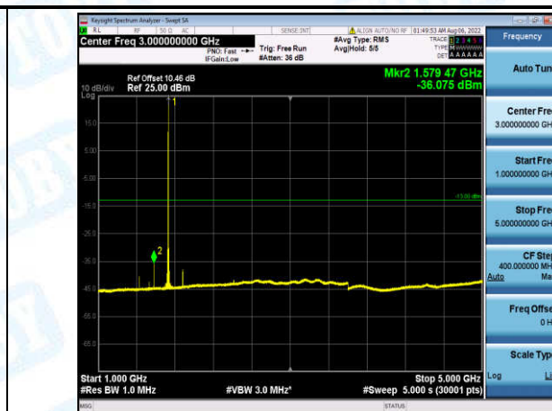
Band4-5MHz-QPSK-20175-1-0-Low-1000-5000--36.08-PASS
