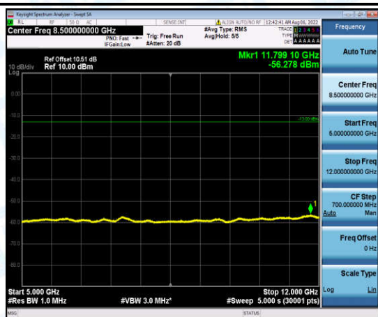
Band4-3MHz-16QAM-20385-1-0-High-5000-12000--56.28-PASS
