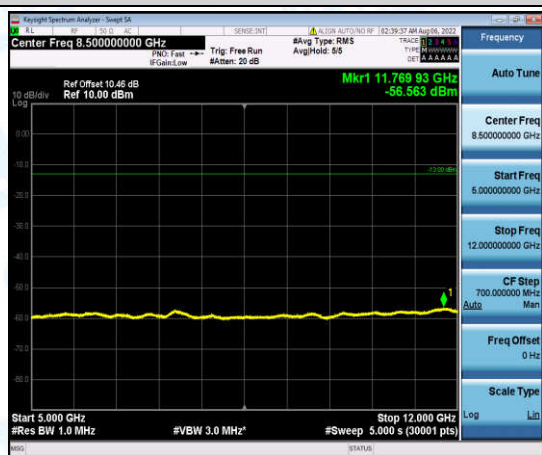
Band4-10MHz-QPSK-20175-1-0-Low-5000-12000--56.56-PASS
