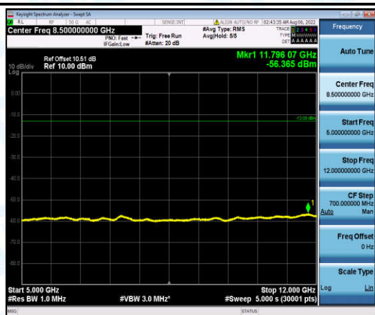
Band4-10MHz-QPSK-20350-1-0-High-5000-12000--56.37-PASS
