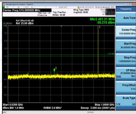
Band5-1.4MHz-16QAM-20643-1-0-High-30-1000--35.22-PASS
