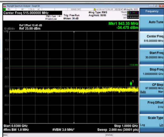
Band4-10MHz-16QAM-20000-1-0-Low-30-1000--34.48-PASS
