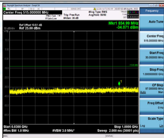
Band4-20MHz-QPSK-20300-1-0-High-30-1000--34.07-PASS
