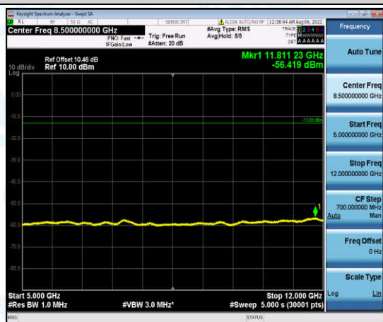
Band4-3MHz-16QAM-20175-1-0-Low-5000-12000--56.42-PASS
