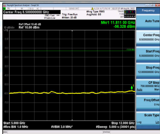
Band4-10MHz-16QAM-20000-1-0-Low-5000-12000--56.33-PASS
