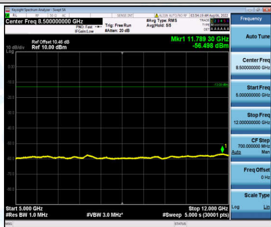
Band4-20MHz-QPSK-20175-1-0-Low-5000-12000--56.5-PASS
