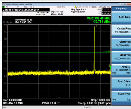
Band5-1.4MHz-QPSK-20643-1-0-High-30-1000--35.78-PASS
