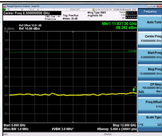
Band4-20MHz-QPSK-20300-1-0-High-5000-12000--56.36-PASS
