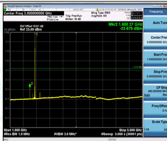
Band4-20MHz-16QAM-20300-1-0-High-1000-5000--33.68-PASS
