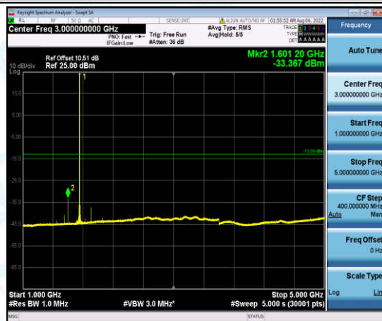
Band4-5MHz-16QAM-20375-1-0-High-1000-5000--33.37-PASS
