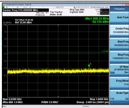
Band4-15MHz-QPSK-20025-1-0-Low-30-1000--34.12-PASS
