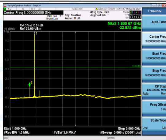
Band4-10MHz-16QAM-20350-1-0-High-1000-5000--33.93-PASS
