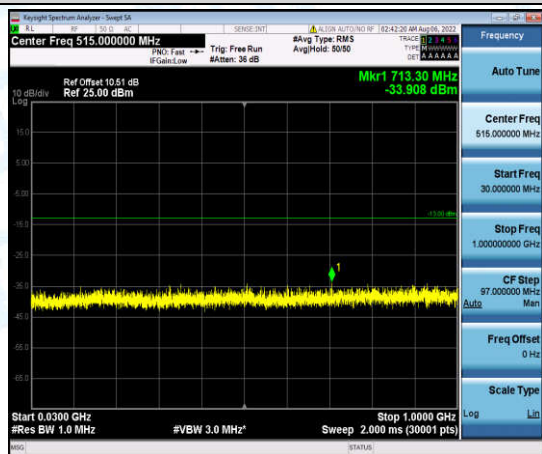
Band4-10MHz-QPSK-20350-1-0-High-30-1000--33.91-PASS
