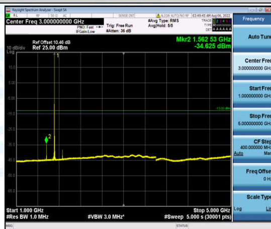
Band4-20MHz-QPSK-20050-1-0-Low-1000-5000--34.63-PASS
