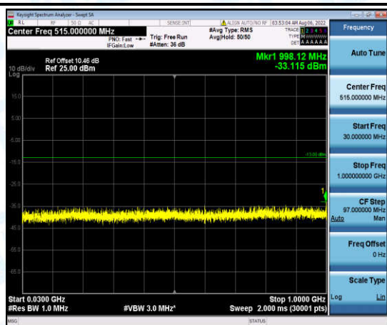
Band4-20MHz-QPSK-20175-1-0-Low-30-1000--33.12-PASS
