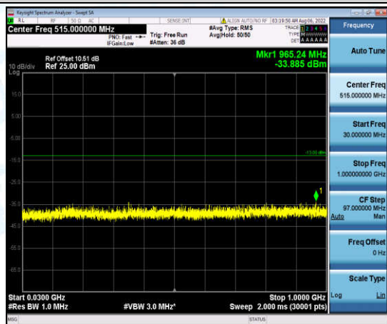
Band4-15MHz-16QAM-20325-1-0-High-30-1000--33.89-PASS
