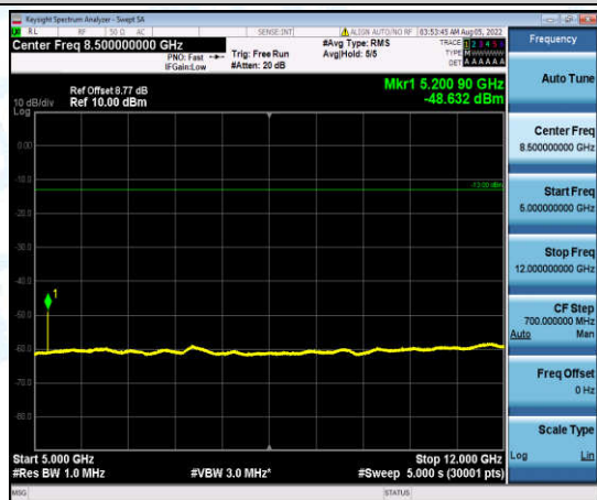
Band5-3MHz-QPSK-20415-1-0-Low-5000-12000--48.63-PASS
