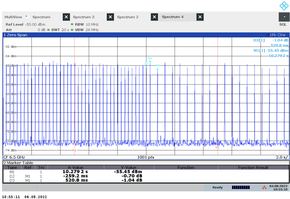
Plot 14: Emissions of the EUT, only at the beginning with associated receiver (EUT3)
