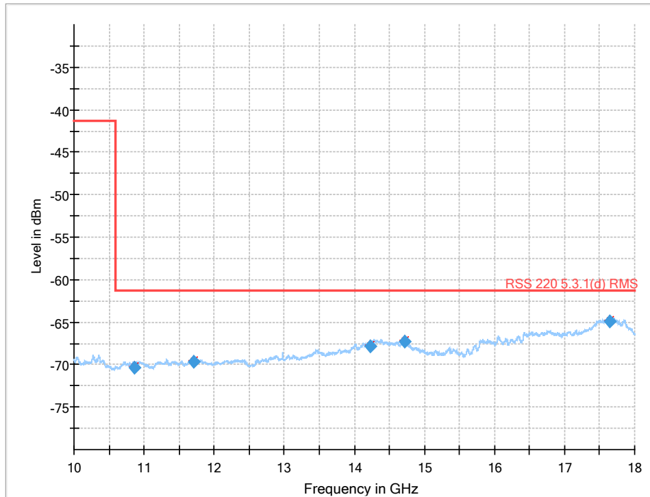
Plot 9: 10 GHz to 18 GHz (EUT2)
