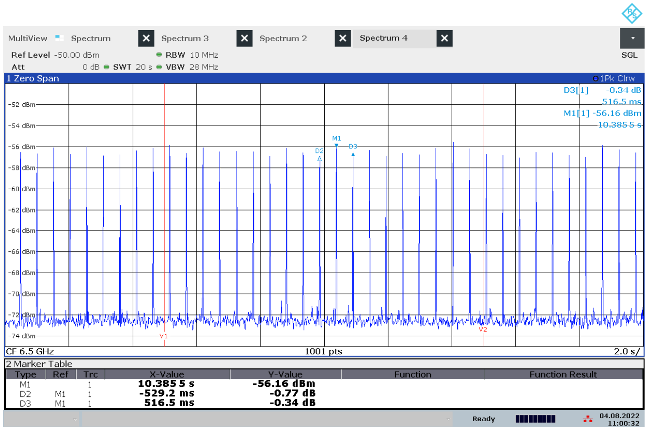
Plot 15: Emissions of EUT without associated receiver (for comparison) (EUT3)
