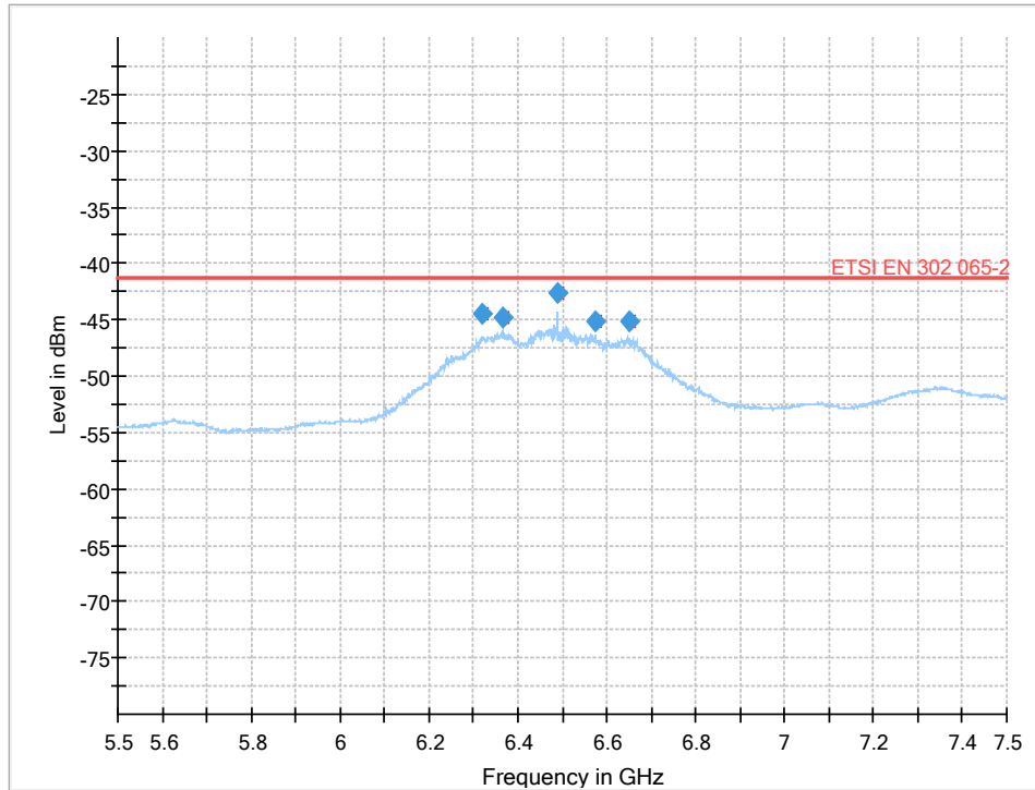
Plot 2: Fundamental emission: RMS (EUT1)
