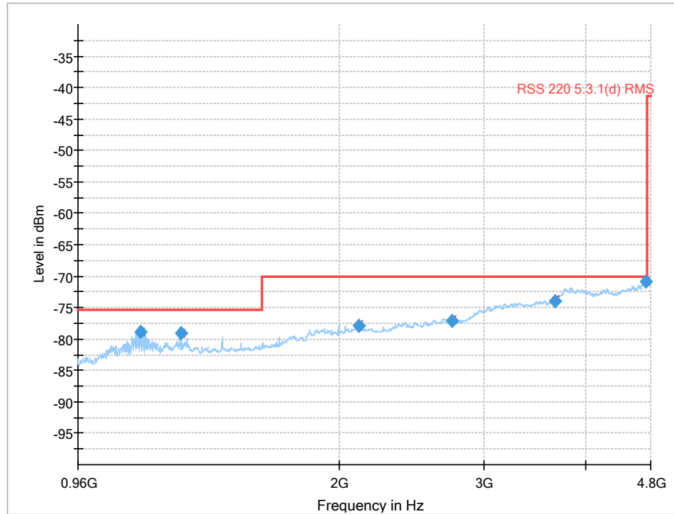
Plot 7: 960 MHz to 4.8 GHz (Limit acc. to RSS-220 5.3.1(d)) (EUT2)
