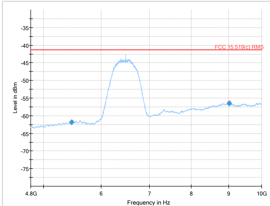
Plot 8: 4.8 GHz to 10 GHz (EUT2)
