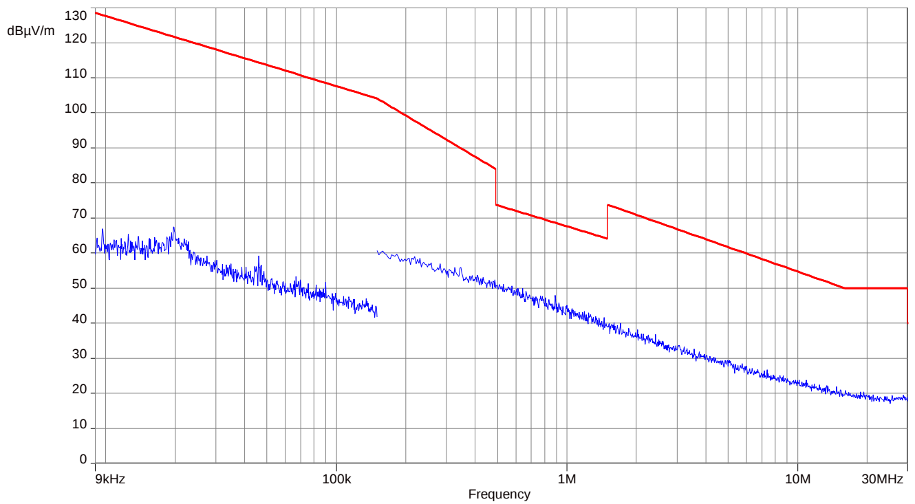
Plot 4: 9 kHz to 30 MHz (EUT2)
