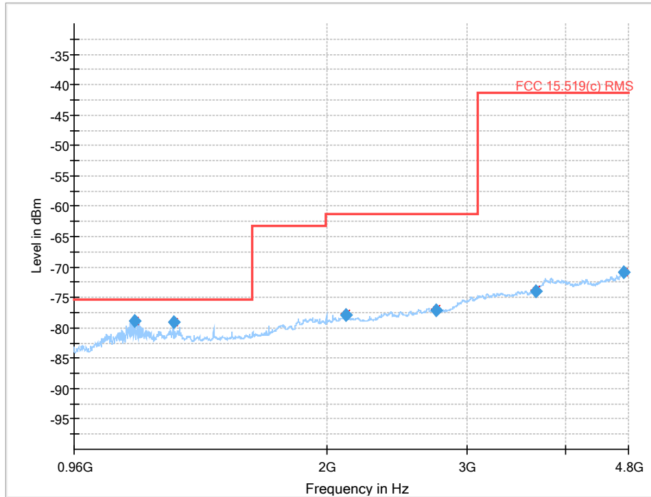
Plot 6: 960 MHz to 4.8 GHz (Limit acc. to §15.519 (c)) (EUT2)
