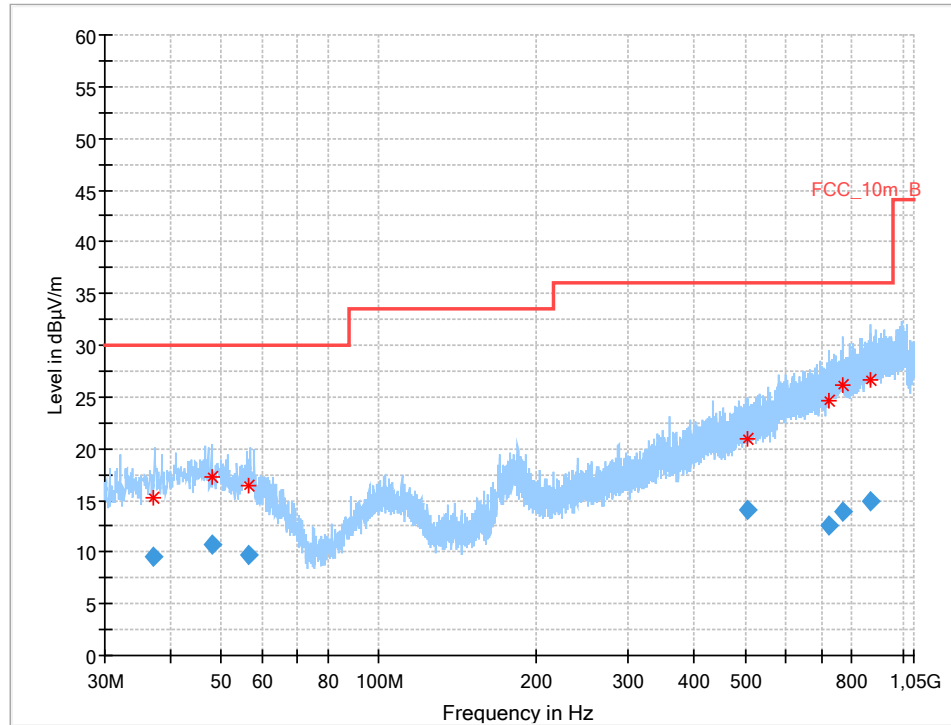
Plot 5: 30 MHz to 1 GHz (EUT2)
