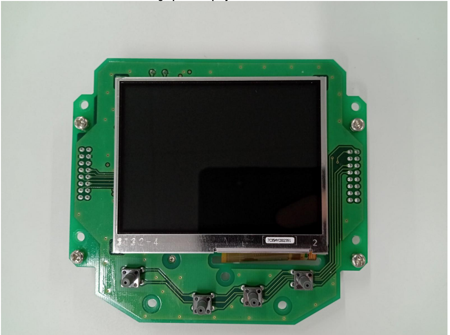
Photograph of Display Board: Screen side
