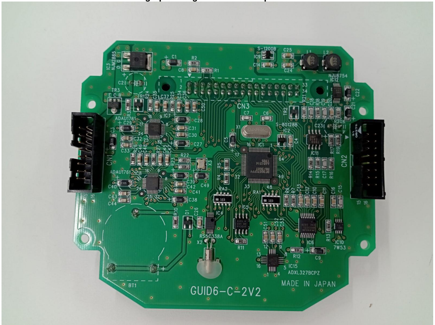
Photograph of Digital Board: Component Side
