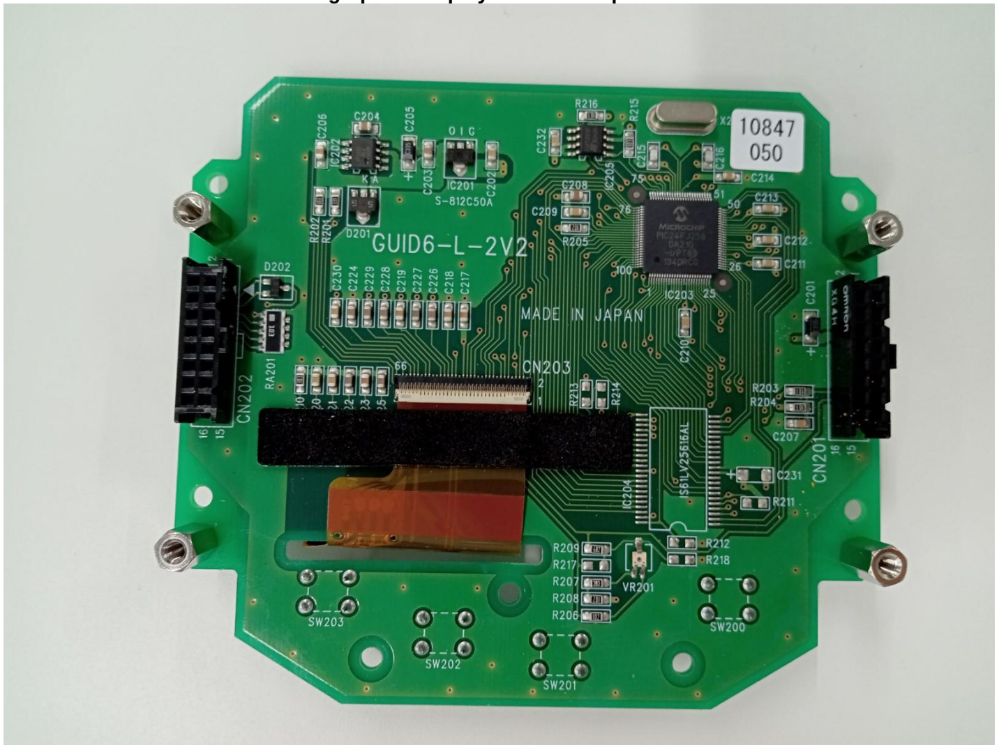
Photograph of Display Board: Component Side
