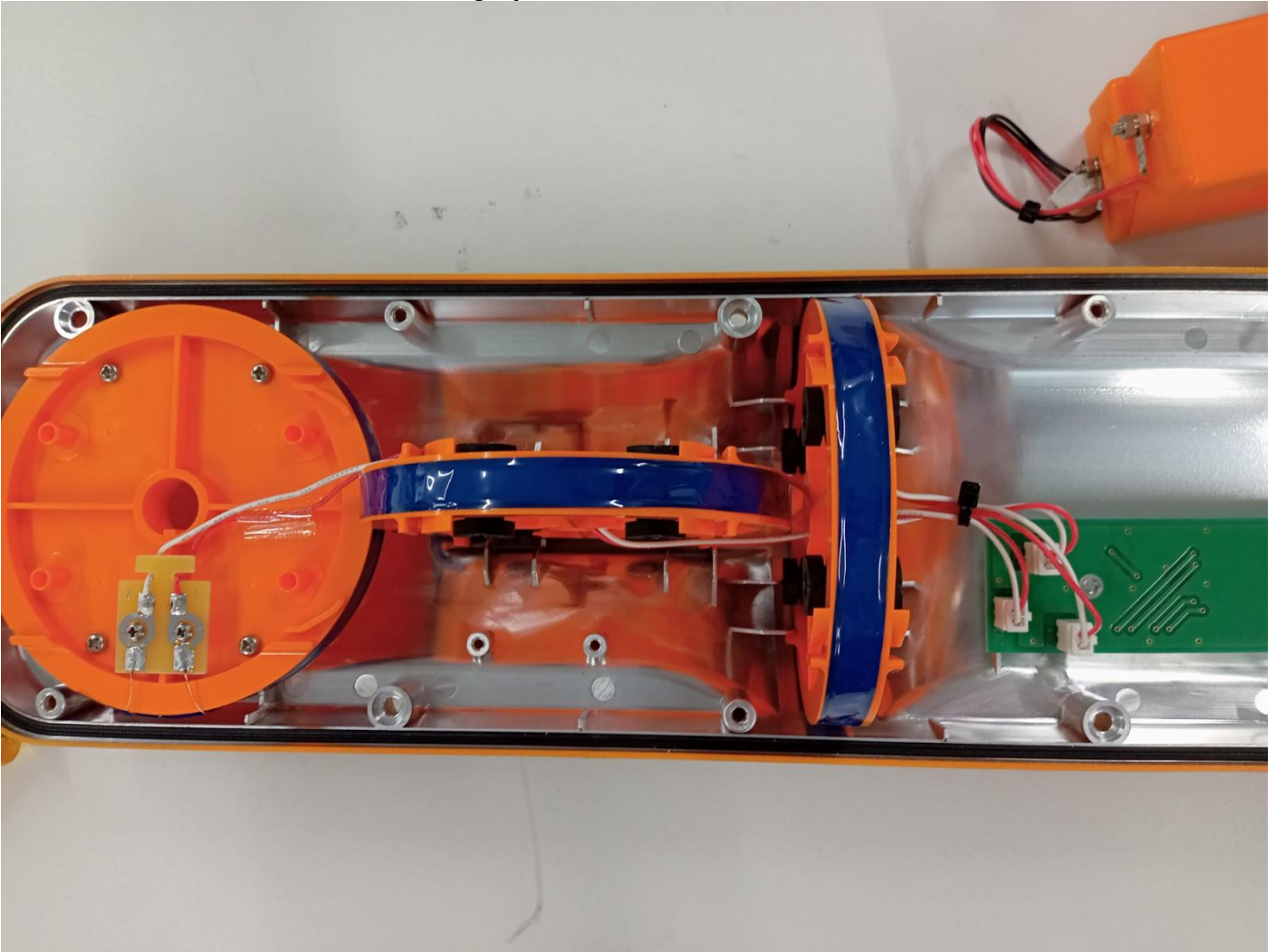
Photographs of EUT; covers removed
