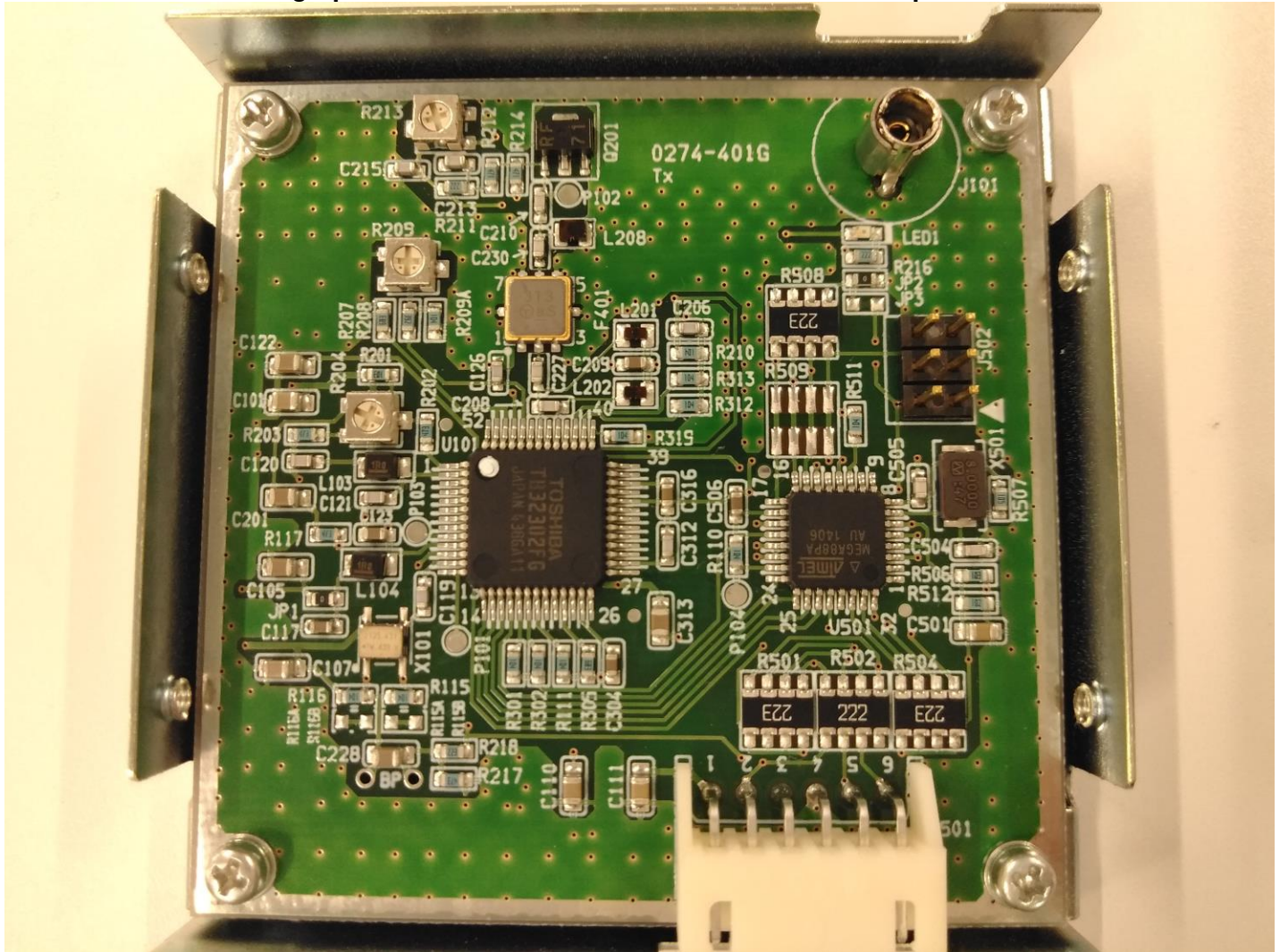
Photograph of RF Board with 460 MHz transmitter: Component Side
