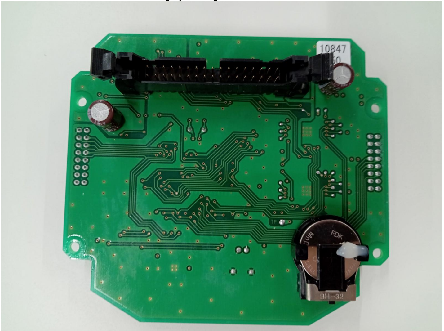
Photograph of Digital Board: Foil Side
