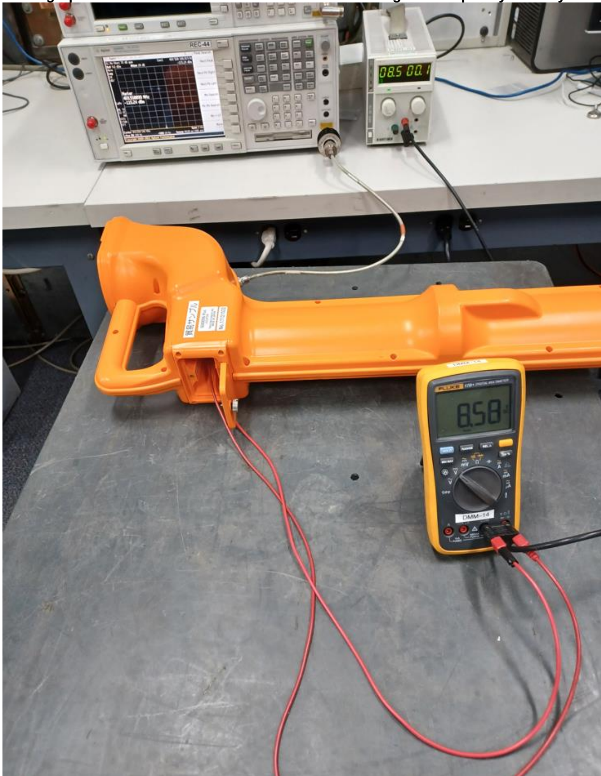
Photograph of Antenna Conducted Emissions and Voltage vs Frequency stability Test
