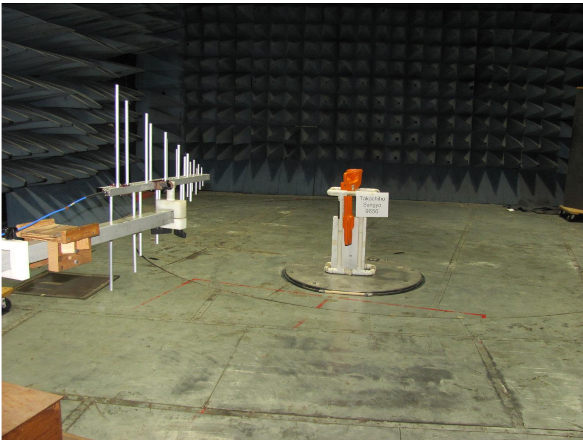
The EUT was taped to a PVC stand to change the axis of rotation.
