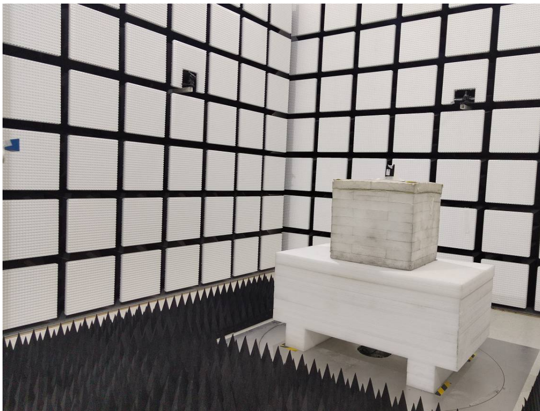
Radiated Emission 26.5-40GHz
