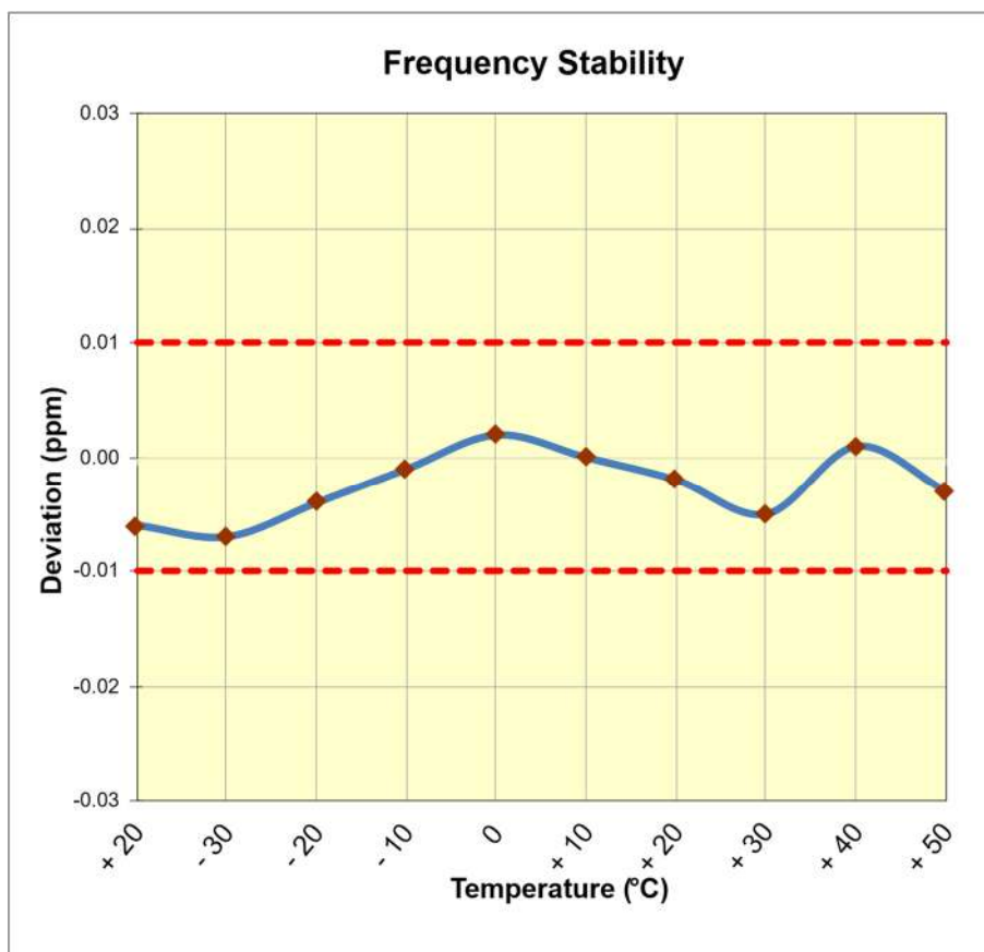
Figure 7-3. Frequency Stability Plot
