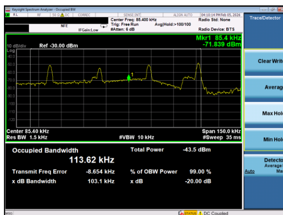
Figure 1-1 WPT Occupied Bandwidth
