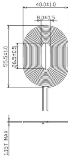
TOP COIL : Smartbonding Litz WIRE 0.08*105P - 15Ts
