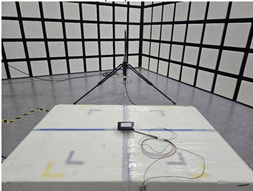
FACE OFF TEST PHOTO (NFC)
