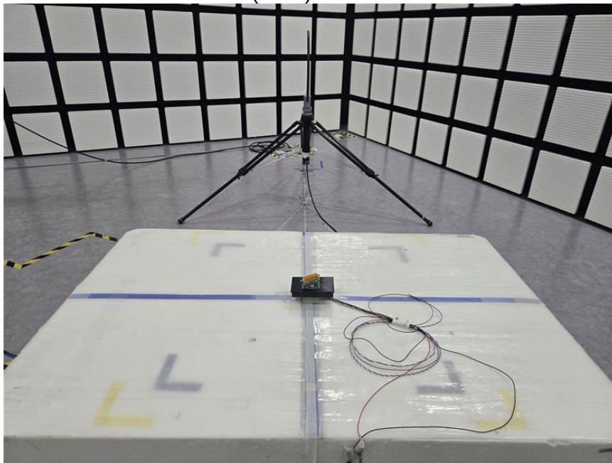
FACE OFF TEST PHOTO (WPT)
