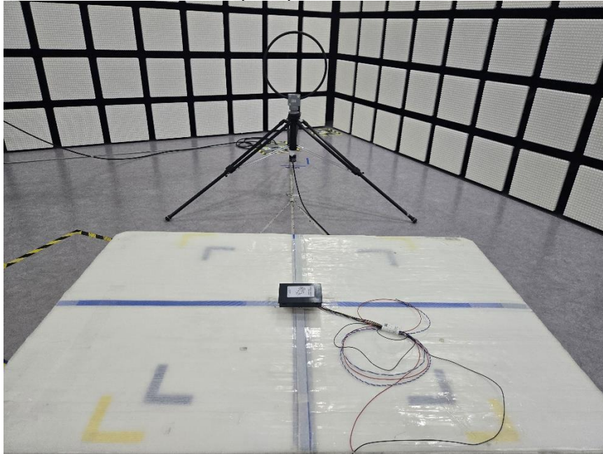
FACE ON TEST PHOTO (NFC)
