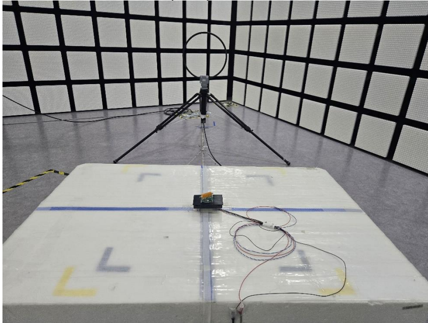
FACE ON TEST PHOTO (WPT)
