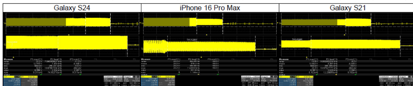
Figure 1-1 WPT Load Removal Power Down
