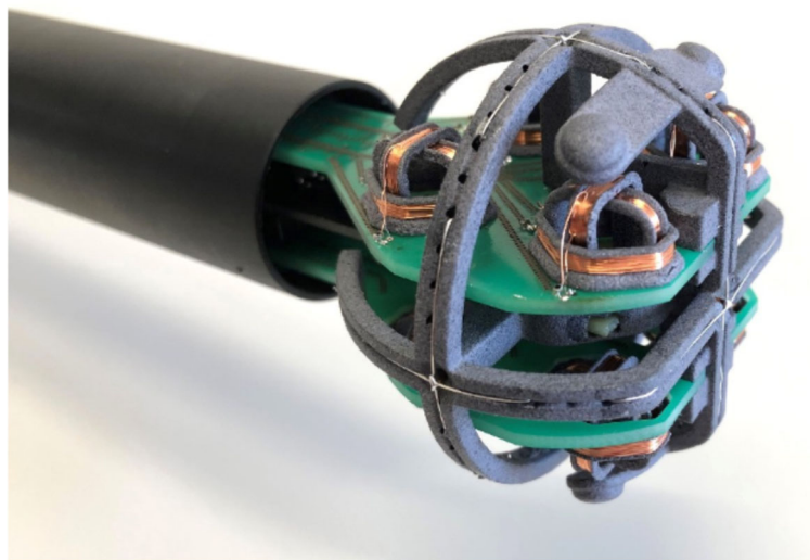
Figure 2-2 MAGPy-8H3D+E3 V2 Measurement Probe
