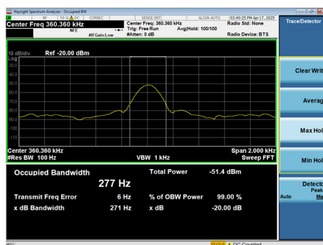
Figure 1-2 WPT Occupied Bandwidth
