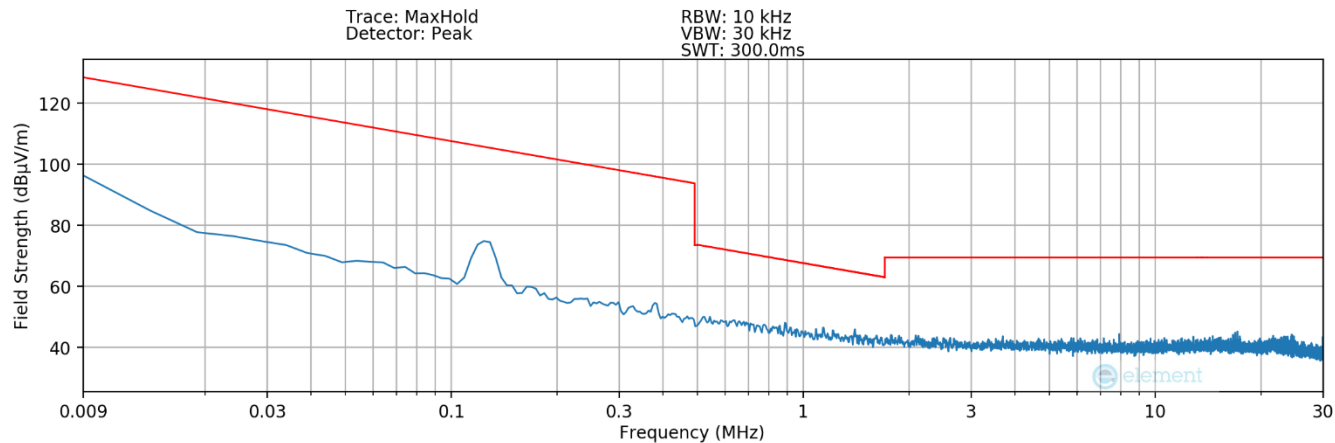
Plot 7-4. Radiated Spurious Plot 9kHz – 30MHz (Pol. X – Condition1)
