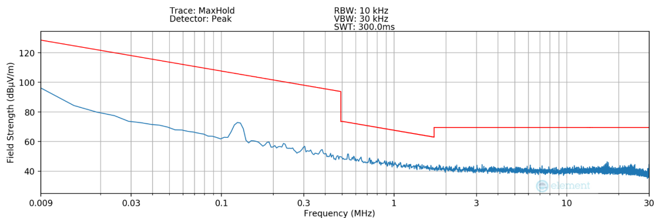
Plot 7-5Radiated Spurious Plot 9kHz – 30MHz (Pol. Y – Condition1)
