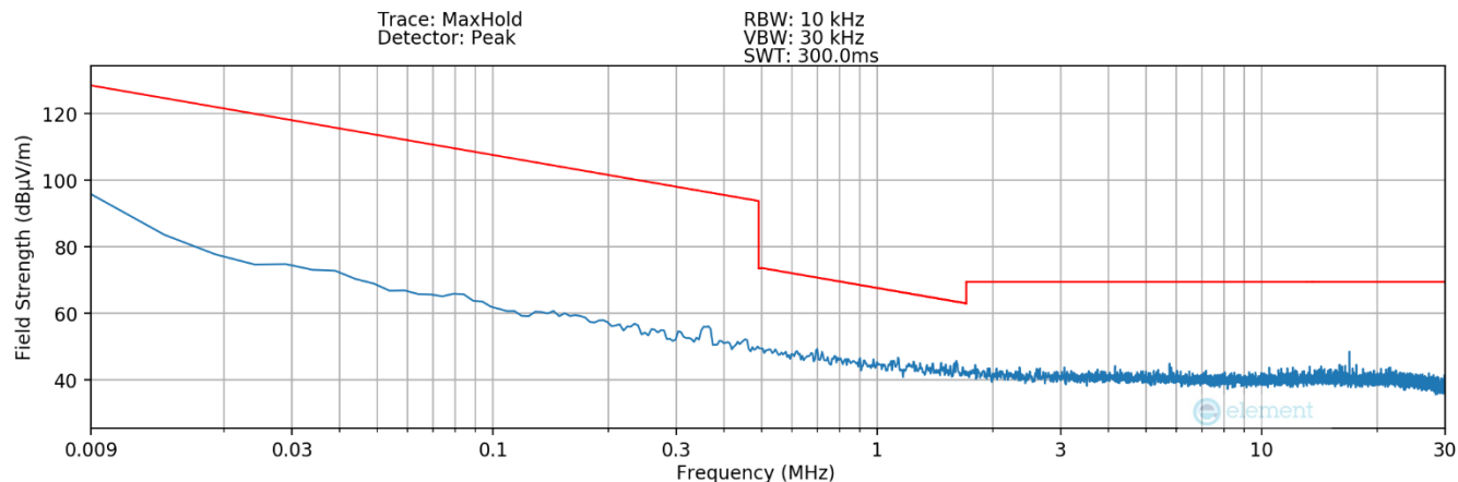
Plot 7-7. Radiated Spurious Plot 9kHz – 30MHz (Pol. X – Condition2)
