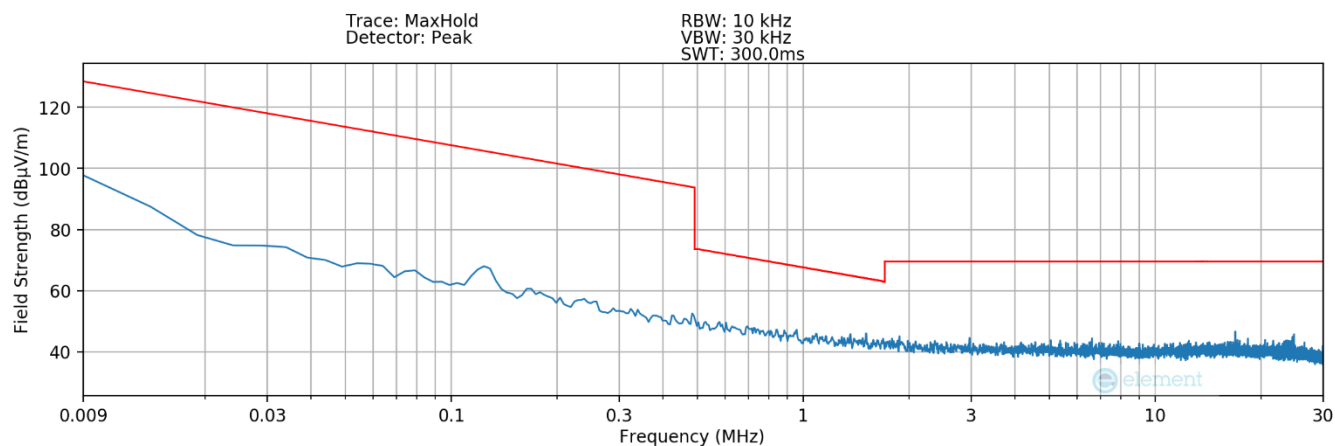
Plot 7-6. Radiated Spurious Plot 9kHz – 30MHz (Pol. Z– Condition1)
