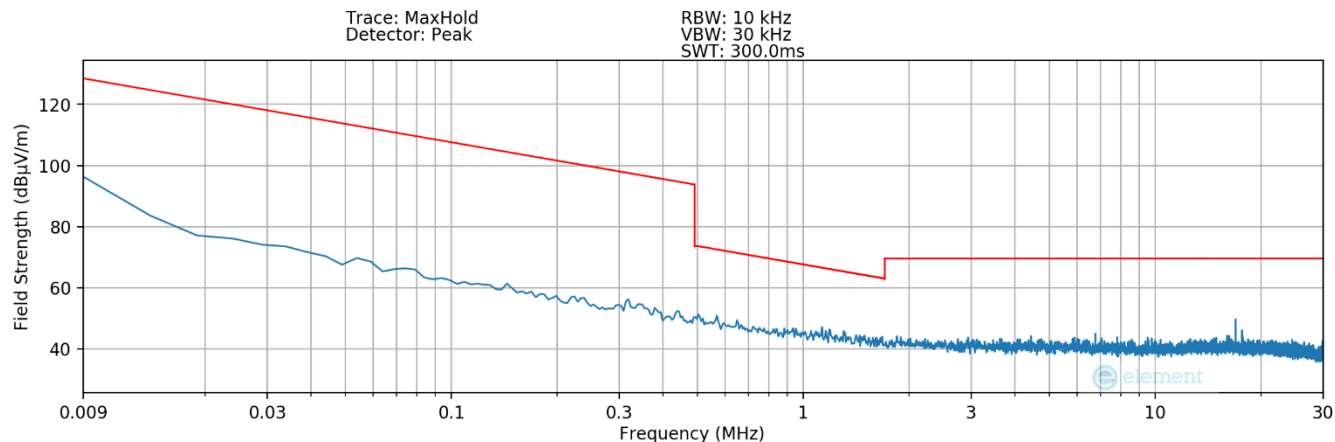
Plot 7-12. Radiated Spurious Plot 9kHz – 30MHz (Pol. Z– Condition3)
