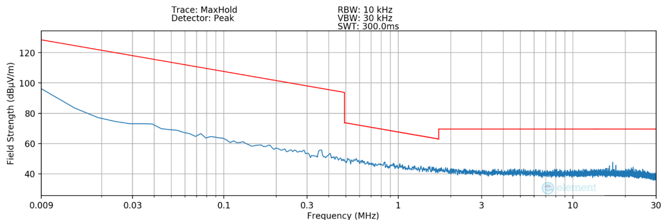
Plot 7-8Radiated Spurious Plot 9kHz – 30MHz (Pol. Y – Condition2)
