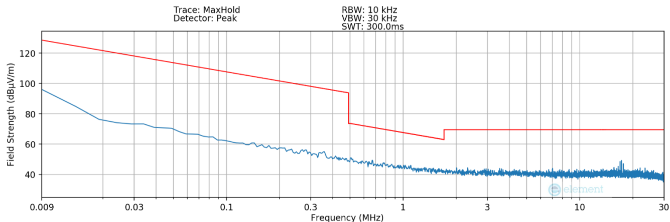
Plot 7-11Radiated Spurious Plot 9kHz – 30MHz (Pol. Y – Condition3)
