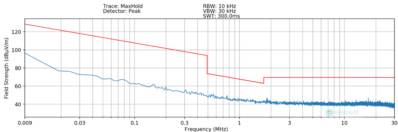
Plot 7-9. Radiated Spurious Plot 9kHz – 30MHz (Pol. Z– Condition2)
