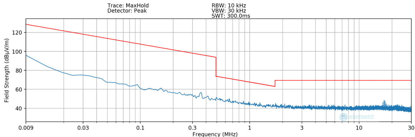
Plot 7-10. Radiated Spurious Plot 9kHz – 30MHz (Pol. X – Condition3)
