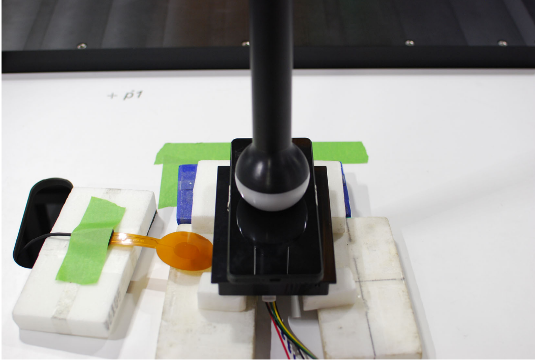
Test Setup Photo 7 EPP, Back side, 0mm
