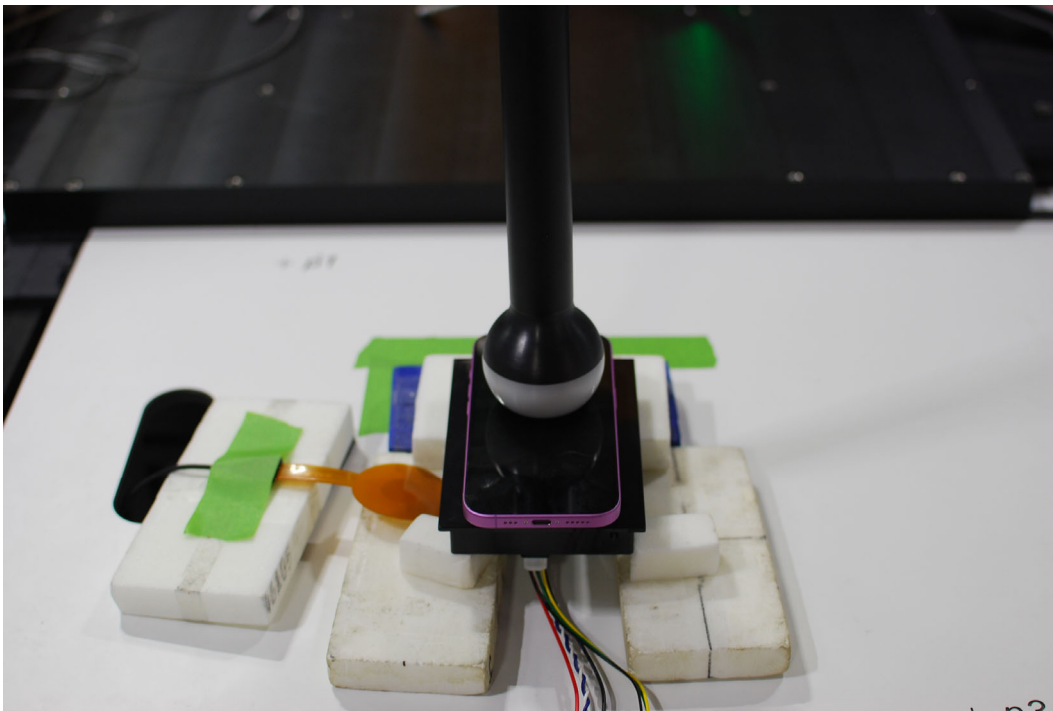
Test Setup Photo 8 MPP (RX1), Back side, 0mm
