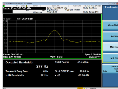
Figure 2-2 WPT Occupied Bandwidth
