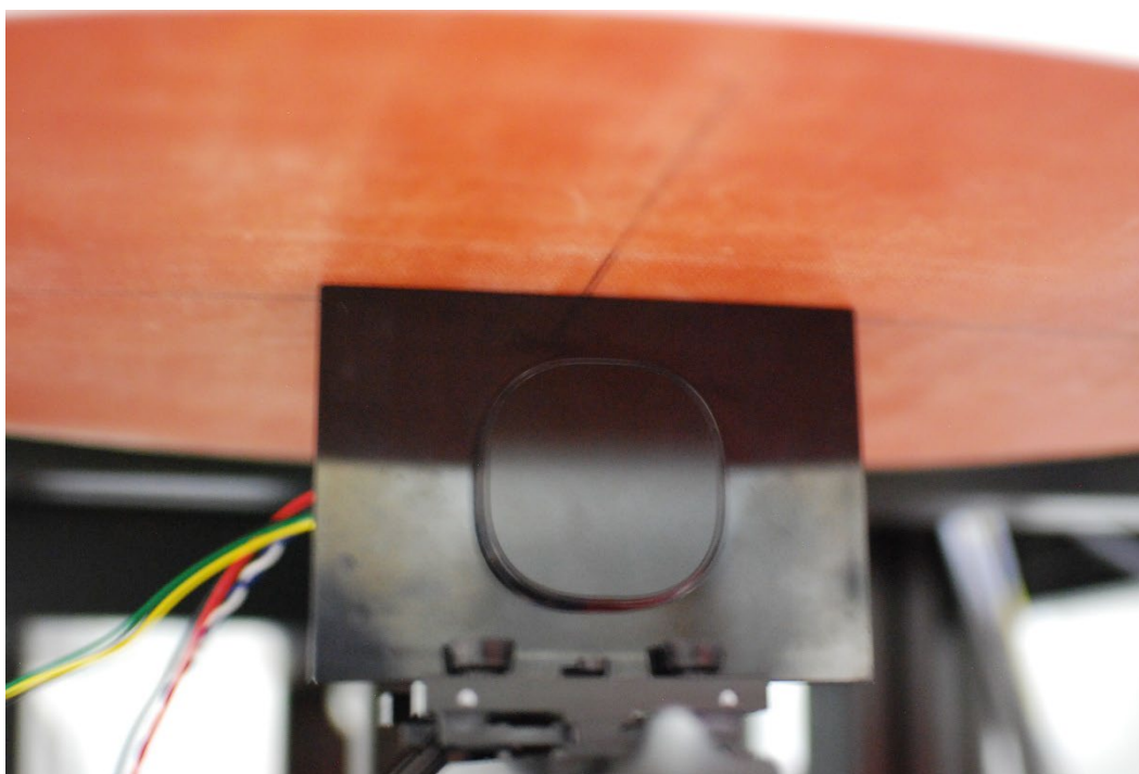
SAR Test Setup Photo 4 – NFC Body, Bottom Side at 0mm
