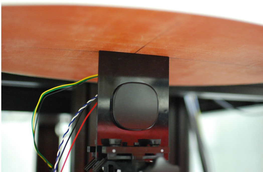
SAR Test Setup Photo 6 – NFC Body, Right Side at 0mm
