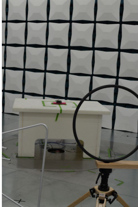
Figure 3. Test Setup – 30MHz-1GHz
