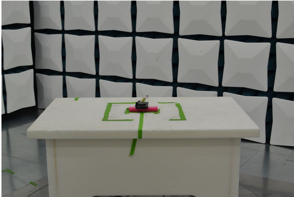
Figure 1. Test Setup – 30MHz-1GHz
