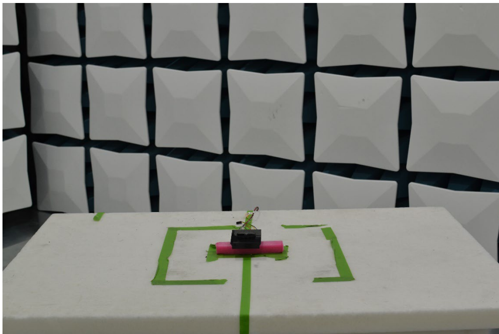
Figure 2. Test Setup – 30MHz-1GHz
