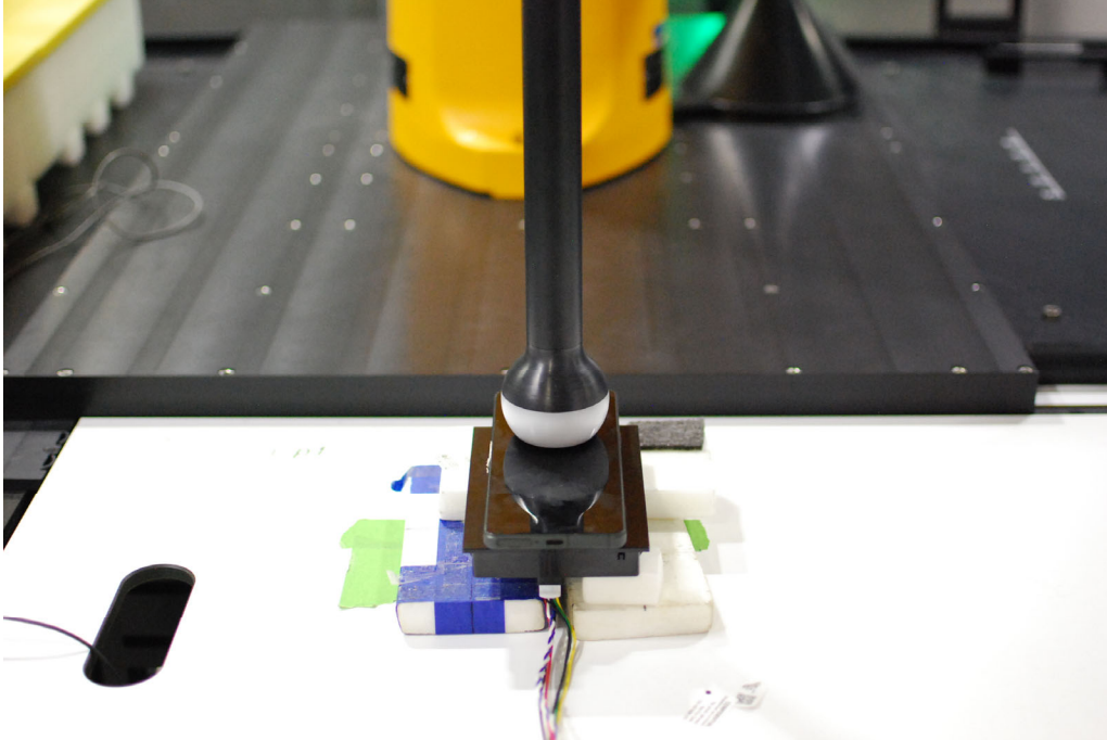
Test Setup Photo 7 EPP, Front Side, 0mm
