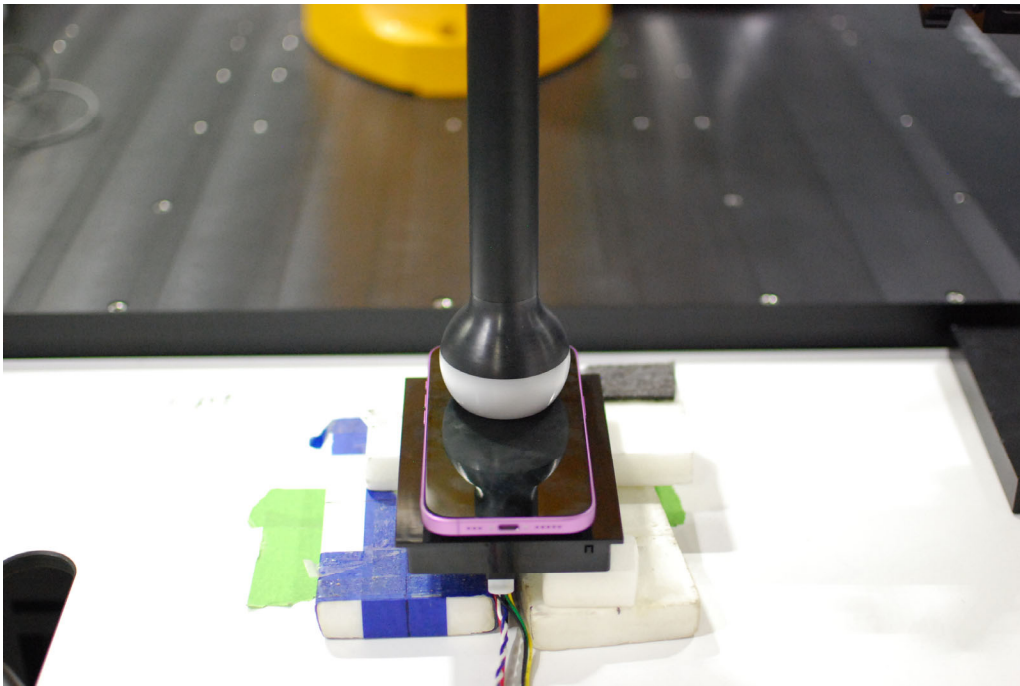
Test Setup Photo 8 MPP (RX1), Front Side, 0mm
