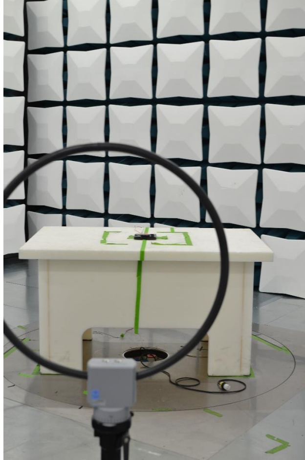
Figure 3. Test Setup – <30MHz
