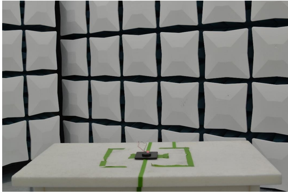
Figure 1. Test Setup – 30MHz-1GHz
