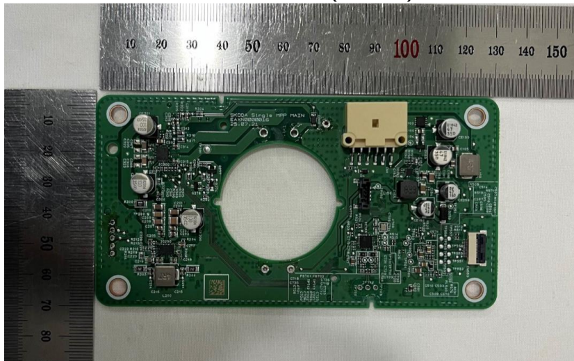
SCB LED Variant (Bottom)
