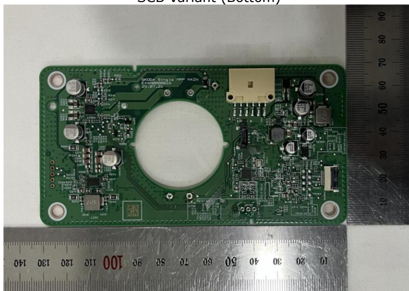
SCB Variant (Bottom)
