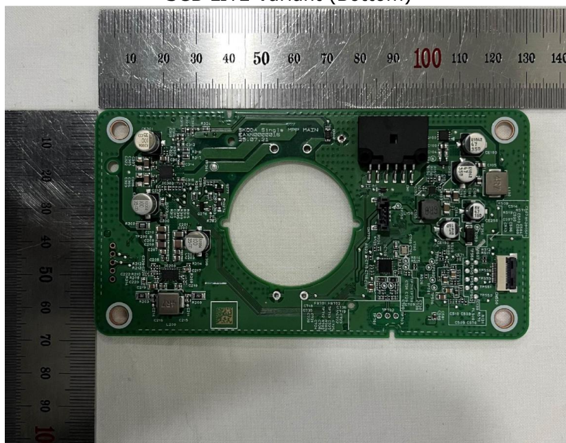
SCB LITE Variant (Bottom)
