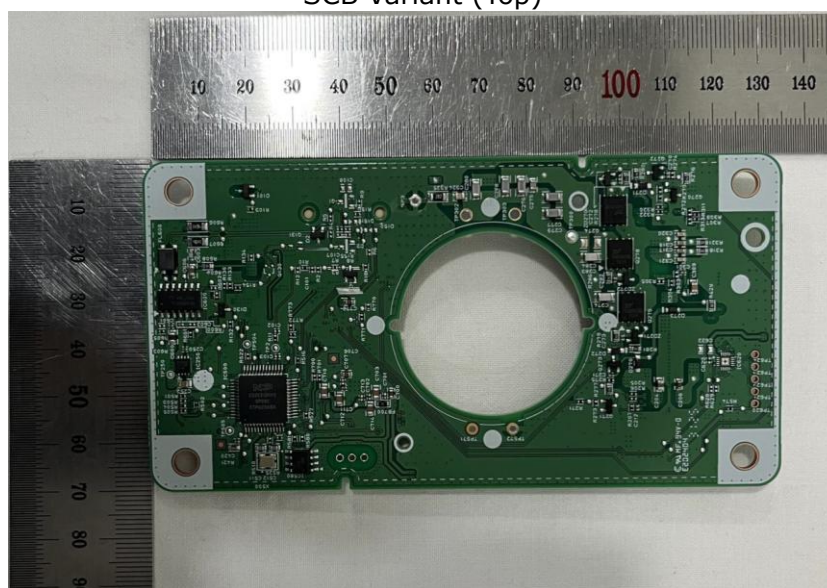
SCB Variant (Top)
