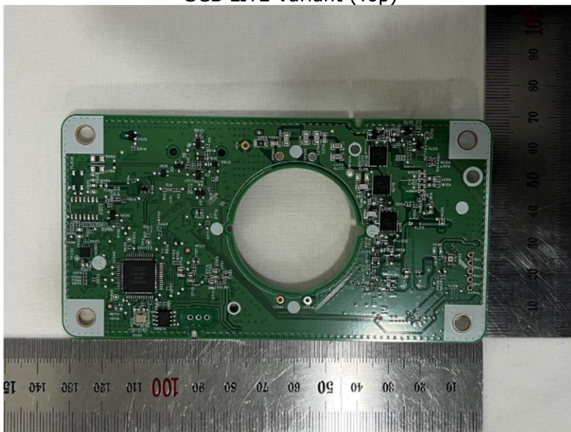
SCB LITE Variant (Top)
