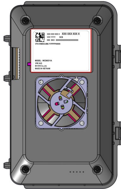
Printed Label Location
