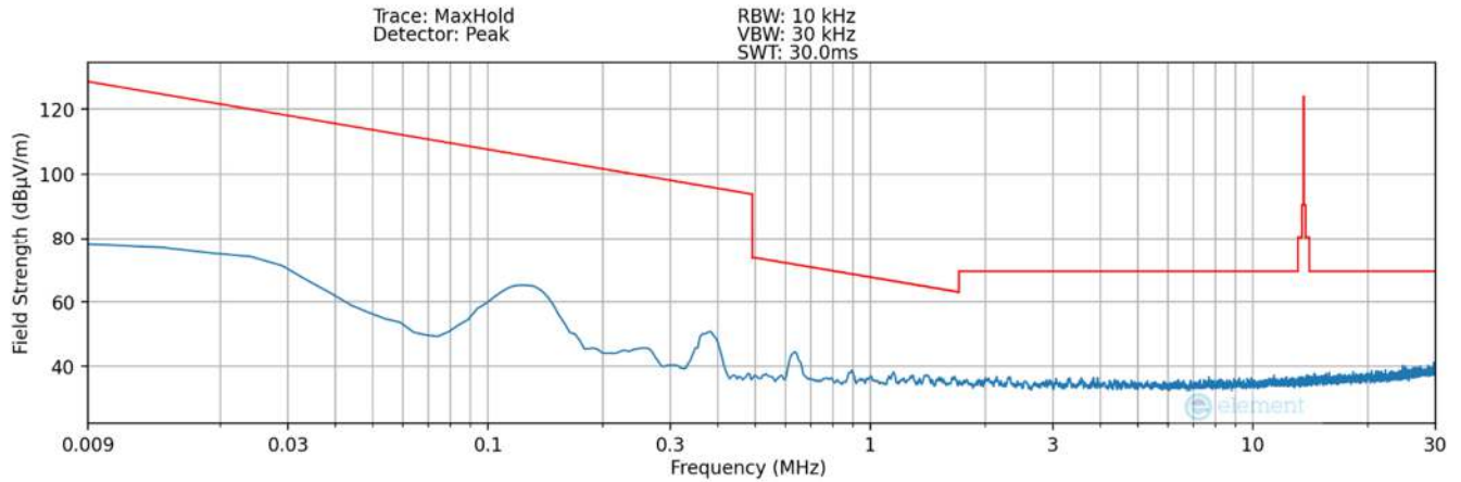
Plot 7-21. Radiated Spurious Plot 9kHz – 30MHz (Pol. Y – Condition2) – SCB Lite
