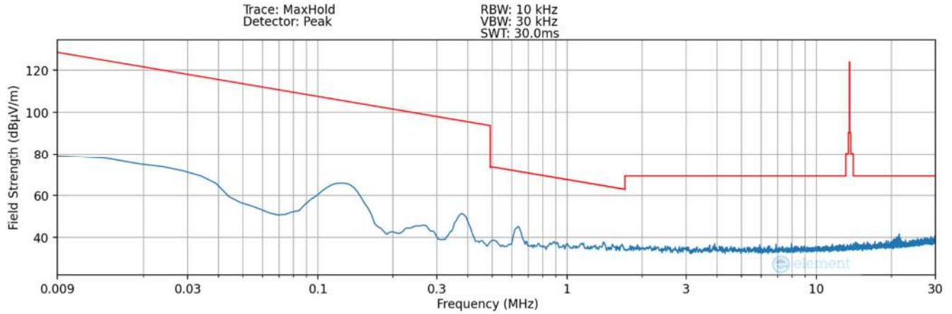
Plot 7-14. Radiated Spurious Plot 9kHz – 30MHz (Pol. X – Condition2) – SCB LED
