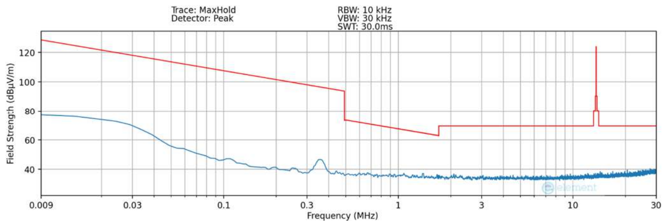
Plot 7-31. Radiated Spurious Plot 9kHz – 30MHz (Pol. Z – Condition3) – SCB Lite
