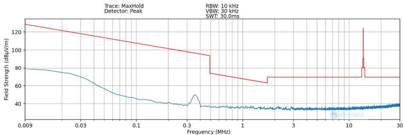
Plot 7-30. Radiated Spurious Plot 9kHz – 30MHz (Pol. Y – Condition3) – SCB Lite
