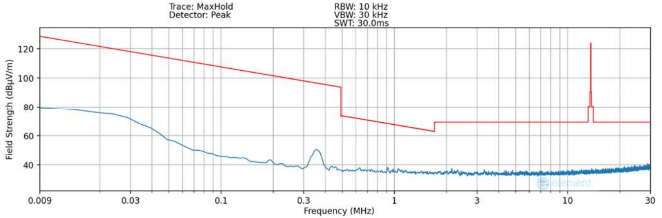
Plot 7-23. Radiated Spurious Plot 9kHz – 30MHz (Pol. X – Condition3) – SCB LED
