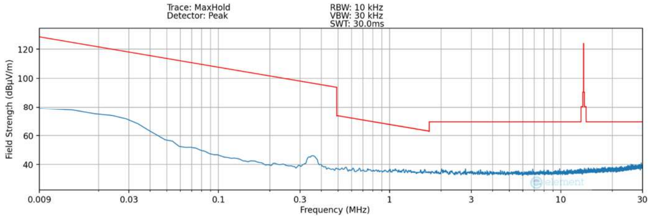
Plot 7-37. Radiated Spurious Plot 9kHz – 30MHz (Pol. Z – Condition4) – SCB
