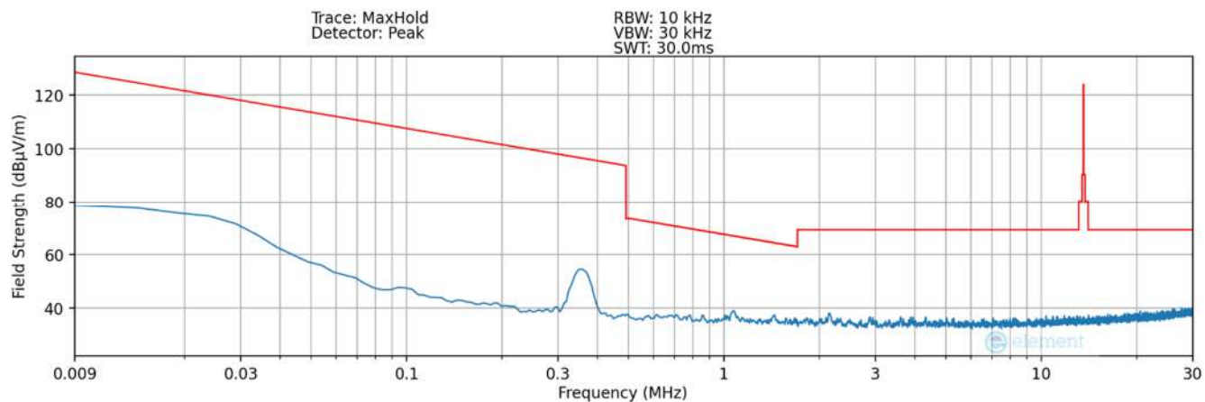
Plot 7-39. Radiated Spurious Plot 9kHz – 30MHz (Pol. Y – Condition4) – SCB Lite
