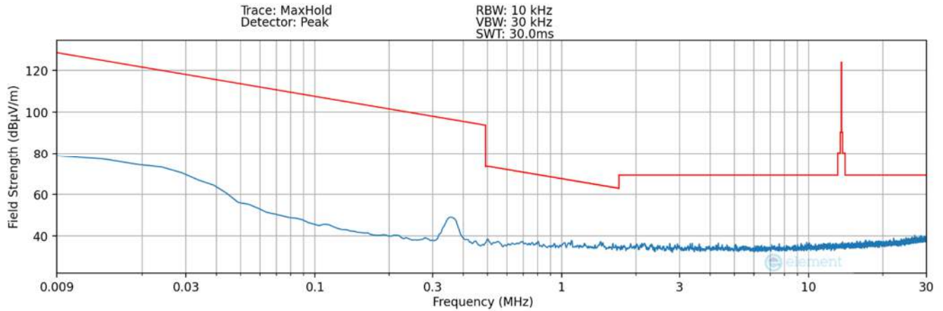
Plot 7-27. Radiated Spurious Plot 9kHz – 30MHz (Pol. Y – Condition3) – SCB
