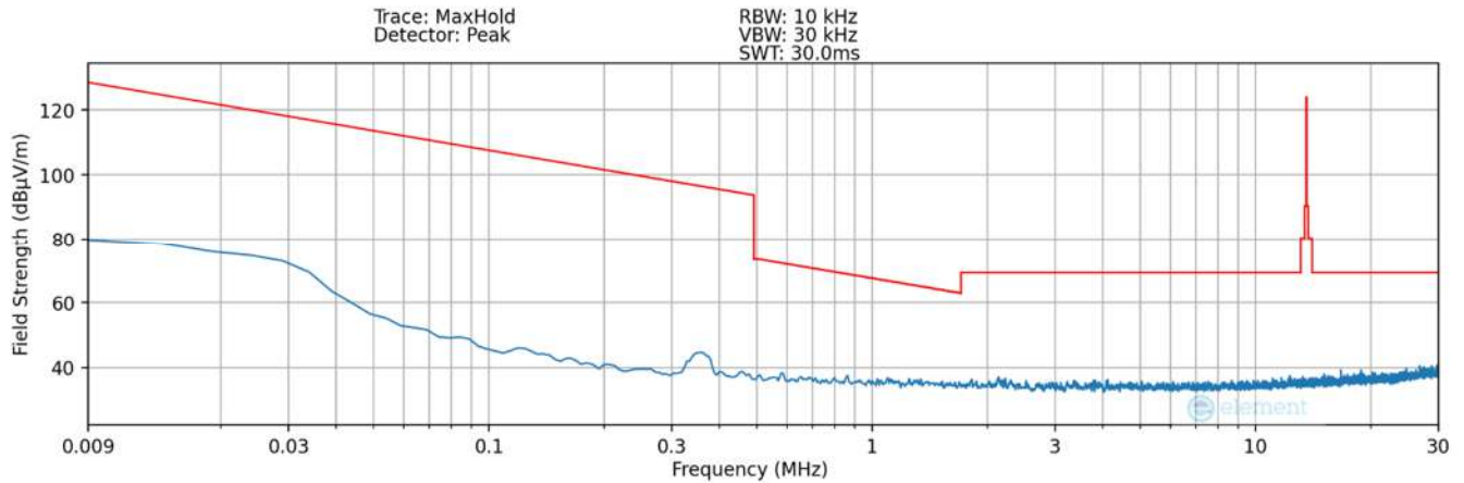
Plot 7-25. Radiated Spurious Plot 9kHz – 30MHz (Pol. Z – Condition3) – SCB LED
