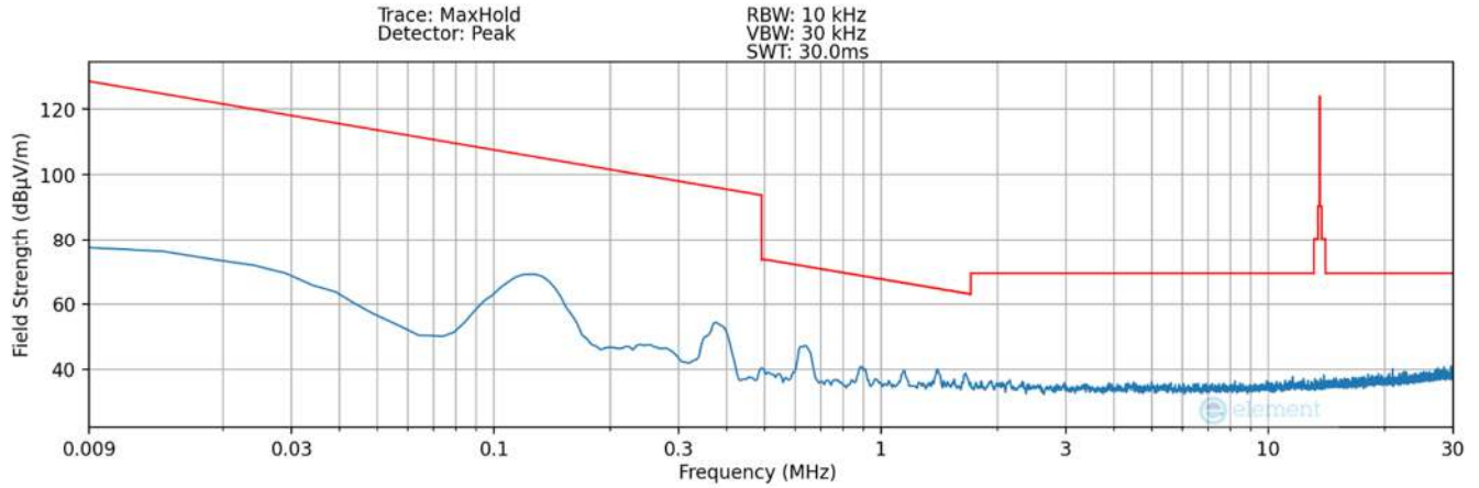
Plot 7-20. Radiated Spurious Plot 9kHz – 30MHz (Pol. X – Condition2) – SCB Lite
