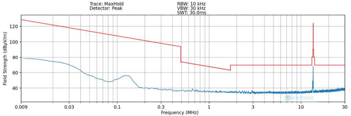
Plot 7-12. Radiated Spurious Plot 9kHz – 30MHz (Pol. Y – Condition1) – SCB Lite
