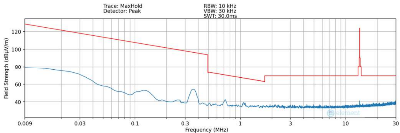
Plot 7-34. Radiated Spurious Plot 9kHz – 30MHz (Pol. Z – Condition4) – SCB LED
