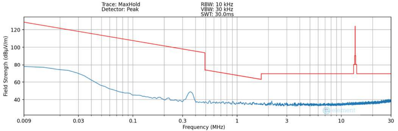
Plot 7-36. Radiated Spurious Plot 9kHz – 30MHz (Pol. Y – Condition4) – SCB
