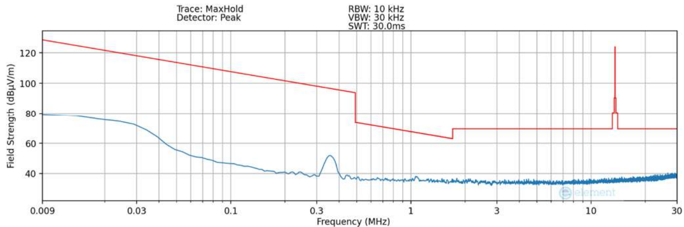
Plot 7-29. Radiated Spurious Plot 9kHz – 30MHz (Pol. X – Condition3) – SCB Lite
