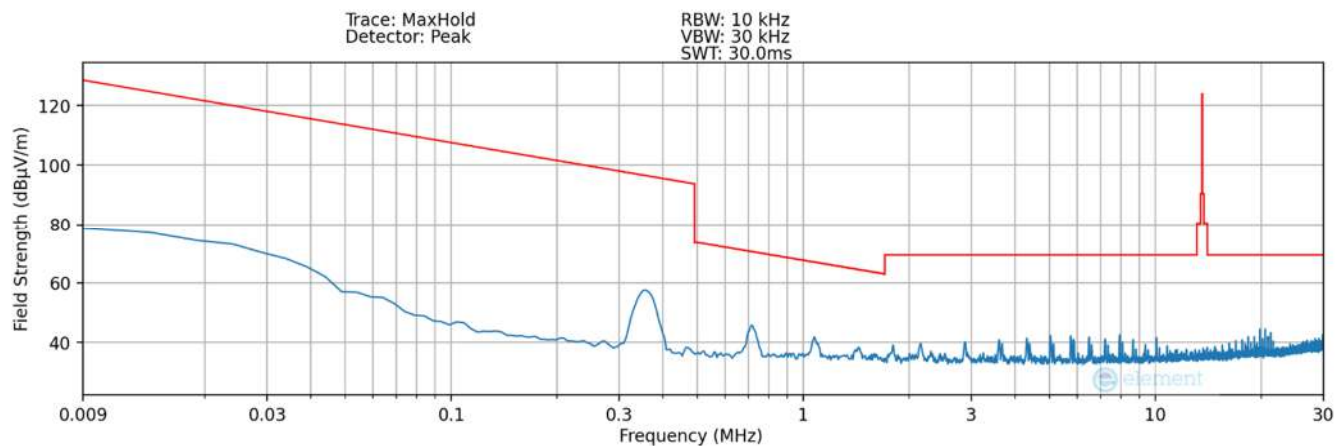
Plot 7-33. Radiated Spurious Plot 9kHz – 30MHz (Pol. Y – Condition4) – SCB LED
