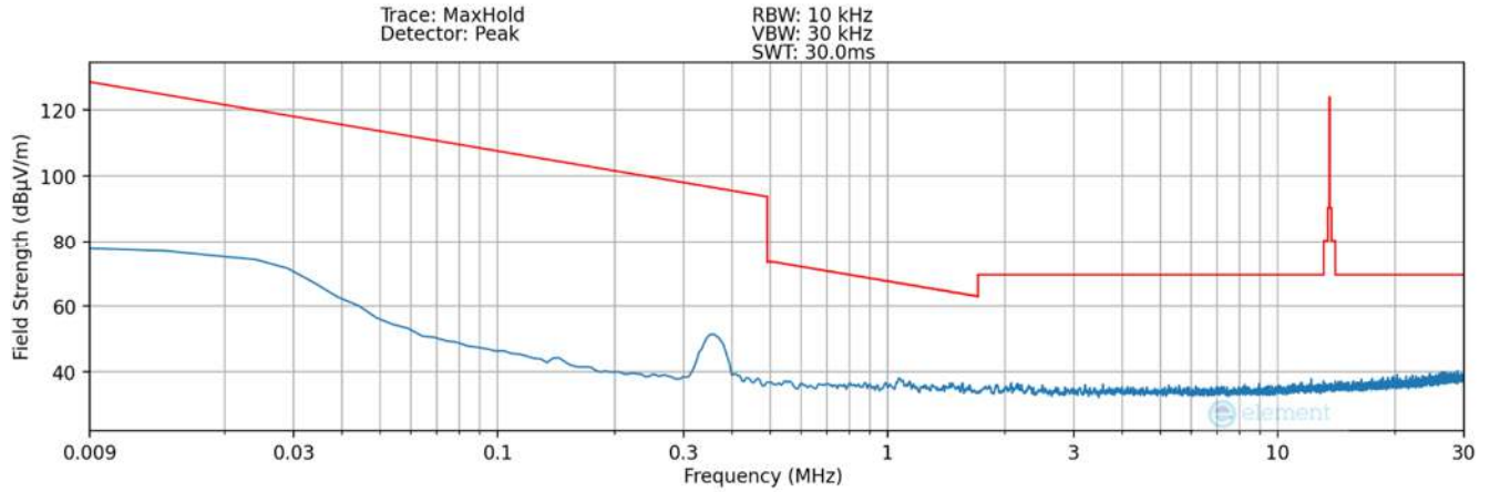
Plot 7-35. Radiated Spurious Plot 9kHz – 30MHz (Pol. X – Condition4) – SCB
