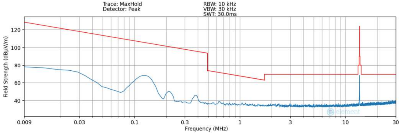
Plot 7-11. Radiated Spurious Plot 9kHz – 30MHz (Pol. X – Condition1) – SCB Lite
