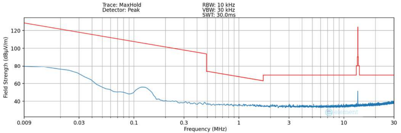
Plot 7-6. Radiated Spurious Plot 9kHz – 30MHz (Pol. Y – Condition1) – SCB LED
