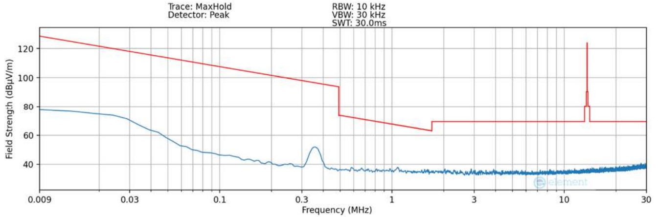
Plot 7-26. Radiated Spurious Plot 9kHz – 30MHz (Pol. X – Condition3) – SCB
