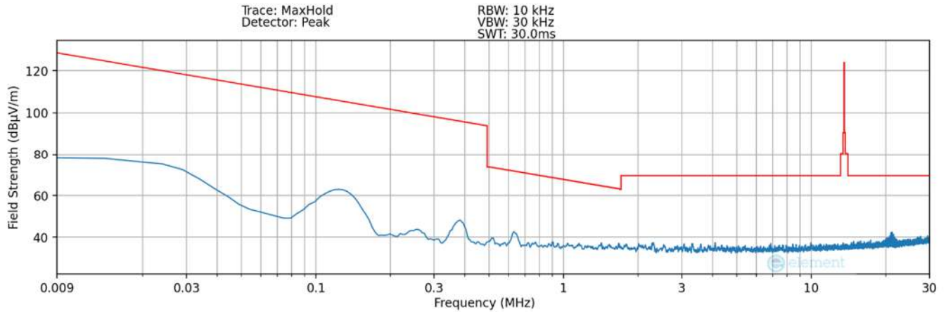
Plot 7-15. Radiated Spurious Plot 9kHz – 30MHz (Pol. Y – Condition2) – SCB LED
