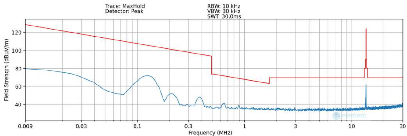
Plot 7-10. Radiated Spurious Plot 9kHz – 30MHz (Pol. Z – Condition1) – SCB
