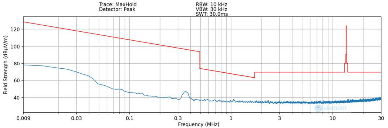
Plot 7-28. Radiated Spurious Plot 9kHz – 30MHz (Pol. Z – Condition3) – SCB
