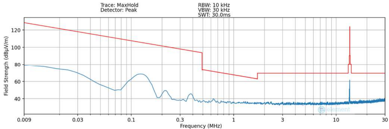
Plot 7-8. Radiated Spurious Plot 9kHz – 30MHz (Pol. X – Condition1) – SCB
