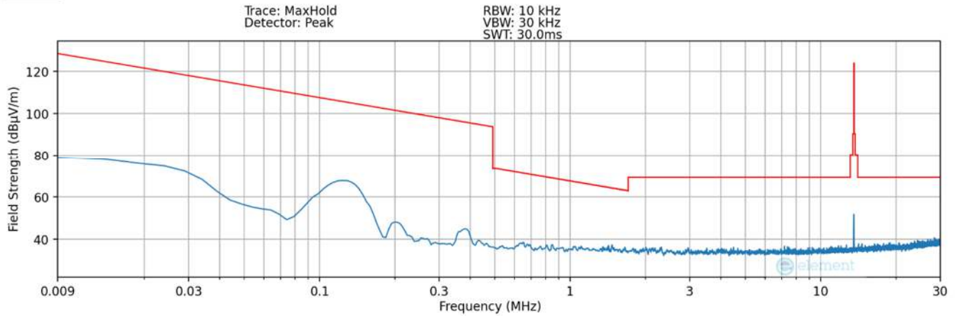
Plot 7-5. Radiated Spurious Plot 9kHz – 30MHz (Pol. X – Condition1) – SCB LED
