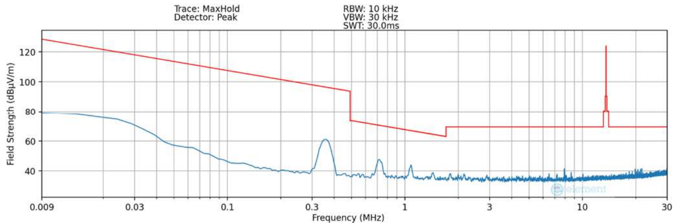
Plot 7-32. Radiated Spurious Plot 9kHz – 30MHz (Pol. X – Condition4) – SCB LED
