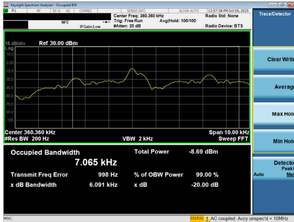
Plot 7-3. Occupied Bandwidth Measurement – Condition 3
