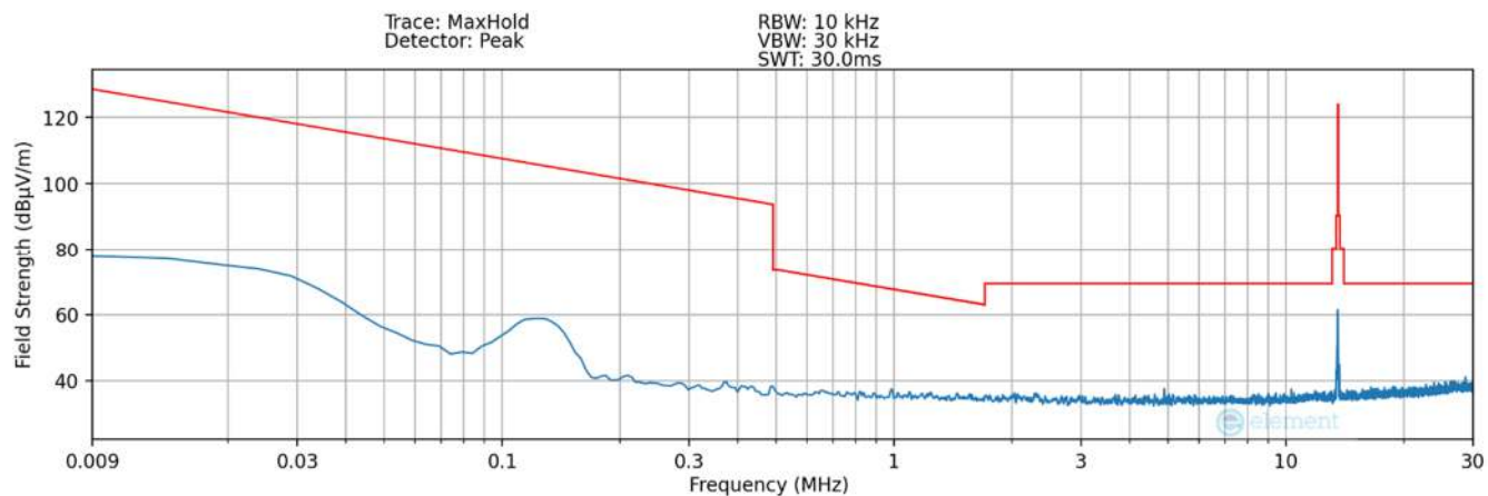
Plot 7-9. Radiated Spurious Plot 9kHz – 30MHz (Pol. Y – Condition1) – SCB
