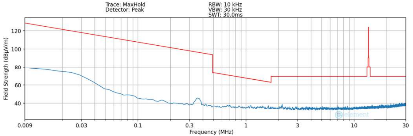
Plot 7-24. Radiated Spurious Plot 9kHz – 30MHz (Pol. Y – Condition3) – SCB LED
