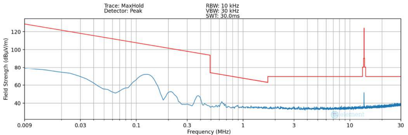
Plot 7-7. Radiated Spurious Plot 9kHz – 30MHz (Pol. Z – Condition1) – SCB LED
