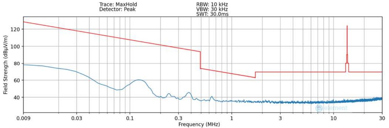
Plot 7-16. Radiated Spurious Plot 9kHz – 30MHz (Pol. Z – Condition2) – SCB LED
