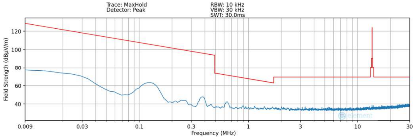
Plot 7-22. Radiated Spurious Plot 9kHz – 30MHz (Pol. Z – Condition2) – SCB Lite
