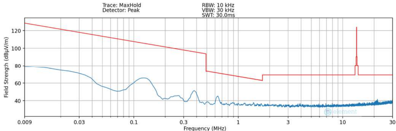
Plot 7-17. Radiated Spurious Plot 9kHz – 30MHz (Pol. X – Condition2) – SCB
