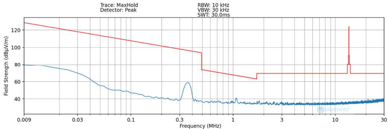
Plot 7-38. Radiated Spurious Plot 9kHz – 30MHz (Pol. X – Condition4) – SCB Lite
