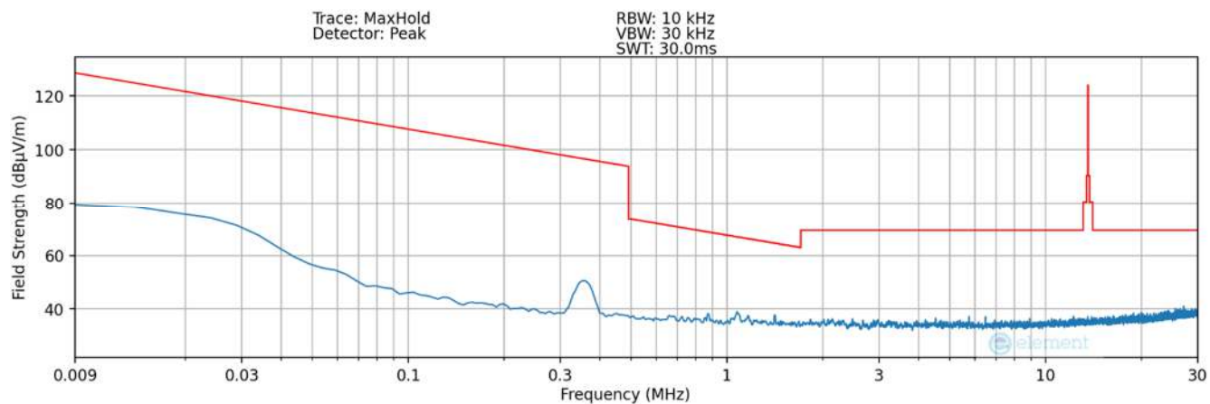
Plot 7-40. Radiated Spurious Plot 9kHz – 30MHz (Pol. Z – Condition4) – SCB Lite
