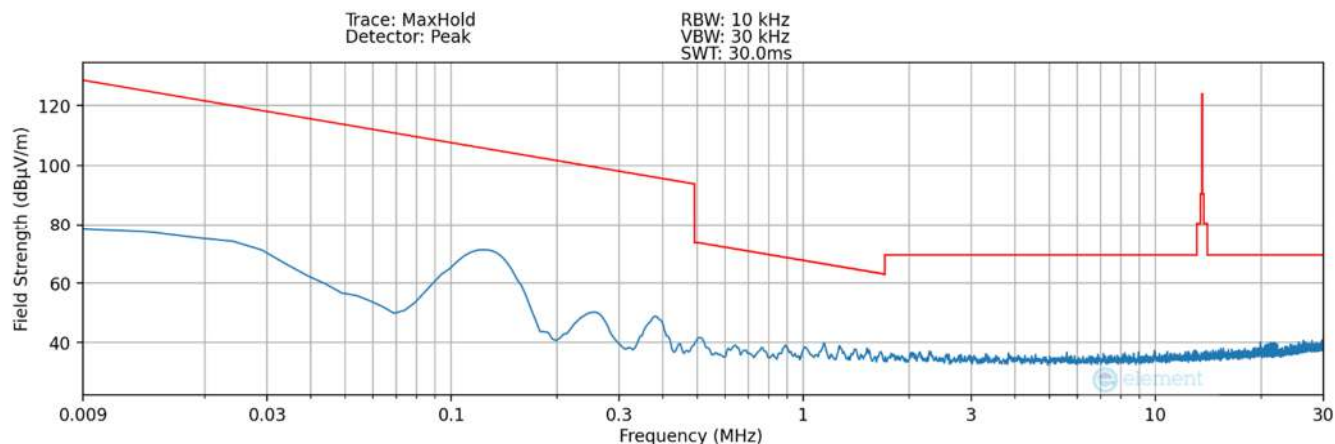
Plot 7-18. Radiated Spurious Plot 9kHz – 30MHz (Pol. Y – Condition2) – SCB
