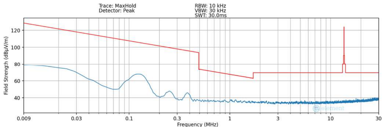
Plot 7-19. Radiated Spurious Plot 9kHz – 30MHz (Pol. Z – Condition2) – SCB
