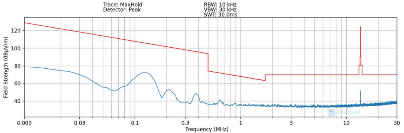
Plot 7-13. Radiated Spurious Plot 9kHz – 30MHz (Pol. Z – Condition1) – SCB Lite
