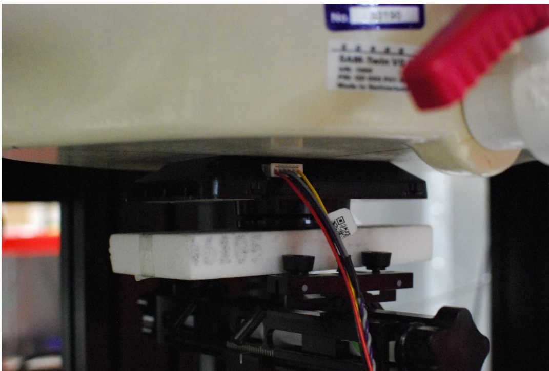
SAR Test Setup Photo 2 – NFC Body, Back Side at 0mm
