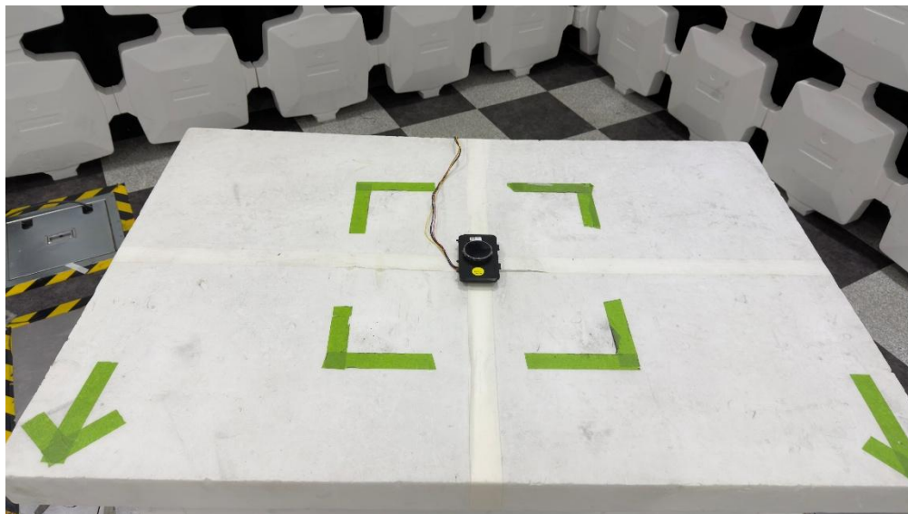
Figure 2. Test Setup – 9kHz-1GHz
