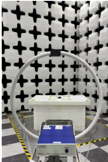
Figure 3. Test Setup – 9kHz-30MHz
