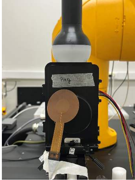
Test Setup Photo 3 Standby (Ping) Signal, Top Side, 0mm
