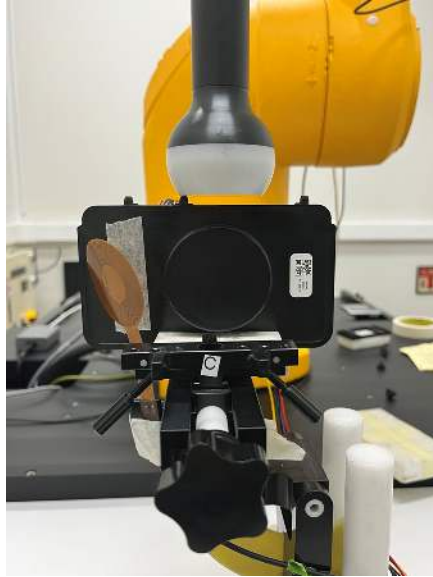
Test Setup Photo 5 Standby (Ping) Signal, Right Side, 0mm
