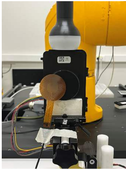
Test Setup Photo 4 Standby (Ping) Signal, Bottom Side, 0mm
