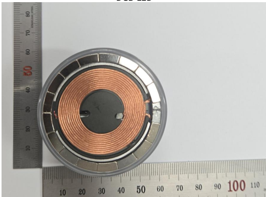
DCB LED
