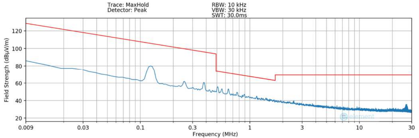
Plot 7-26. Radiated Spurious Plot 9kHz – 30MHz (Pol. X- #4) – DCB
