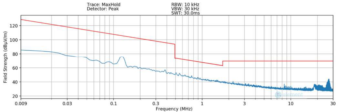
Plot 7-27. Radiated Spurious Plot 9kHz – 30MHz (Pol. Y- #4) – DCB
