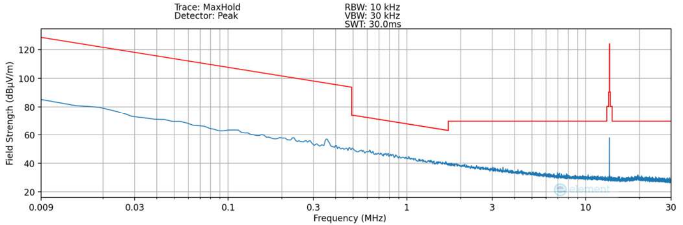
Plot 7-17. Radiated Spurious Plot 9kHz – 30MHz (Pol. X – #3) – DCB LED
