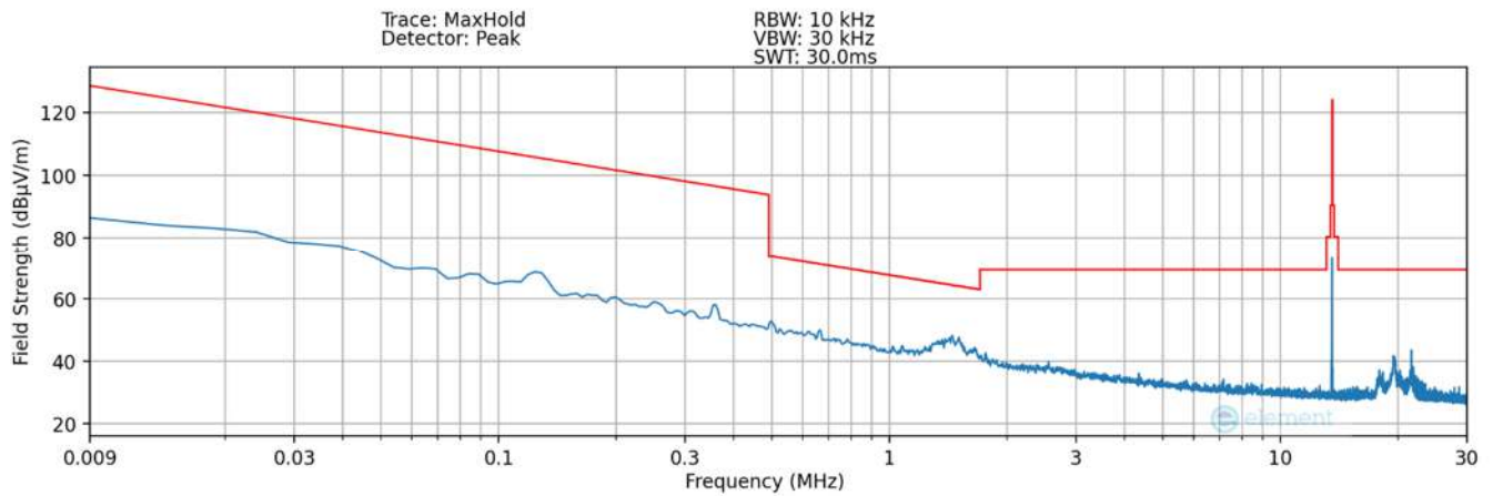
Plot 7-39. Radiated Spurious Plot 9kHz – 30MHz (Pol. Y – #6) – DCB
