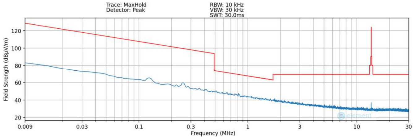
Plot 7-16. Radiated Spurious Plot 9kHz – 30MHz (Pol. Z – #2) – DCB
