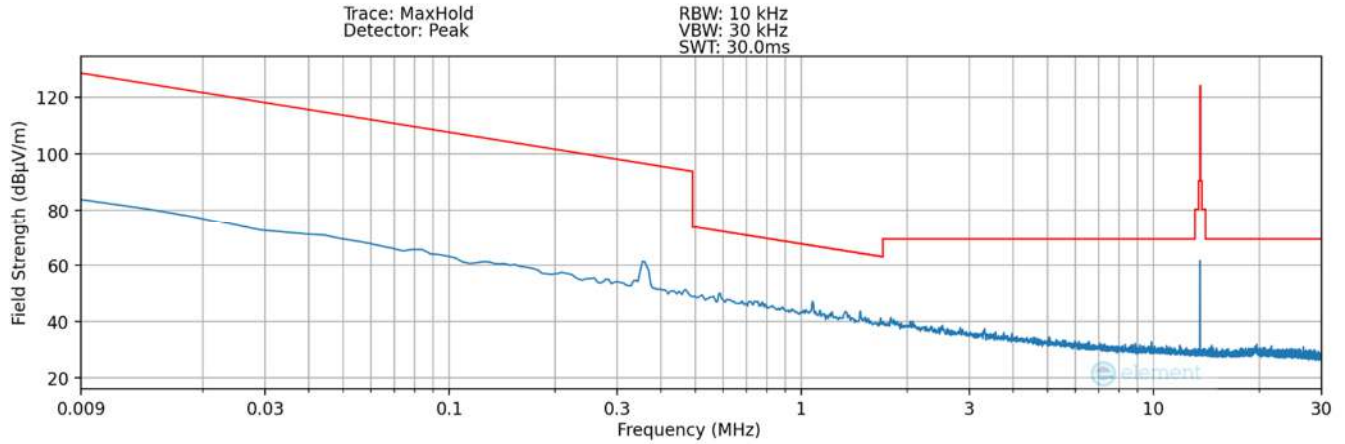
Plot 7-20. Radiated Spurious Plot 9kHz – 30MHz (Pol. X – #3) – DCB
