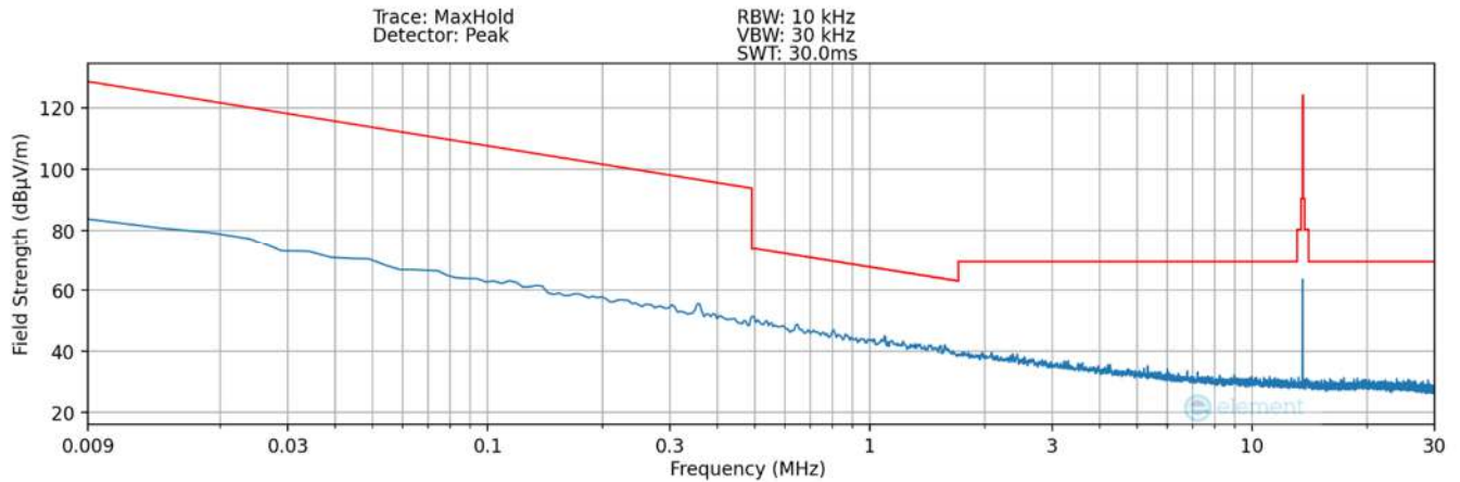
Plot 7-22. Radiated Spurious Plot 9kHz – 30MHz (Pol. Z – #3) – DCB
