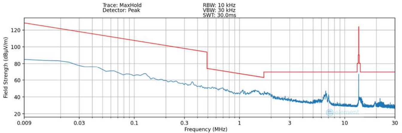
Plot 7-36. Radiated Spurious Plot 9kHz – 30MHz (Pol. Y- #6) – DCB LED
