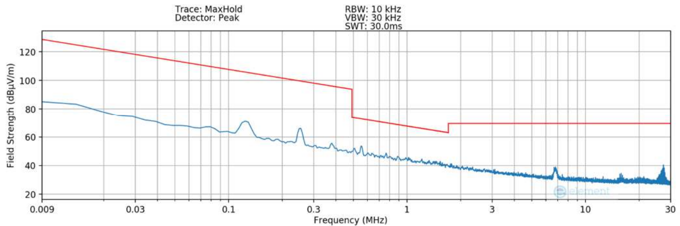
Plot 7-23. Radiated Spurious Plot 9kHz – 30MHz (Pol. X – #4) – DCB LED
