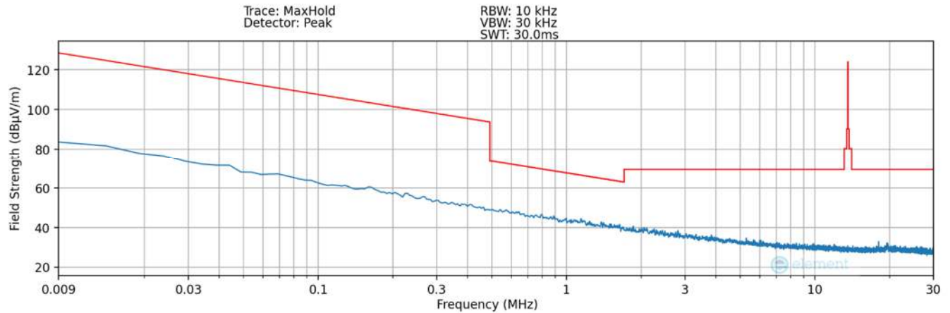
Plot 7-8. Radiated Spurious Plot 9kHz – 30MHz (Pol. X – #1) – DCB
