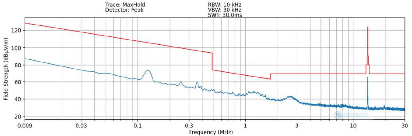
Plot 7-38. Radiated Spurious Plot 9kHz – 30MHz (Pol. X – #6) – DCB
