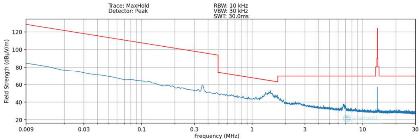
Plot 7-29. Radiated Spurious Plot 9kHz – 30MHz (Pol. X- #5) – DCB LED
