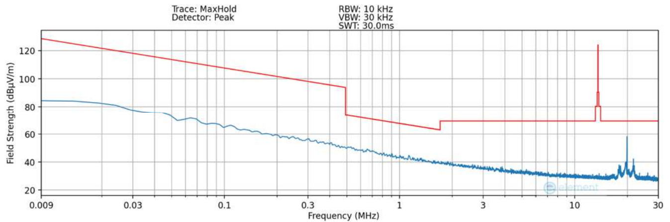
Plot 7-9. Radiated Spurious Plot 9kHz – 30MHz (Pol. Y – #1) – DCB
