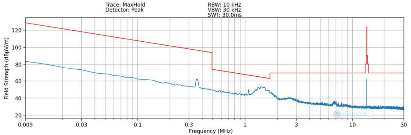
Plot 7-32. Radiated Spurious Plot 9kHz – 30MHz (Pol. X – #5) – DCB
