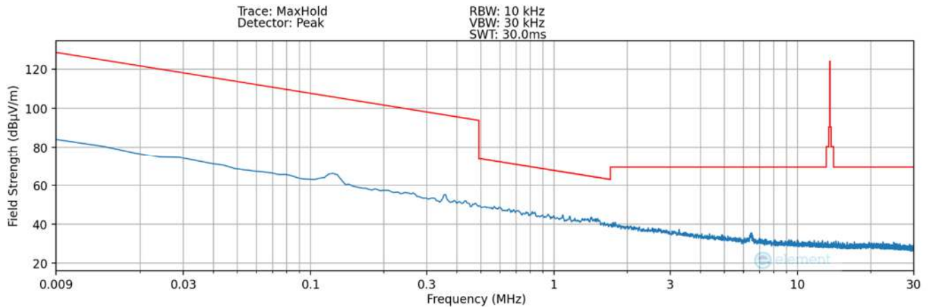
Plot 7-37. Radiated Spurious Plot 9kHz – 30MHz (Pol. Z- #6) – DCB LED
