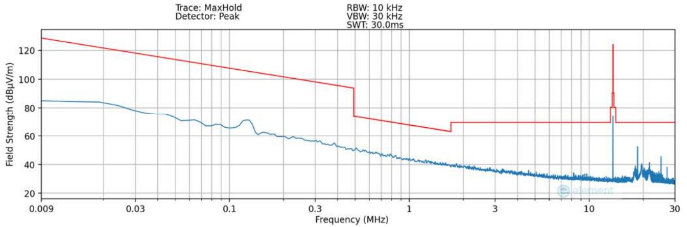
Plot 7-15. Radiated Spurious Plot 9kHz – 30MHz (Pol. Y – #2) – DCB
