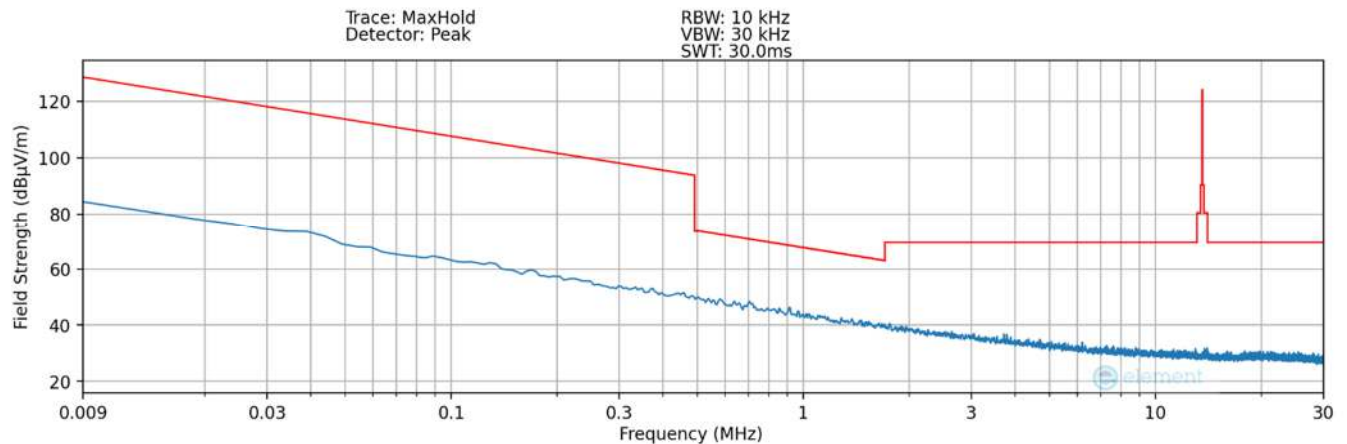
Plot 7-10. Radiated Spurious Plot 9kHz – 30MHz (Pol. Z – #1) – DCB
