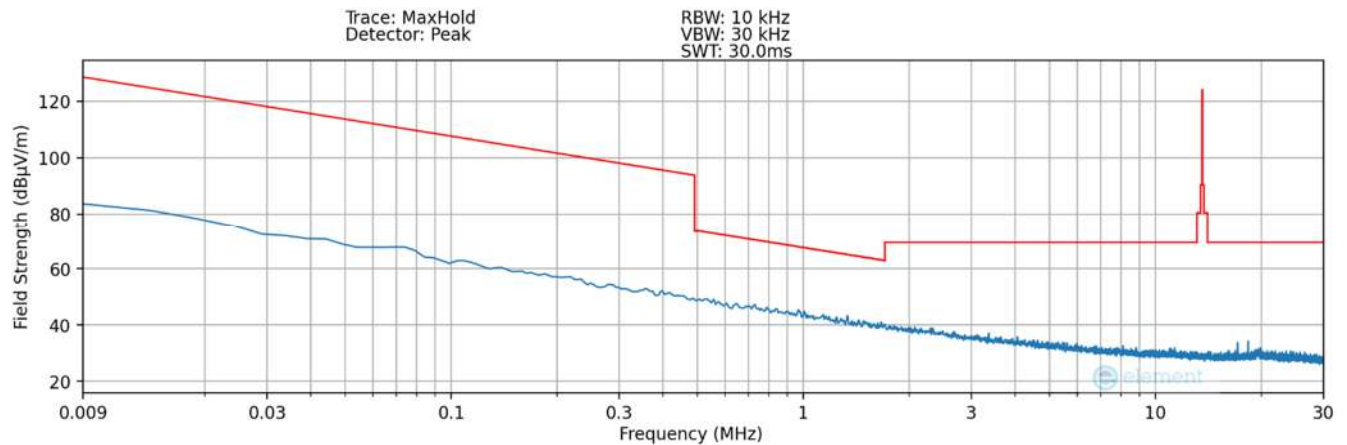
Plot 7-5. Radiated Spurious Plot 9kHz – 30MHz (Pol. X – #1) – DCB LED
