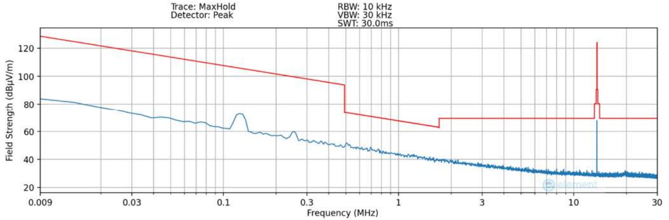
Plot 7-14. Radiated Spurious Plot 9kHz – 30MHz (Pol. X – #2) – DCB
