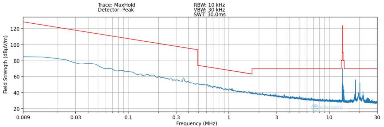
Plot 7-18. Radiated Spurious Plot 9kHz – 30MHz (Pol. Y – #3) – DCB LED
