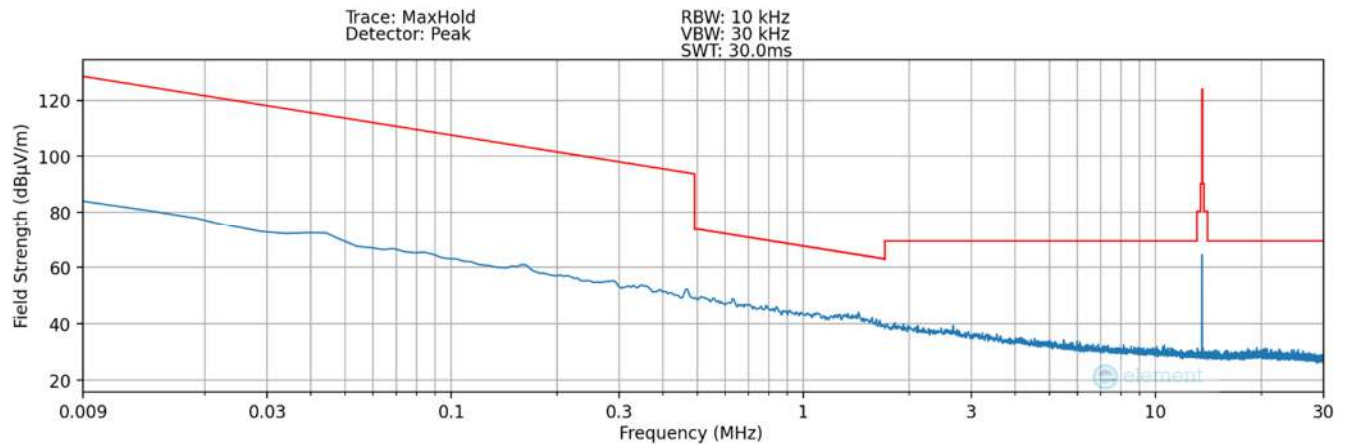
Plot 7-34. Radiated Spurious Plot 9kHz – 30MHz (Pol. Z – #5) – DCB
