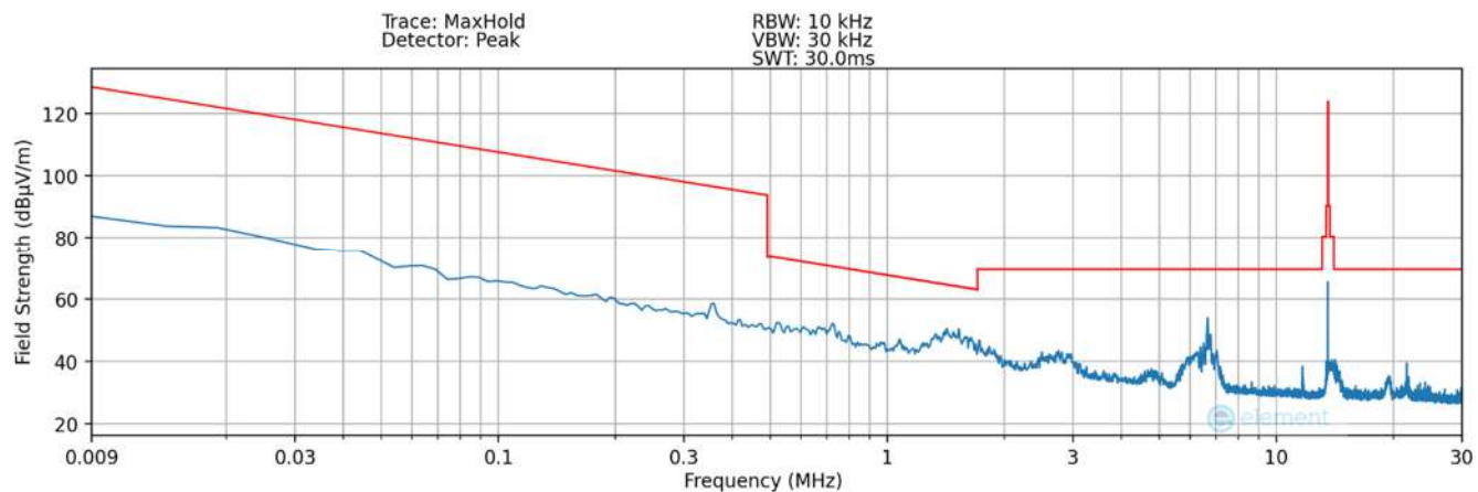
Plot 7-30. Radiated Spurious Plot 9kHz – 30MHz (Pol. Y- #5) – DCB LED
