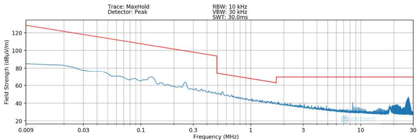
Plot 7-24. Radiated Spurious Plot 9kHz – 30MHz (Pol. Y – #4) – DCB LED
