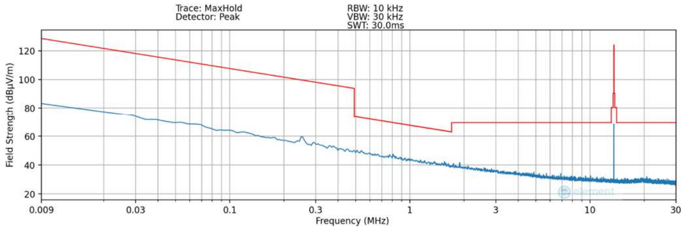
Plot 7-13. Radiated Spurious Plot 9kHz – 30MHz (Pol. Z – #2) – DCB LED
