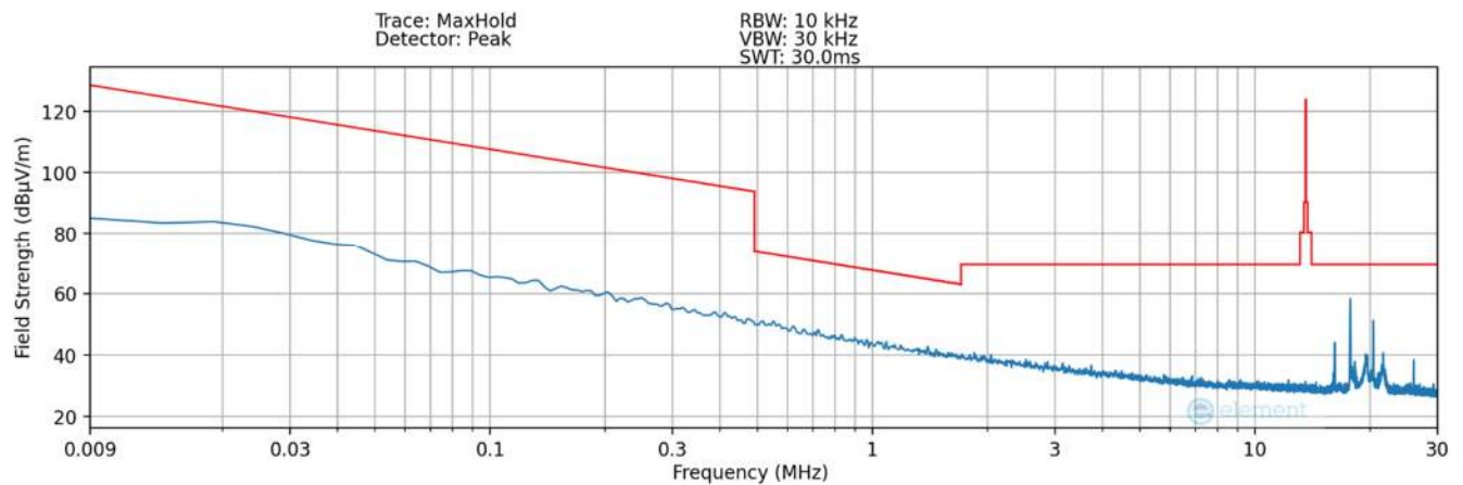
Plot 7-6. Radiated Spurious Plot 9kHz – 30MHz (Pol. Y – #1) – DCB LED
