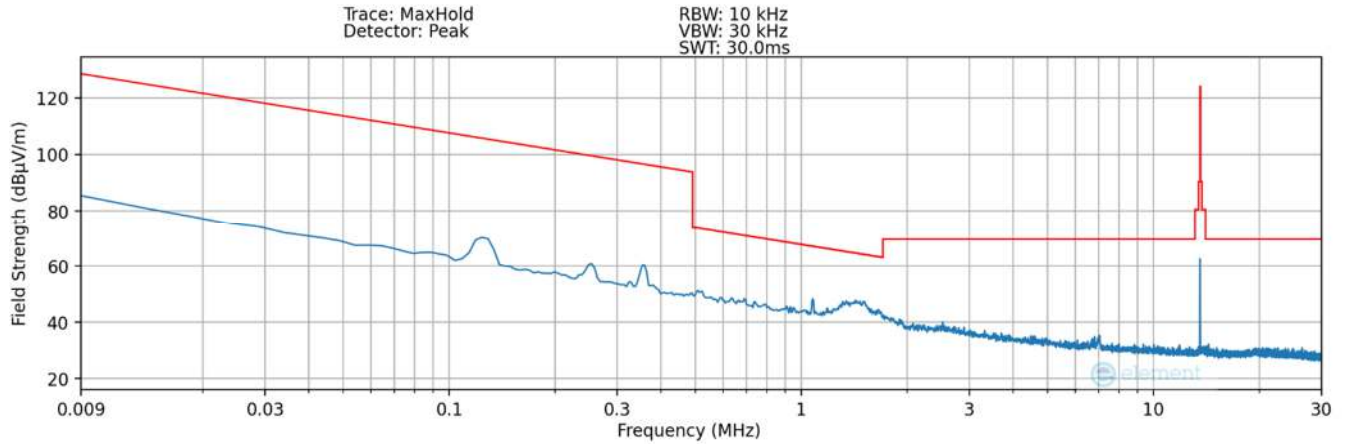
Plot 7-35. Radiated Spurious Plot 9kHz – 30MHz (Pol. X- #6) – DCB LED
