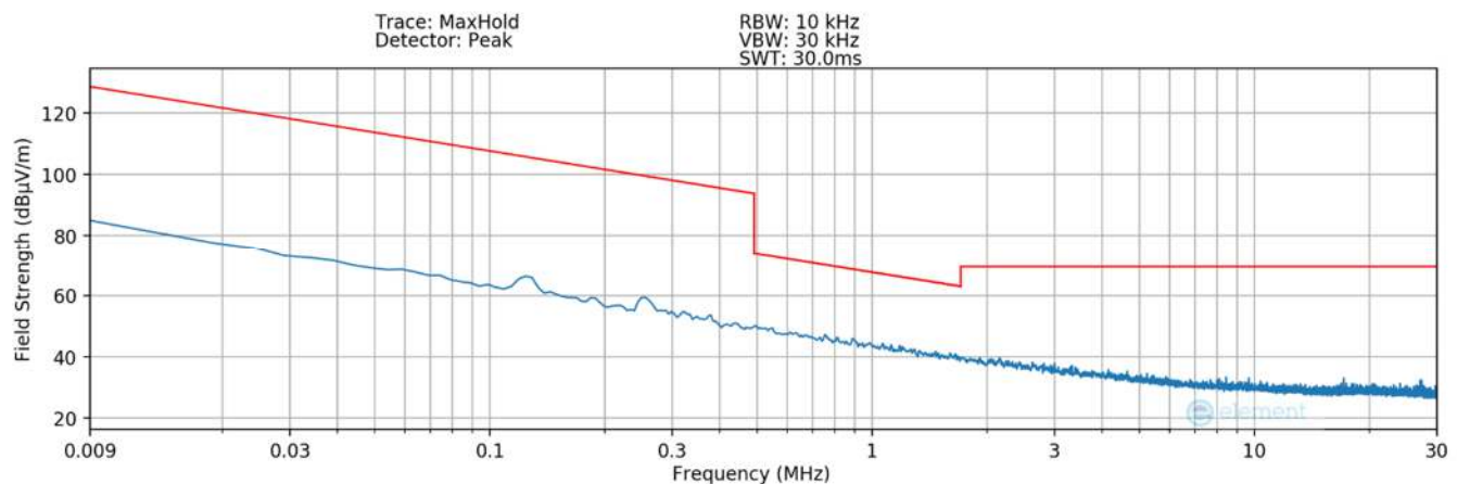
Plot 7-25. Radiated Spurious Plot 9kHz – 30MHz (Pol. Z – #4) – DCB LED
