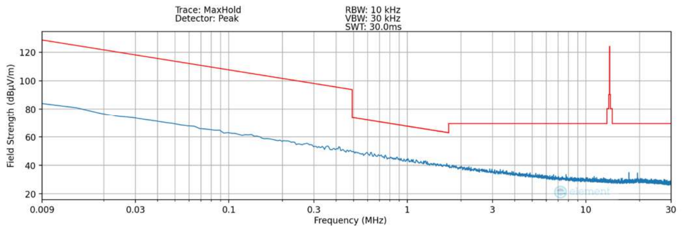
Plot 7-7. Radiated Spurious Plot 9kHz – 30MHz (Pol. Z – #1) – DCB LED
