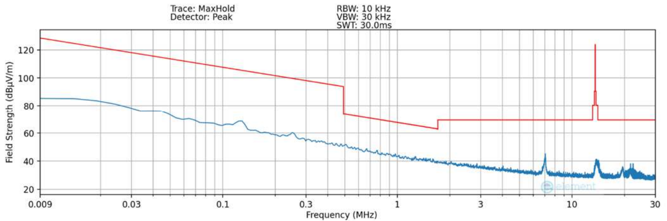
Plot 7-12. Radiated Spurious Plot 9kHz – 30MHz (Pol. Y – #2) – DCB LED
