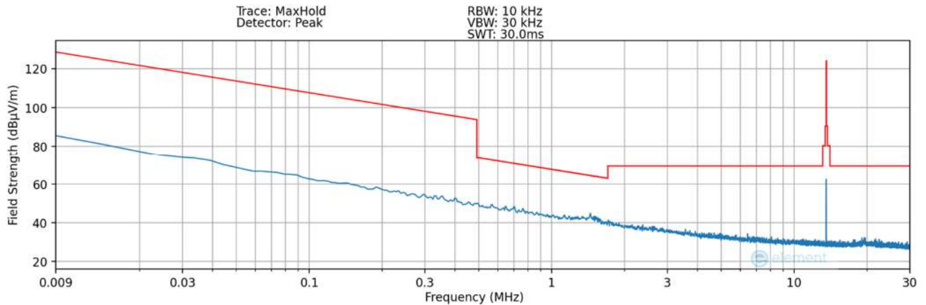
Plot 7-19. Radiated Spurious Plot 9kHz – 30MHz (Pol. Z – #3) – DCB LED
