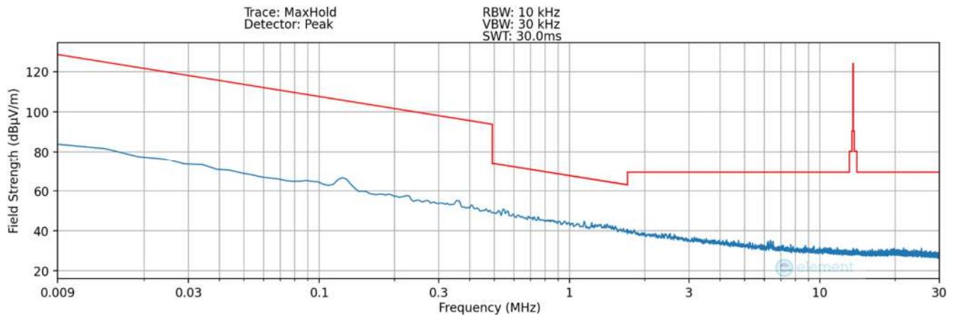
Plot 7-40. Radiated Spurious Plot 9kHz – 30MHz (Pol. Z – #6) – DCB
