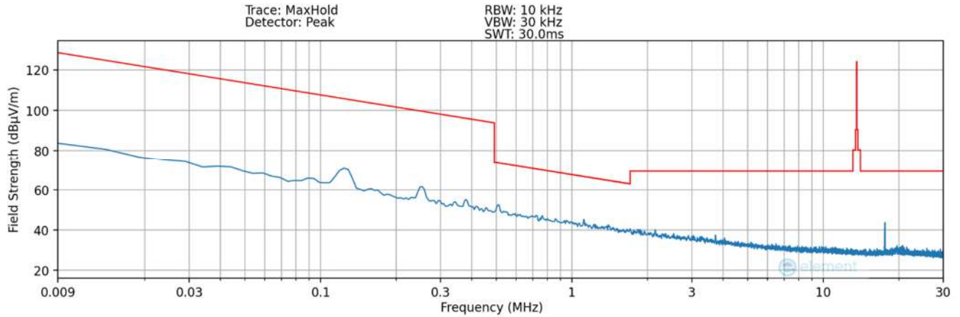
Plot 7-11. Radiated Spurious Plot 9kHz – 30MHz (Pol. X – #2) – DCB LED
