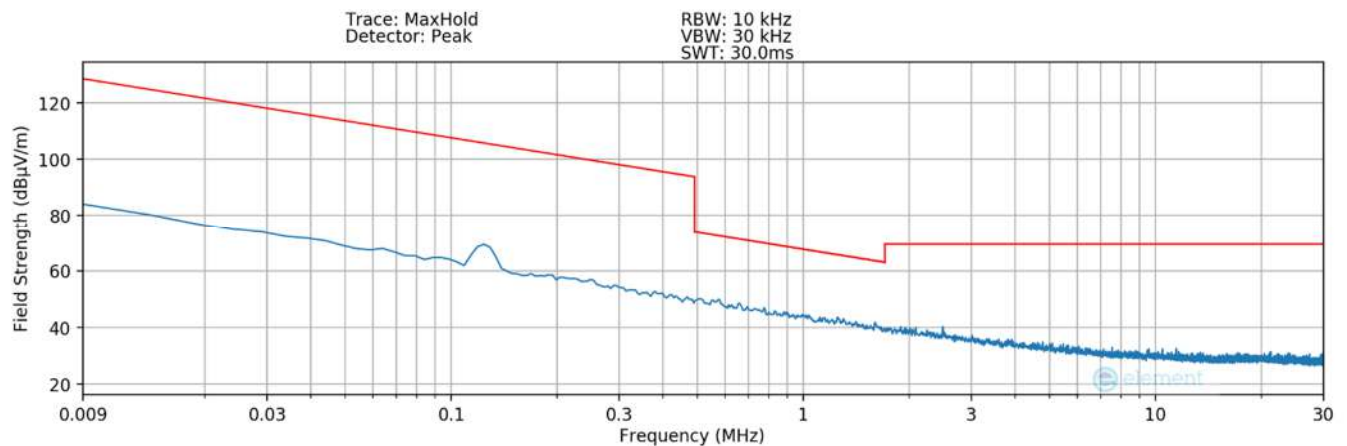
Plot 7-28. Radiated Spurious Plot 9kHz – 30MHz (Pol. Z - #4) – DCB
