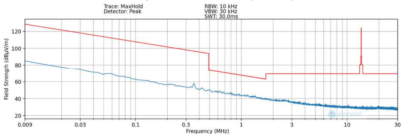
Plot 7-31. Radiated Spurious Plot 9kHz – 30MHz (Pol. Z - #5) – DCB LED
