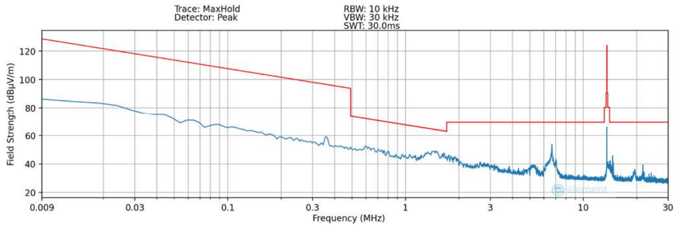
Plot 7-33. Radiated Spurious Plot 9kHz – 30MHz (Pol. Y – #5) – DCB
