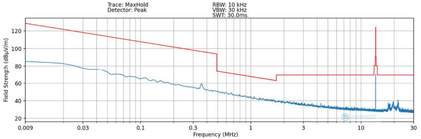
Plot 7-21. Radiated Spurious Plot 9kHz – 30MHz (Pol. Y – #3) – DCB
