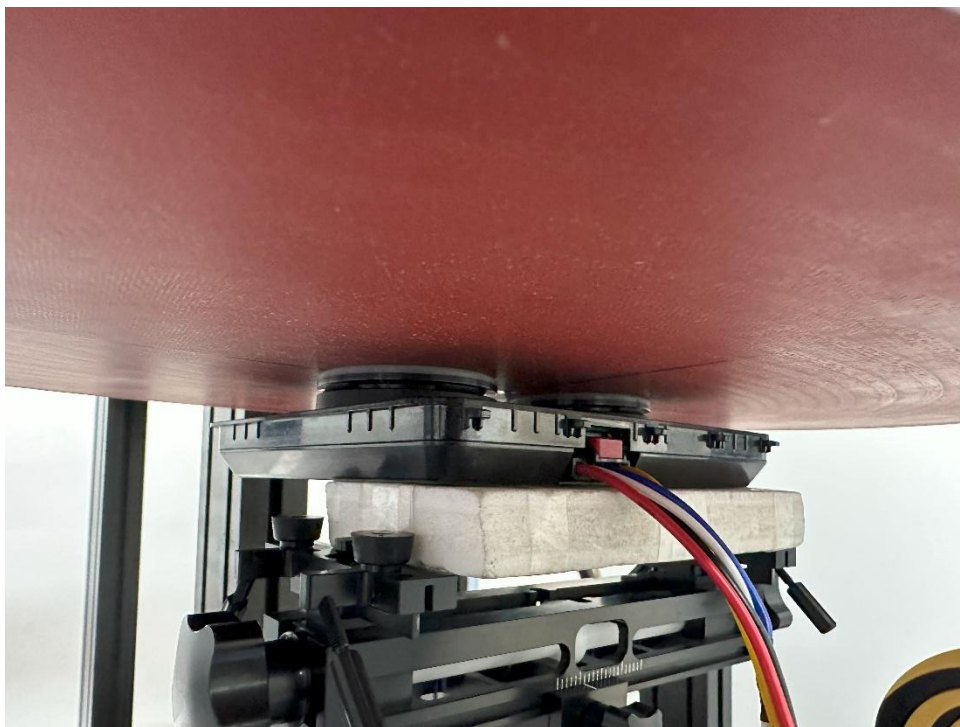
SAR Test Setup Photo 1 – NFC Body, Front Side at 0mm
