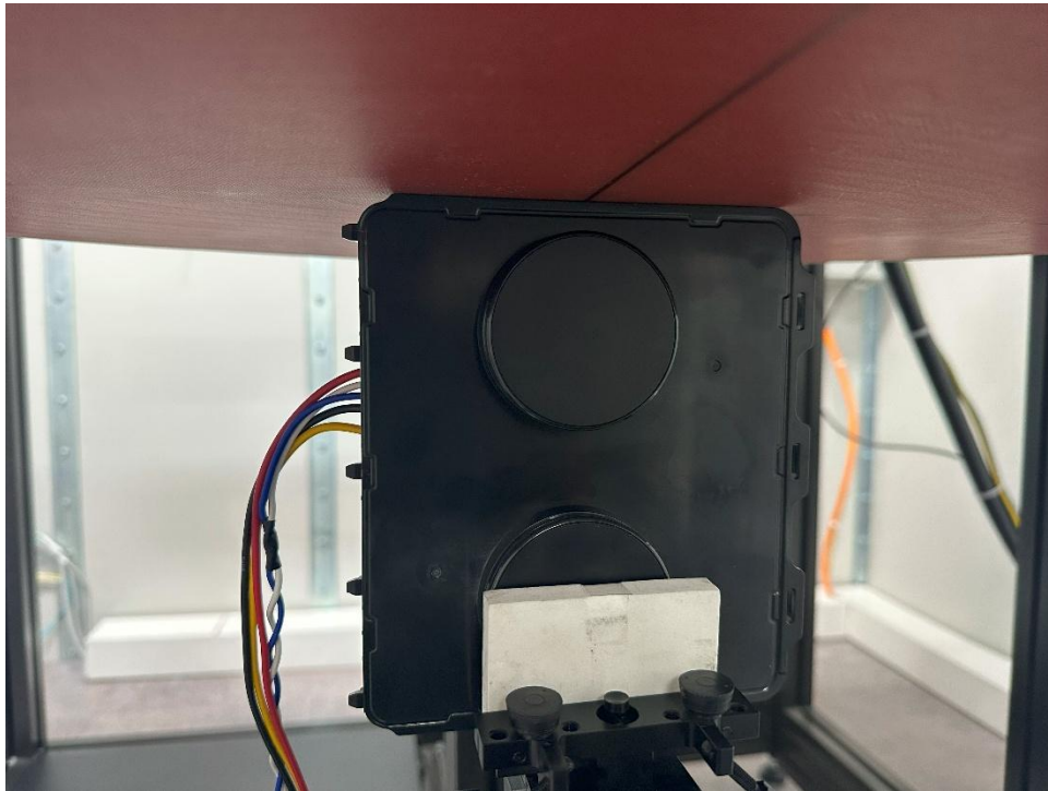
SAR Test Setup Photo 5 – NFC Body, Left Side at 0mm
