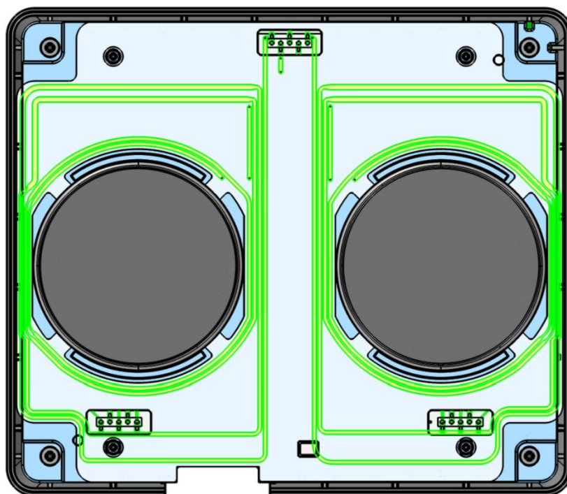
Figure F-1 NFC Antenna Locations
