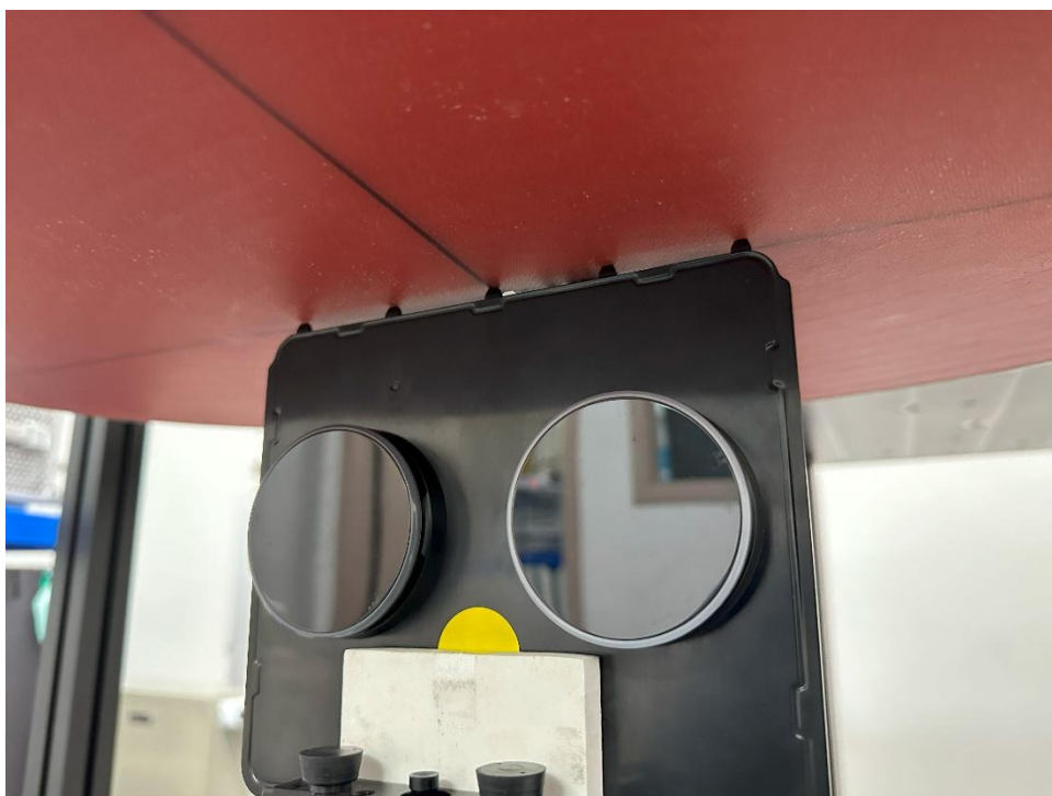
SAR Test Setup Photo 4 – NFC Body, Bottom Side at 0mm
