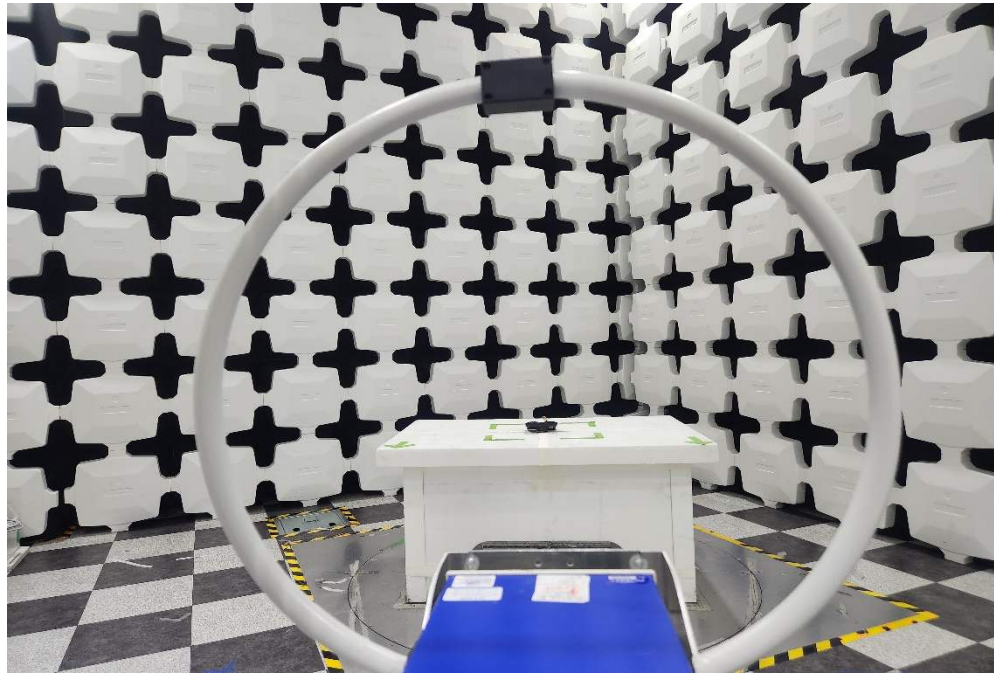
Figure 3. Test Setup – 9kHz-30MHz
