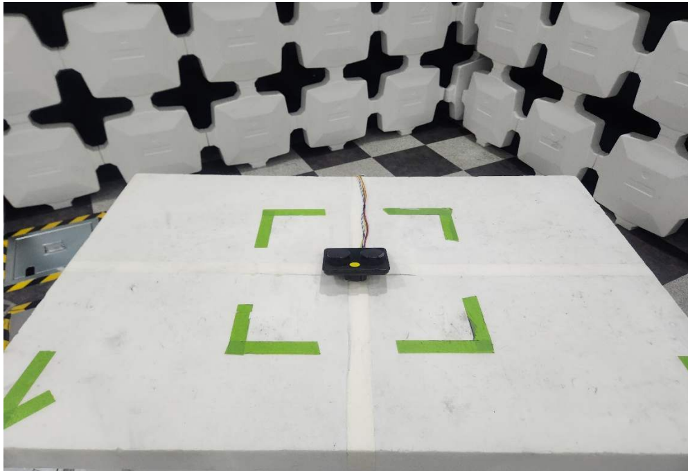
Figure 2. Test Setup – 9kHz-1GHz
