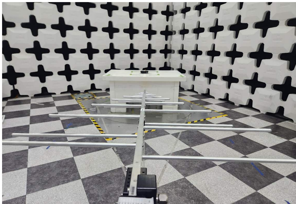
Figure 4. Test Setup – 30MHz-1GHz
