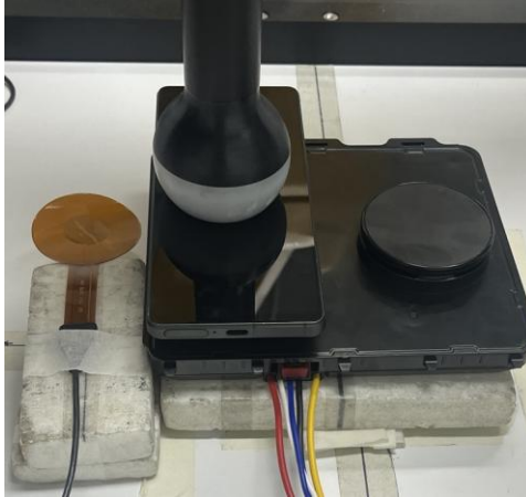
Test Setup Photo 7 EPP, Front side, 0mm
