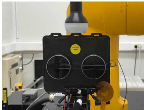
Test Setup Photo 3 Standby (Ping) Signal, Top Side, 0mm
