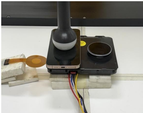
Test Setup Photo 9 MPP (RX2), Front side, 0mm
