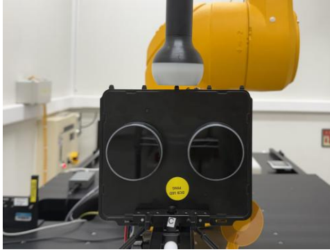
Test Setup Photo 4 Standby (Ping) Signal, Bottom Side, 0mm
