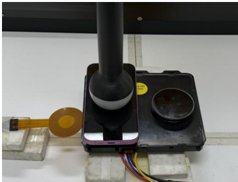
Test Setup Photo 8 MPP (RX1), Front side, 0mm
