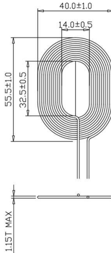
BOTTOM COIL : Smartbonding Litz WIRE 0.08*105P _ 12Ts
