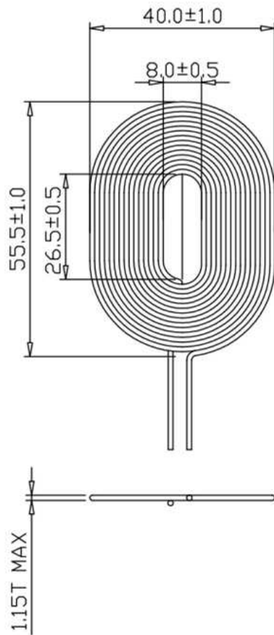
TOP COIL : Smartbonding Litz WIRE 0.08*105P _ 15Ts
