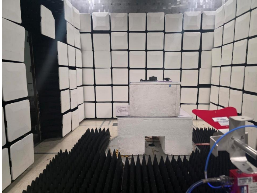
Figure 5 - Radiated emissions above 1 GHz (1 – 18 GHz), front view.
