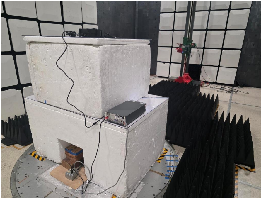
Figure 8 - Radiated emissions above 1 GHz (1 – 18 GHz), rear view (50kHz BW with GPS Simulator)
