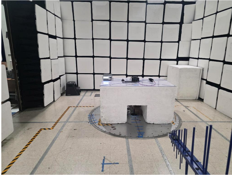
Figure 3 - Radiated emissions below 1 GHz (0.03 – 1 GHz), front view (50kHz BW with GPS Simulator)
