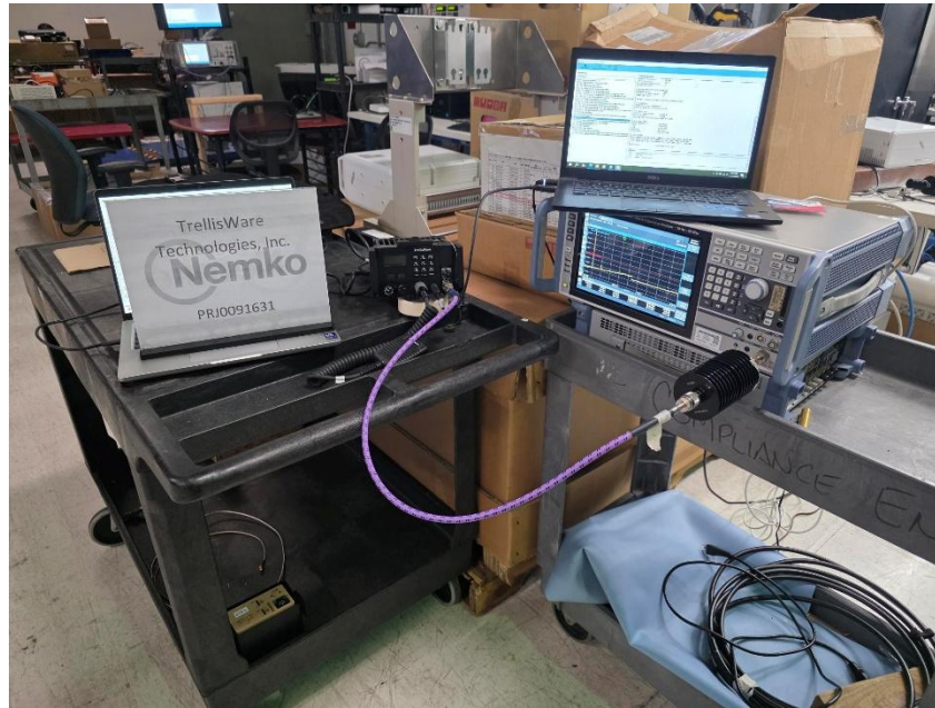
Figure 9 – Test setup (spectrum analyzer measurements)
