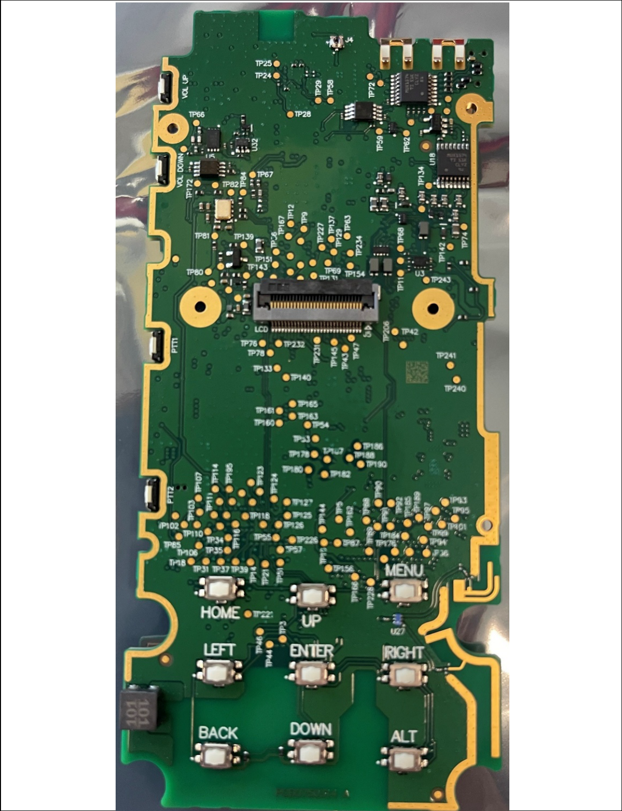
Figure 3. Module on PCB - Bottom
