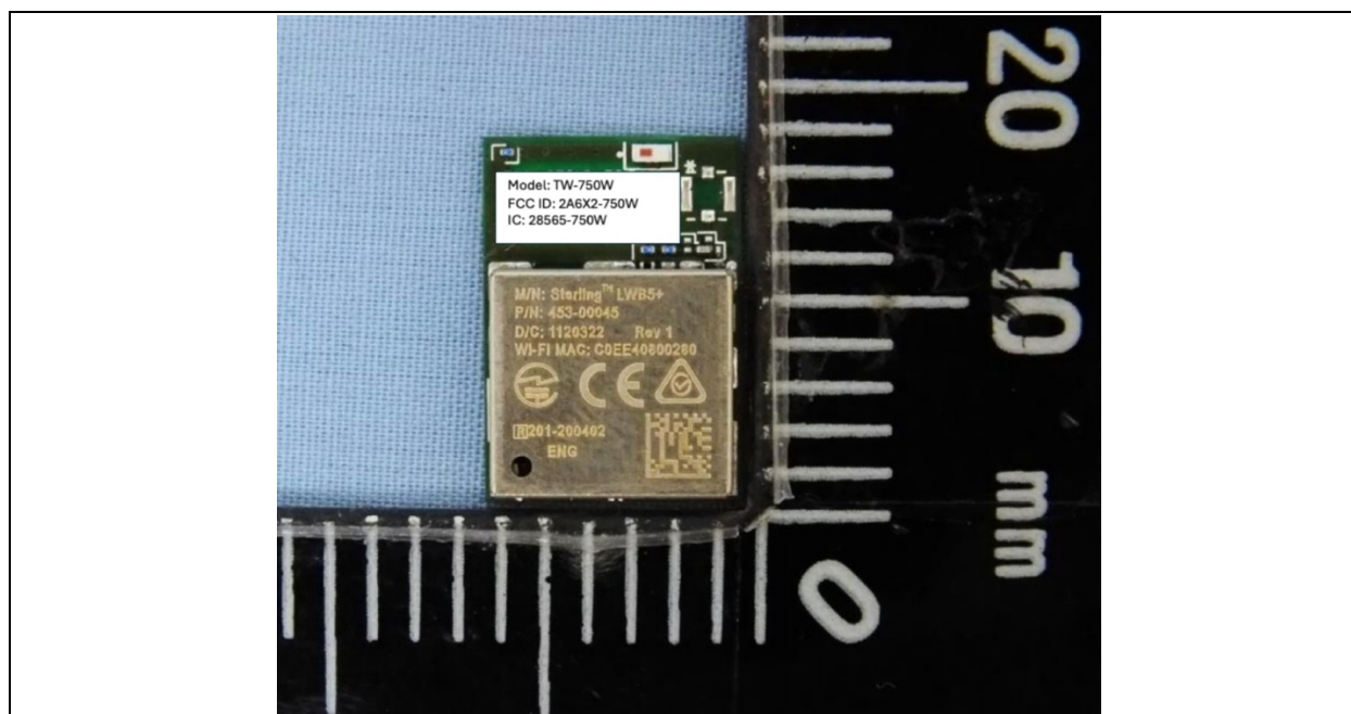
Figure 1. Front View
