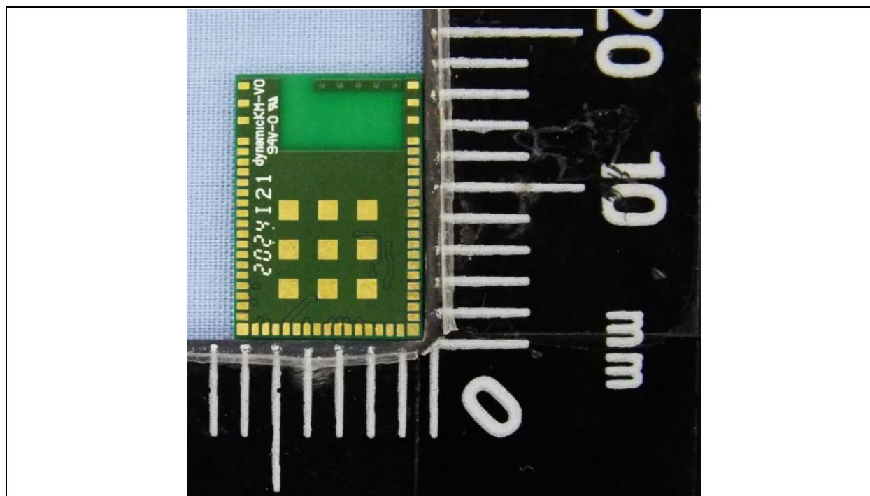
Figure 2. Rear View
