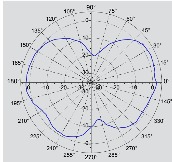
Gain
